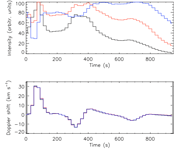
Fig. 6. Synthetic observations of a propagating wave by Hinode/EIS in the spectroscopy mode corresponding to Fig. 2. Three different iron lines with a 1'' slot are used. The black, red and blue lines correspond to Fe XII, Fe XI and Fe X, respectively.
