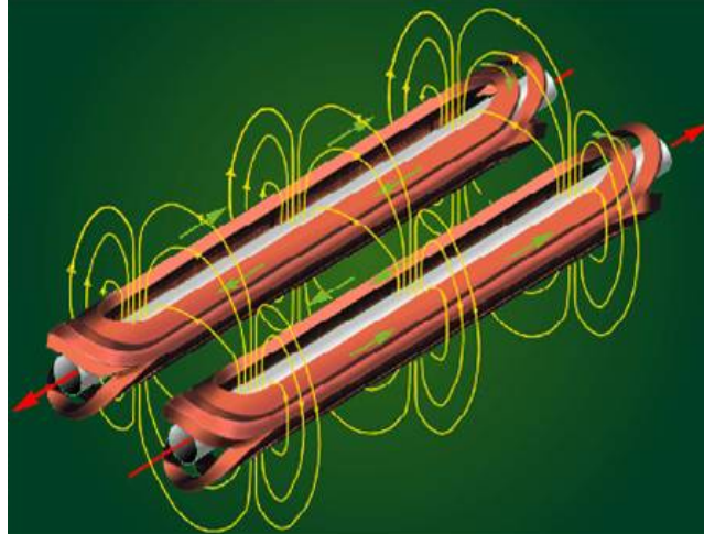
Figure 2.3: The magnetic field lines in a LHC main dipole.
