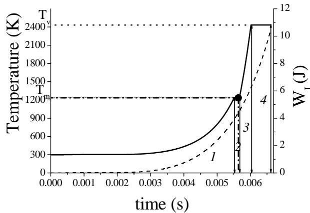
Figure 14: Simulation of the temperature evolution (continuous line) with the experimental value of t_p (solid circle) and W_J (dashed line) in the fuse during the pre-arcing time.
