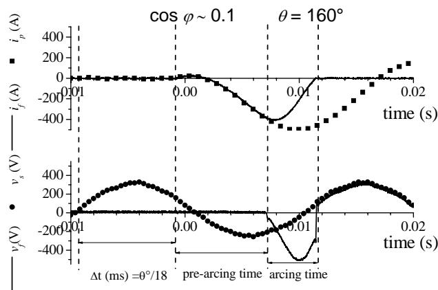
Figure 1 : Characteristic curves of fuse breaking under AC supply: fuse voltage v_f , supply voltage v_s , fuse current i_f , prospective current i_p .
