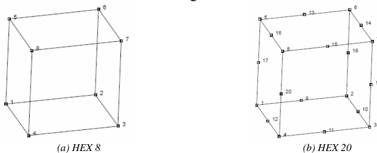
Figure B.16 : Eléments finis solides
