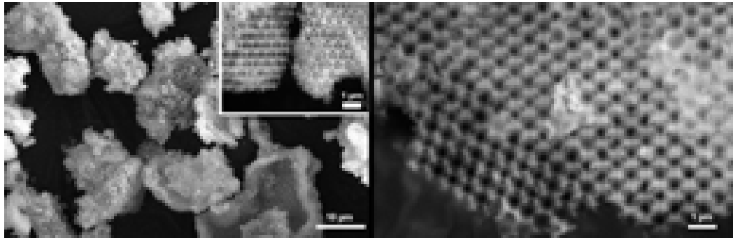
Figure IV.7 – Micrographies MEB de la phase Zn 2 Cr
