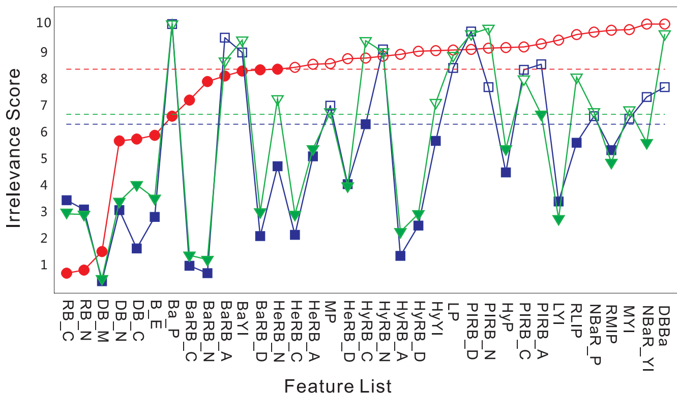
Figure 2 Verification of the features that potentially influence peptide fragmentation. The importance of the features listed in Table 1 is evaluated by the Bayesian neural network and the results are shown: Red circles: normalized irrelevance scores of the features under non-mobile status. Blue squares: normalized irrelevance scores of the features under partial-mobile status. Green triangles: normalized irrelevance scores of the features under mobile status. The higher an irrelevance score is, the less important the corresponding feature is. The threshold of each mobility status is shown in dashed line and the features proven to be influential on peptides' fragmentation (below threshold) are highlighted with filled circles/squares/triangles.
