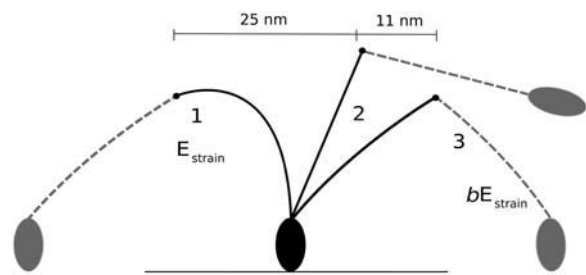
FIGURE 3 The mechanical movement of myosin-V takes place in two separate steps. The first step, through a distance d_W \approx 25 nm, is from the highly strained state 1 to state 2 where the internal strain balances the external force. When the molecule diffuses to state 3, through a further distance d_D \approx 11 nm, the internal strain increases to bE_{\text{strain}} .
