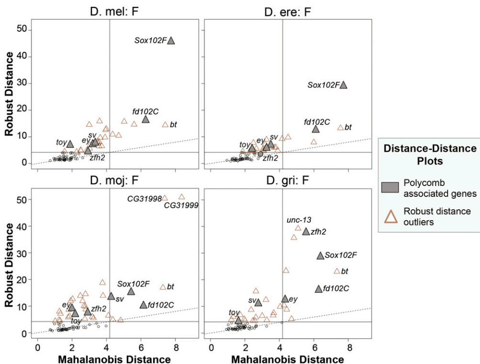
Figure 7 Distance–Distance Plots of robust distance (RD) vs. Mahalanobis distance (MD) show both common and species-specific outliers. The horizontal and vertical lines correspond to the cutoff values for outliers (97.5% quantile of the \chi^2 distribution, see File S1). Values greater than the cutoff values identify outliers. Triangles in the upper right quadrant are outliers based on both RD and MD. Triangles in the upper left quadrant are outliers only based on RD. The dashed line corresponds to points with equal RD and MD values. F element genes that reside in a Polycomb domain in D. melanogaster are highlighted in gray.
