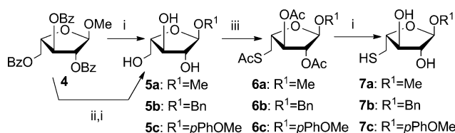
Scheme 1 Chemical synthesis of 5-deoxy-5-thio- \alpha -L-arabinofuranosides: i) MeONa (0.01 M), MeOH, rt: 5a (100%), 7a (100%), 7b (94%), 7c (98%); ii) a) Ac 2 O, cat. H 2 SO 4 , CH 2 Cl 2 , rt, b) BF 3 ·OEt 2 (3.1 eq.), Et 3 N (0.08 eq.), alcohol (1.2 eq.), CH 2 Cl 2 , rt, 24 h: 5b (71%), 5c (63%); iii) a) thioacetic acid (1.8 eq.), PPh 3 (1.7 eq.), DIAD (1.7 eq.), THF, rt, overnight, b) Ac 2 O/pyridine (1/1), rt, 3 h: 6a (69%), 6b (74%), 6c (74%).
