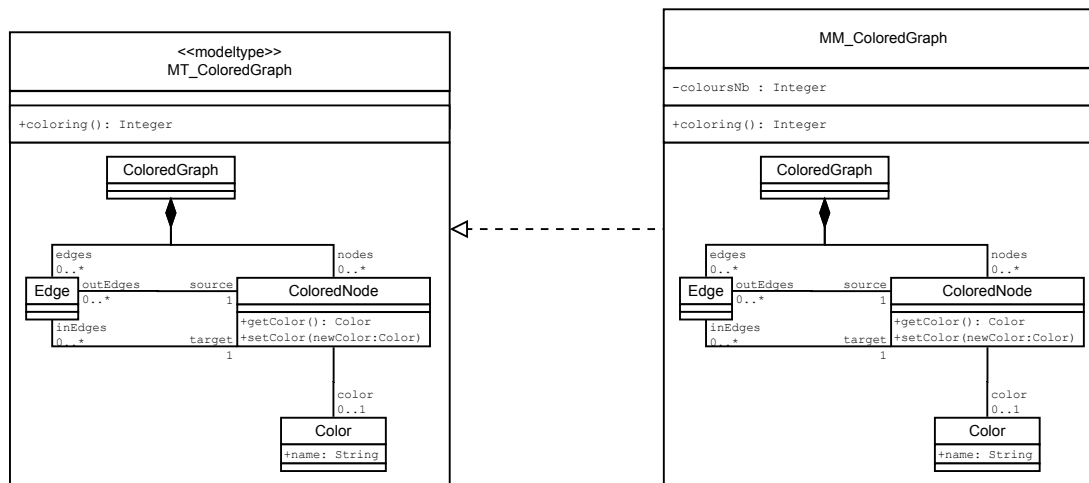
FIGURE 6.8 – Type de mod eles MT_{ColoredGraph} (  gauche) et m etamod ele MM_{ColoredGraph} impl ementant MT_{ColoredGraph} (  droite).
