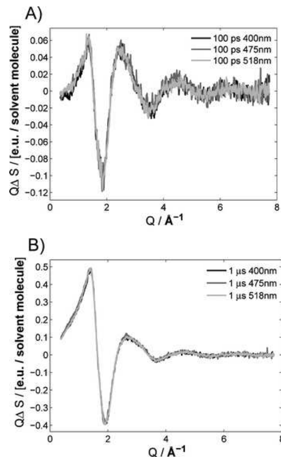
Fig. 7 100 ps (A) and 1 \mu\text{s} (B) difference scattering curves scaled to the 400 nm signal obtained for dye mediated solvent heating using 1 mM 4-bromo-4'-( N,N -diethylamino)-azobenzene ( 2 ) in acetonitrile and exciting at 400 nm, 475 nm and 518 nm. The recorded difference scattering curves are identical within the noise. All data have been recorded with 200 \mu\text{J} ( 0.15 \text{ J cm}^{-2} ) per pulse.
