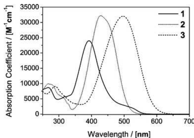
Fig. 3 Absorption spectra of sodium 4-aminoazobenzene-3,4'-disulphonate ( 1 ), 4-bromo-4'-( N,N -diethylamino)-azobenzene ( 2 ) and 4-( N,N -diethylamino)-2-methoxy-4'-nitro-azobenzene ( 3 ) in methanol.
