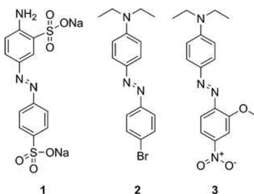
Fig. 2 Molecular structure of sodium 4-aminoazobenzene-3,4'-disulphonate (1), 4-bromo-4'-( N,N -diethylamino)-azobenzene (2) and 4-( N,N -diethylamino)-2-methoxy-4'-nitro-azobenzene (3).
