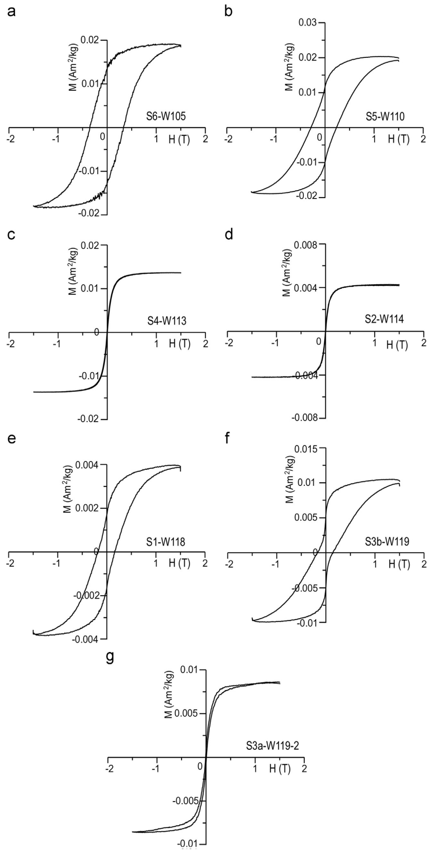
Fig. 12. Hysteresis loops of samples of the wells studied after subtraction of the paramagnetic susceptibility. H (T): induced field, M ( \text{A m}^2/\text{kg} ): induced magnetization. Same notations as in Fig. 10.
