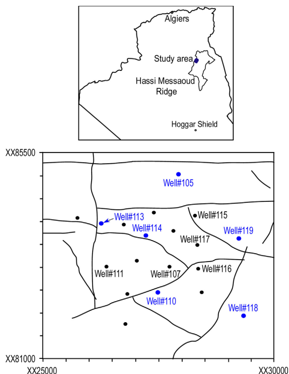
Fig. 1. Location of the study area (according to Askri et al. (1995) and Aouimer and Cherriff (2008)). Lines: faults, circles: exploration wells.
