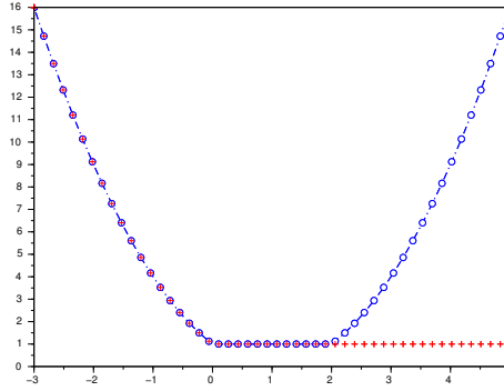
FIGURE 1. The graphs of the Hamiltonian p \mapsto H_i(O, p) (with the circles) and of p \mapsto H_i^+(O, p) \equiv \max_{a \in A_i: f_i(O, a) \geq 0} (-p f_i(O, a) - \ell_i(O, a)) (with the signs +). In the example, \mathcal{P}_0^i = [0, 2] .
