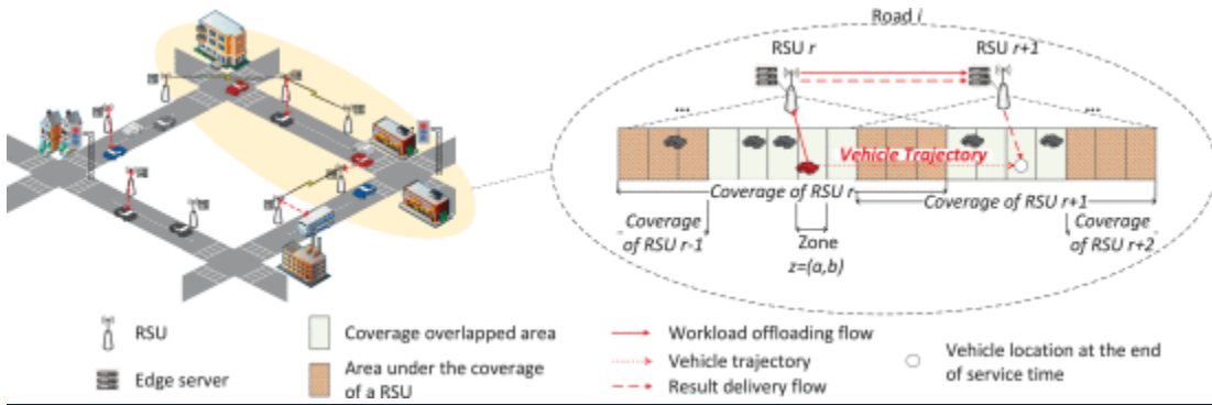
Fig. 1. Network model.
