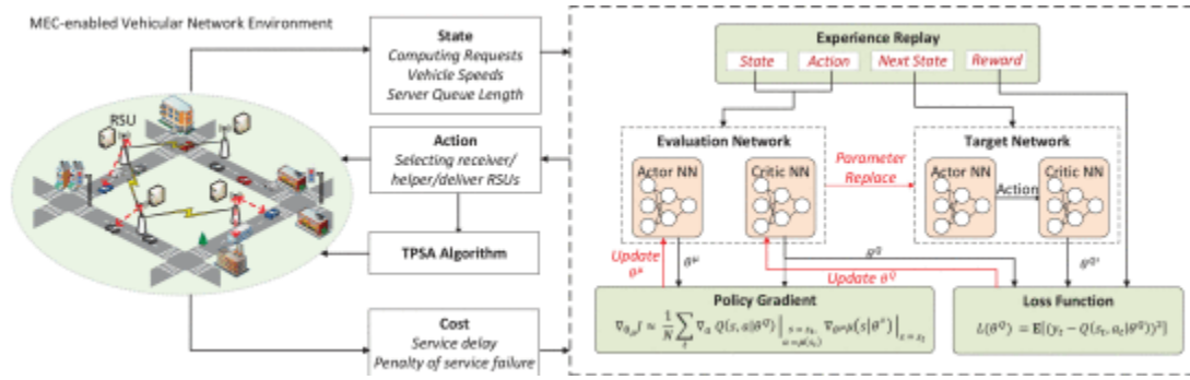
Fig. 3. AI-based collaborative computing approach.
