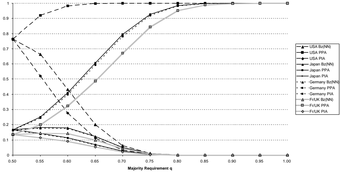
Figure 2: Effect of the Majority Requirement q on Coleman's and Banzhaf's Indices, Top Five Members of the IMF
