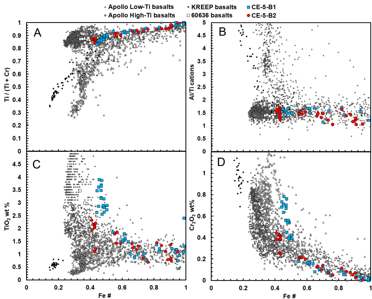
Fig. S12. Pyroxene minor element composition mineral chemistry in basalt fragments CE-5-B1 (blue symbols) and CE-5-B2 (red symbols). Fe\# ( Fe/(Fe+Mg) ) vs. (a) Ti\# ( Ti/(Ti+Cr) ), (b) Al/Ti (cation ratio), (c) TiO_2 wt% and (d) Cr_2O_3 wt%. Data are compared with Apollo low-Ti mare basalts from the Apollo 12 and 15 landing sites; high-Ti mare basalts from the Apollo 11 and 17 landing sites (41); KREEP basalts (41, 40) and intermediate-Ti basalt fragments in sample 60639 (42).
