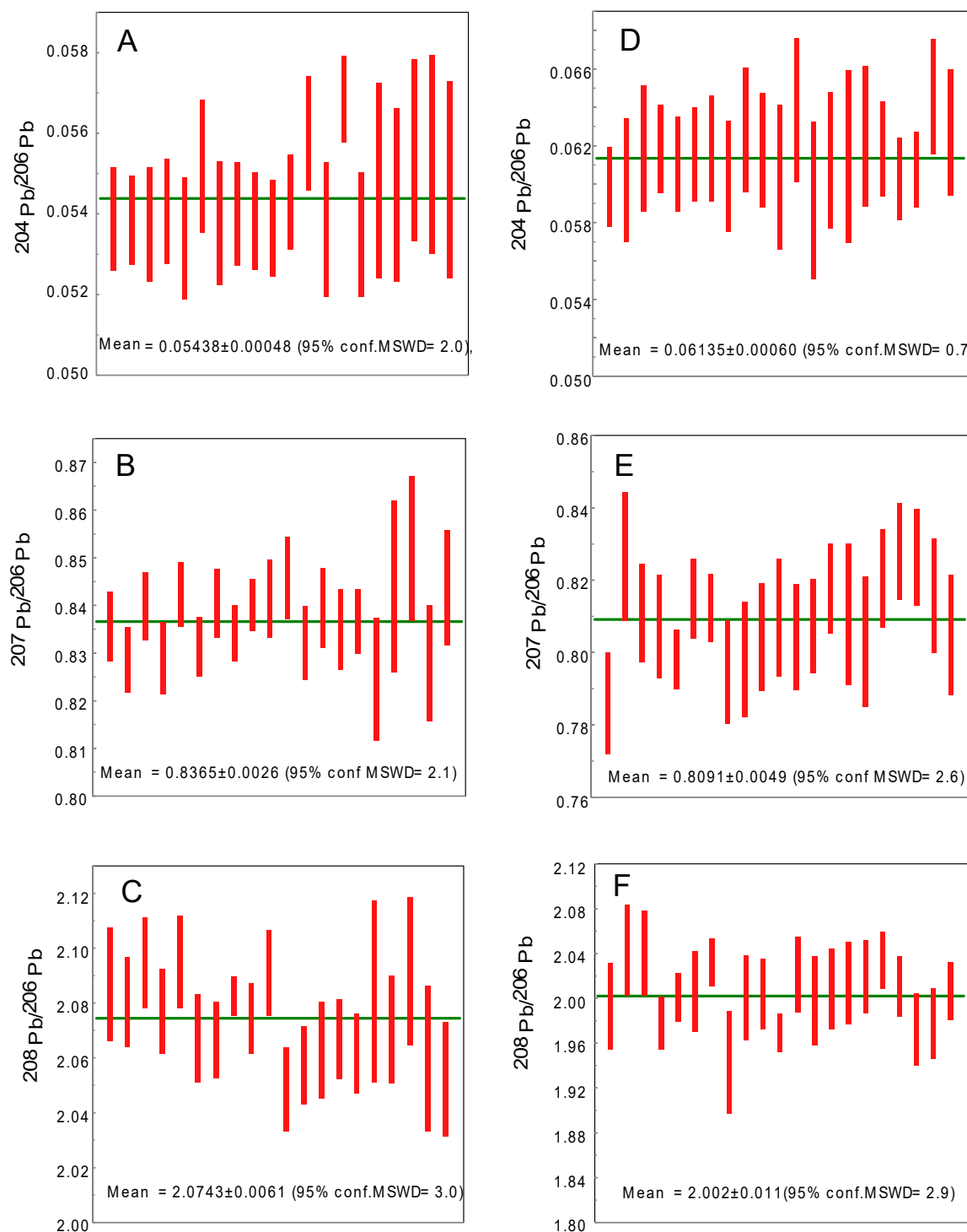
Fig. S3. Lead isotope analyses of BCR-2G obtained during the analytical session.
