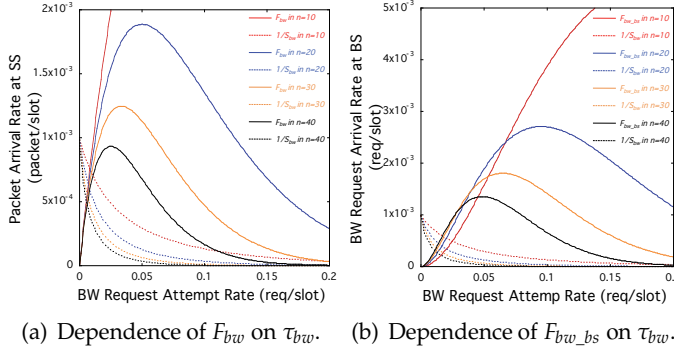
Fig. 8. Dependence of each element on \tau_{bw} .
