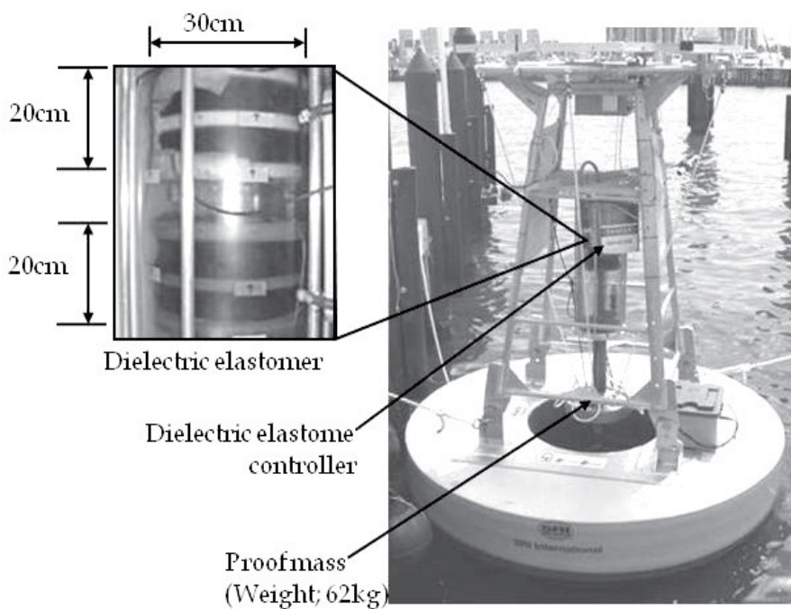
Photo 6. Dielectric elastomer generator on the test buoy
