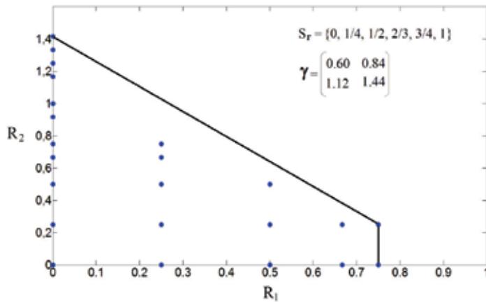
Fig. 10. Example of OFDMA rate region with discrete codebook S_r .
