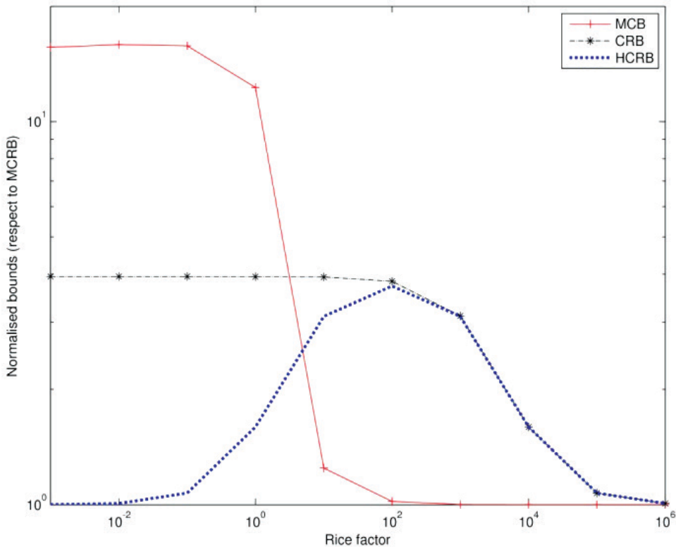
Fig. 4. Normalized bounds versus the Rice factor
