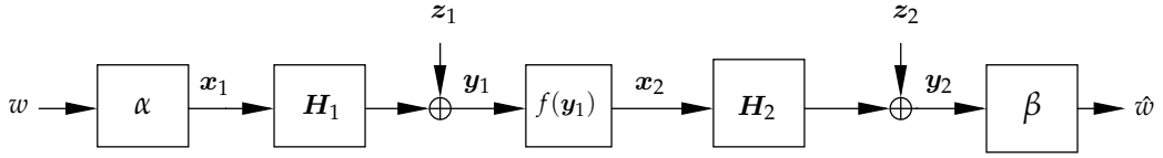
Fig. 1. Gaussian two-hop MIMO relaying.
