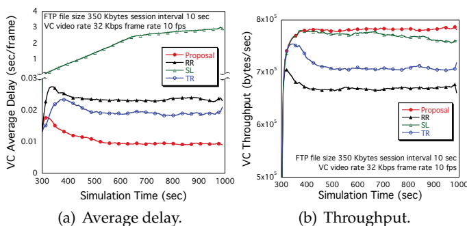
Fig. 17. Transition of VC on FTP file size 350K bytes.
