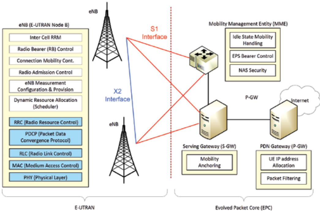
Fig. 1. LTE Architecture and functional split between E-UTRAN and EPC
