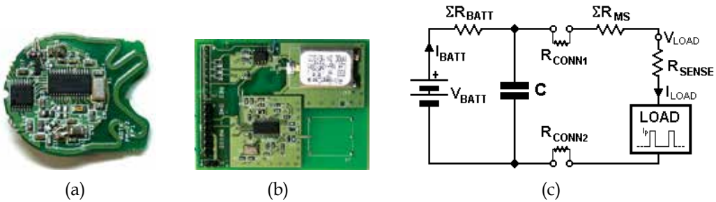
Fig. 11. Pictures of wireless control systems with capacitor place at the battery terminals, (a) high-value aluminium organic and (b) super-capacitor. (c) Schematic diagram of power supply system with high-value capacitor at the battery ends
