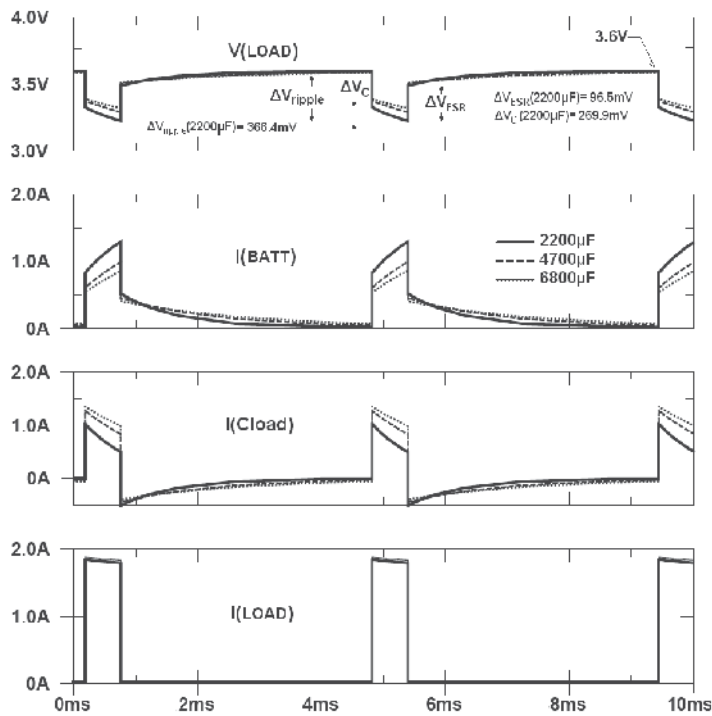
Fig. 15. (a) Voltage ripple in the load, V(\text{LOAD}) , (b) battery, (c) capacitor and (d) load current with capacitors of 2200, 4700 and 6800 \mu\text{F}
