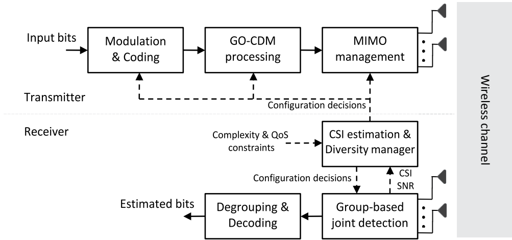
Fig. 4. Communication architecture for a MIMO-GO-CDM with group-size adaptation.
