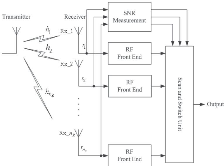
Fig. 2. Block diagram of switch combining scheme
