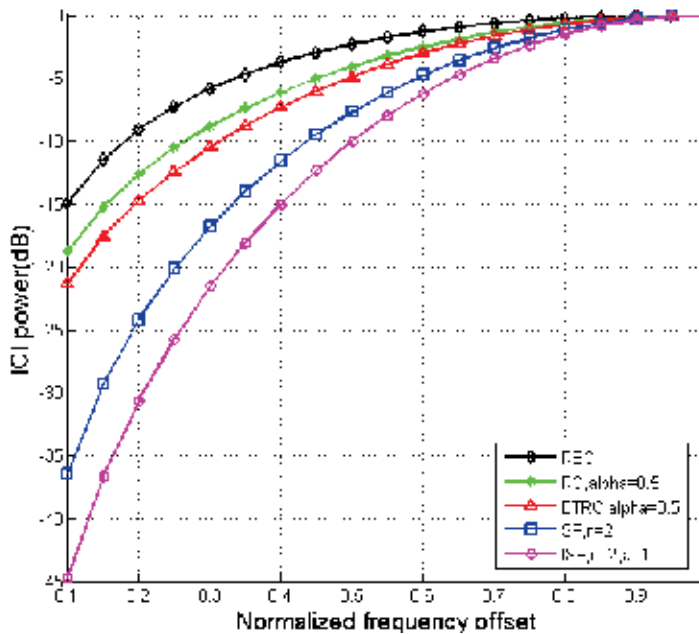
Fig. 7. ICI comparison for different pulse shapes
