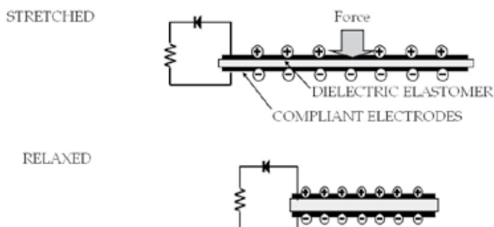
Fig. 7. Operating principle of dielectric elastomer power generation
