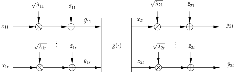
Fig. 3. Equivalent parallel channel.
