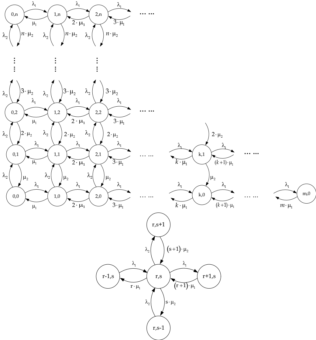
Fig. 3. The two-dimensional Markov model's state transition diagram
