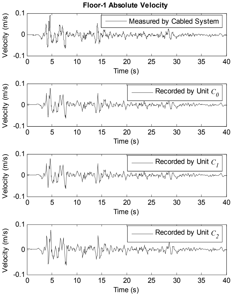
(a) Floor-1 absolute velocity data recorded by the cabled and wireless sensing systems
