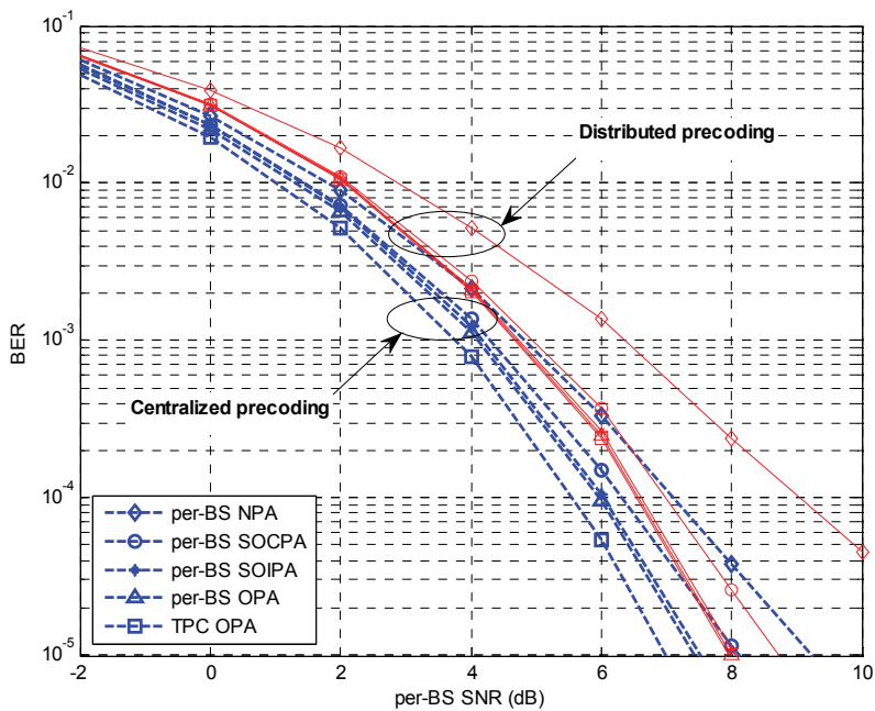
Fig. 7. Performance evaluation of the proposed distributed and centralized multi-cell schemes for scenario 3
