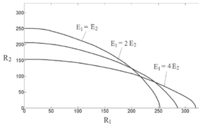
Fig. 17. Outage rate regions when the users' channels have different average energy ( E_m ).
