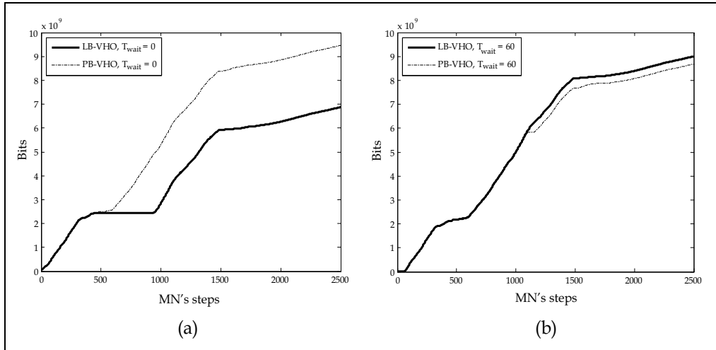
Fig. 6. CRB during a simulated scenario with PB and LB-VHO approaches, for (a) T_{wait} = 0 s, (b) T_{wait} = 60 s
