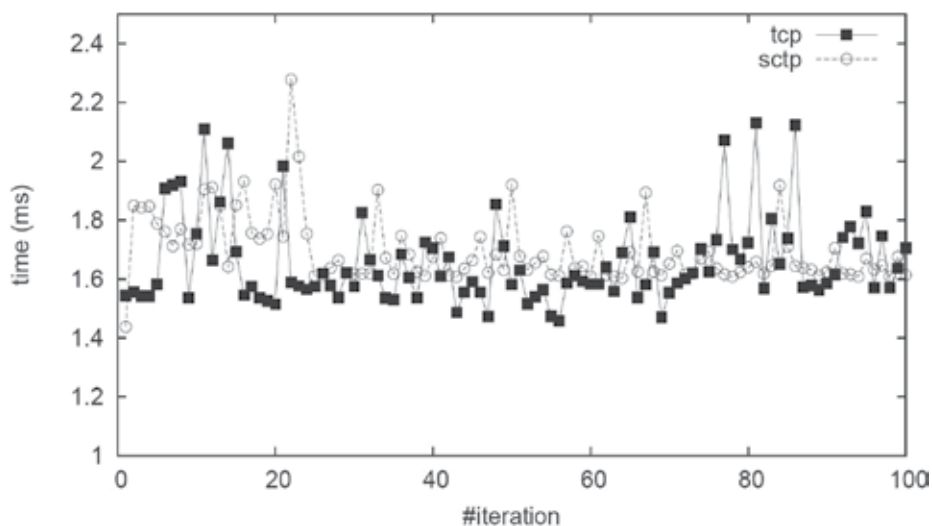
Fig. 7. Socket initiation time in TCP and SCTP in two-file downloading
