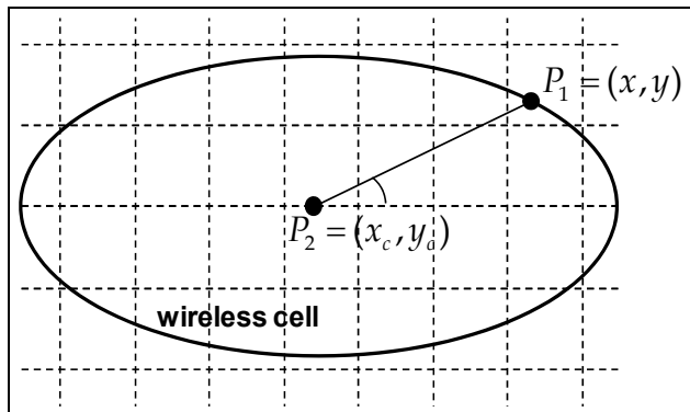
Fig. 9. Trigonometric approach for path loss map building in a (circular) wireless cell environment
