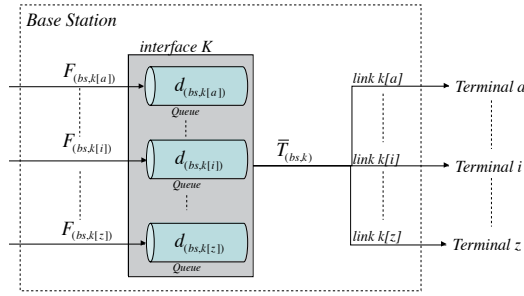
(a) Downlink cost associated by 11-interface.
