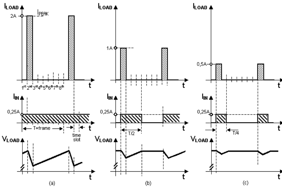
Fig. 21. PA GSM cellular terminal voltage and current waveforms for three power levels, (a) maximum and (b) (c) intermediate
