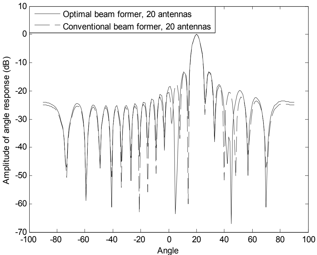
Fig. 18. Angle responses of optimal and conventional beamforming schemes
