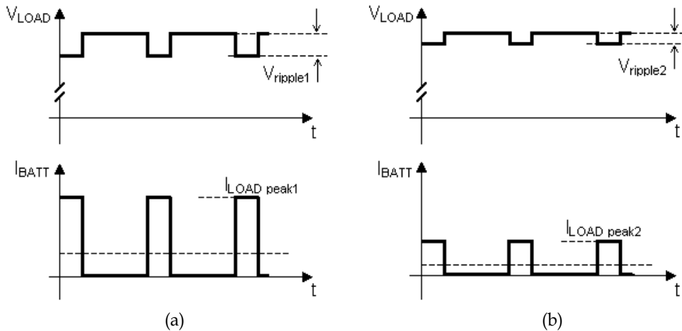
Fig. 6. Load voltage and battery current waveforms of a wireless system with discontinuous consumption for (a) maximum consumption and (b) mean consumption
