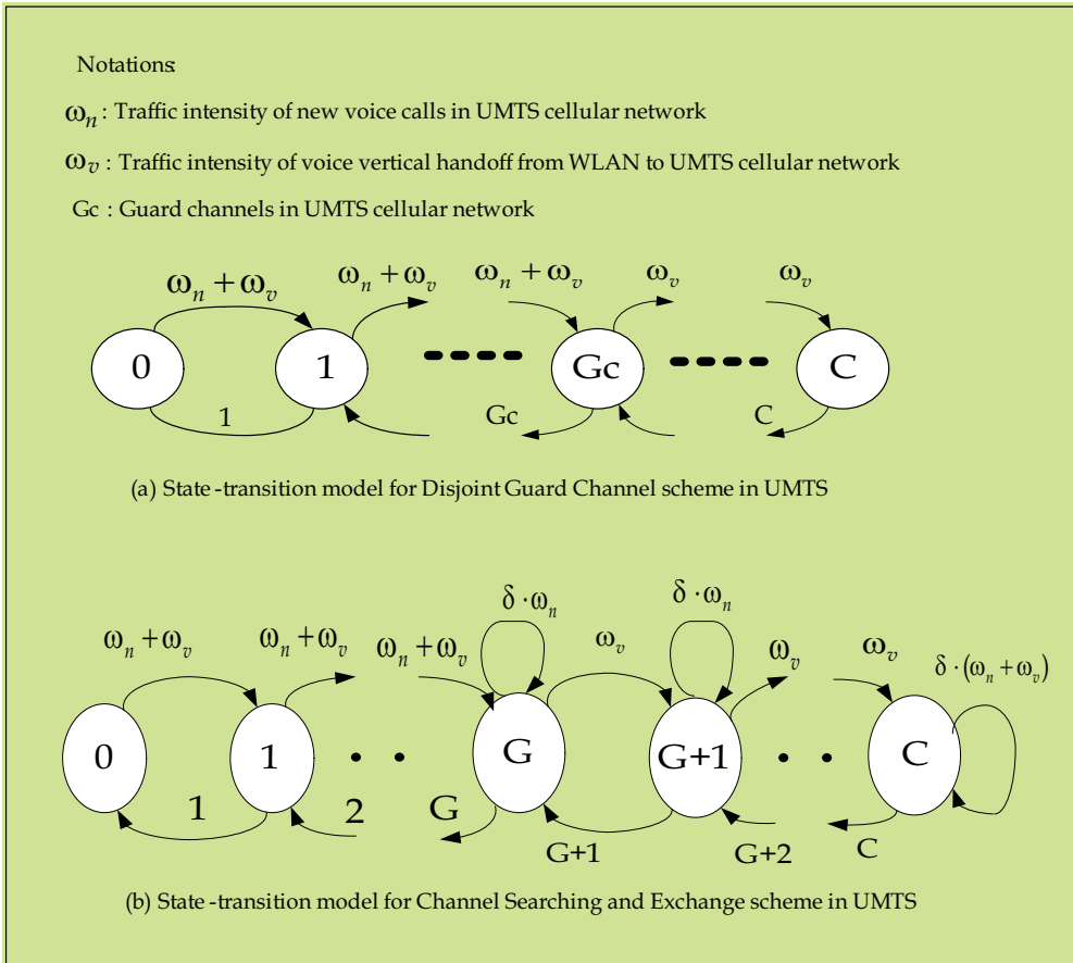
Fig. 9. State-transition diagram for DGC and CSR algorithms
