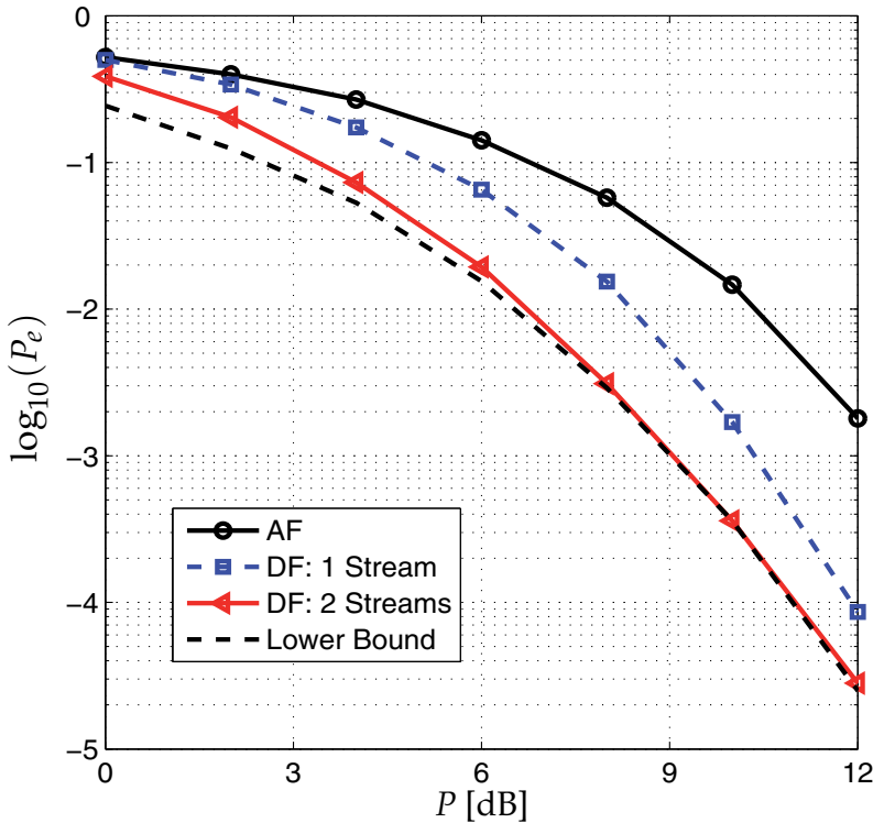
Fig. 5. Average message error probability ( P_e ) using 16-QAM modulation for different forwarding strategies (AF, conventional DF (i.e., one stream) and proposed DF (i.e., two streams with permuted modulations)). Here we set P_1 = P_2 = P , N_1 = N_2 = 1 , number of antennas at the source is N = 1 and number of antennas at the relay and the destination are L = M = 10 .
