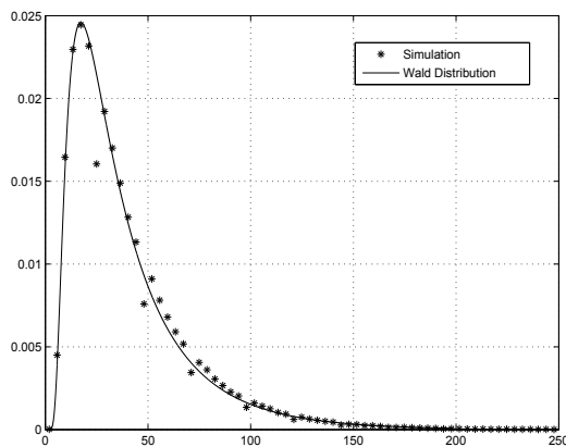
Fig. 9. Approximation of decision time using Wald Distribution.
