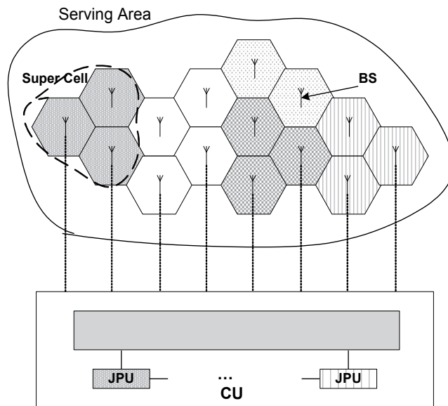
Fig. 1. Enhanced cellular architecture
