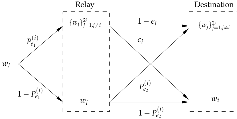
Fig. 4. Error probability transition in DF relaying.
