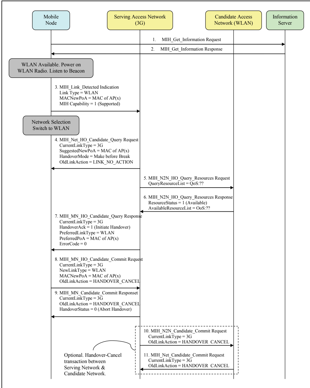
Fig. 2. MN-initiated and MN-cancelled handover
