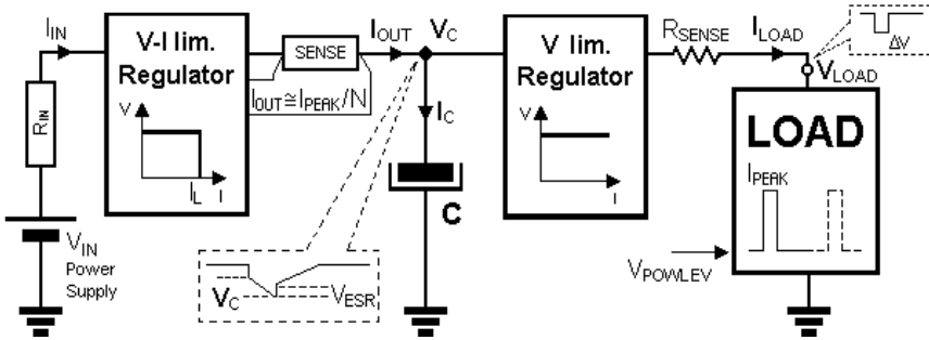
Fig. 22. Block diagram of constant current and constant input current power supply
