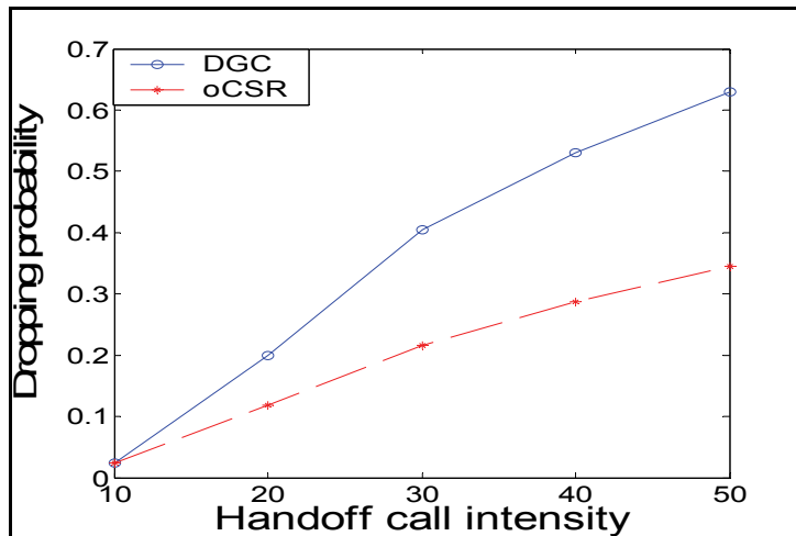
Fig. 15. Dropping probability with optimal CSR and DGC
