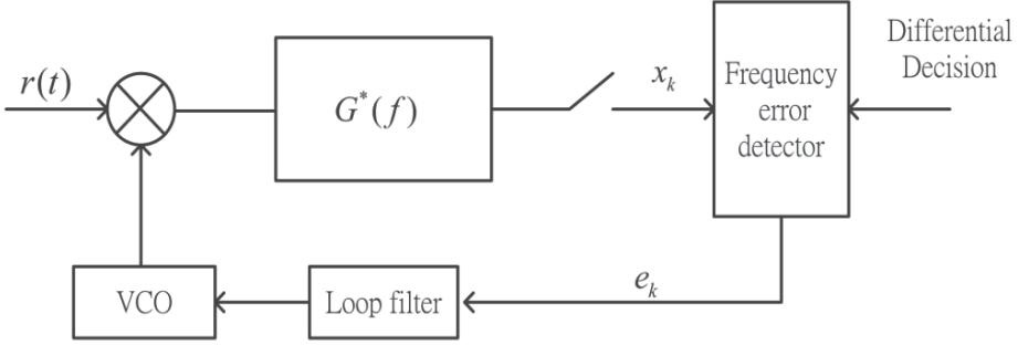
Fig. 6. Differential decision-directed (DDD) algorithm
