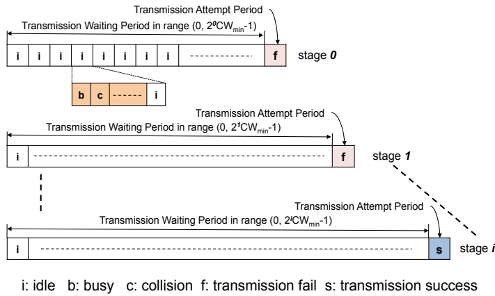
Fig. 2. Exponential binary backoff in IEEE802.11.
