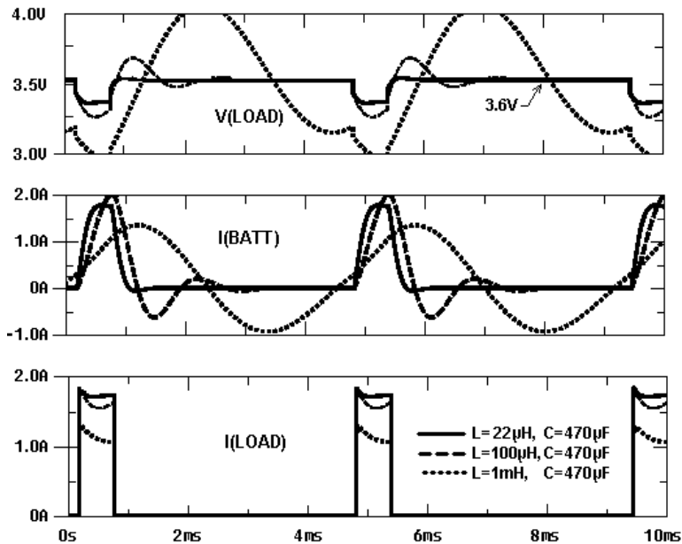
Fig. 19. Load voltage ripple, battery and load current for a capacitor of 470\ \mu\text{F} and de 22\ \mu , 100\ \mu and 1\text{mH} inductors
