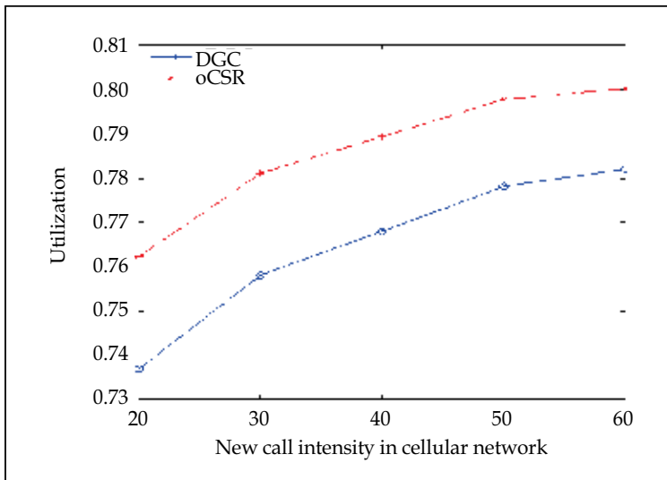
Fig. 13. Utilization with new call intensity in UMTS
