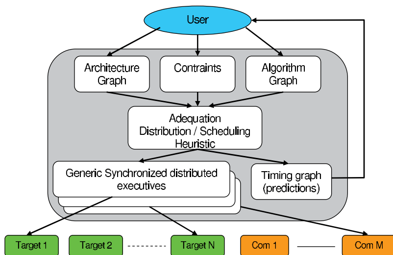
Fig. 5. SynDEX utilization global view
