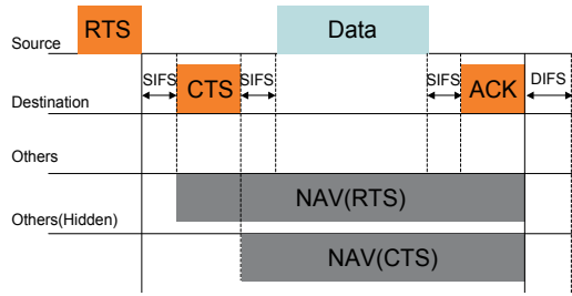
Fig. 3. RTS/CTS access control sequence in IEEE802.11.
