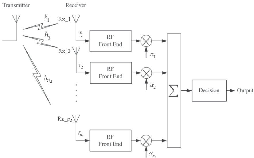
Fig. 3. Block diagram of MRC scheme
