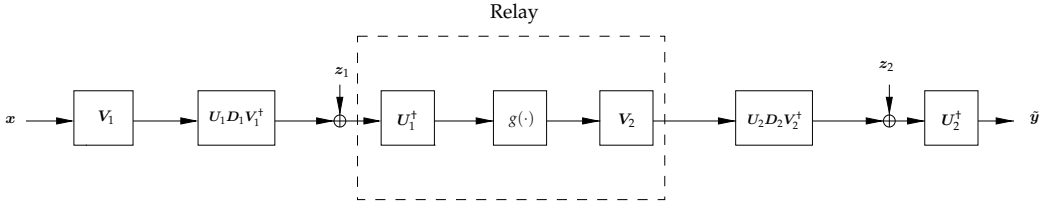
Fig. 2. Processing using the SVD of the channel matrices.
