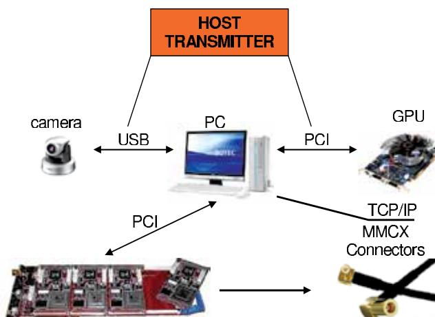
Fig. 3. Hardware Architecture
