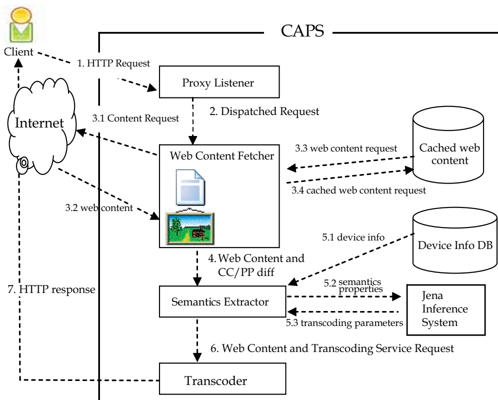
Fig. 1. System architecture of content adaptation proxy server
