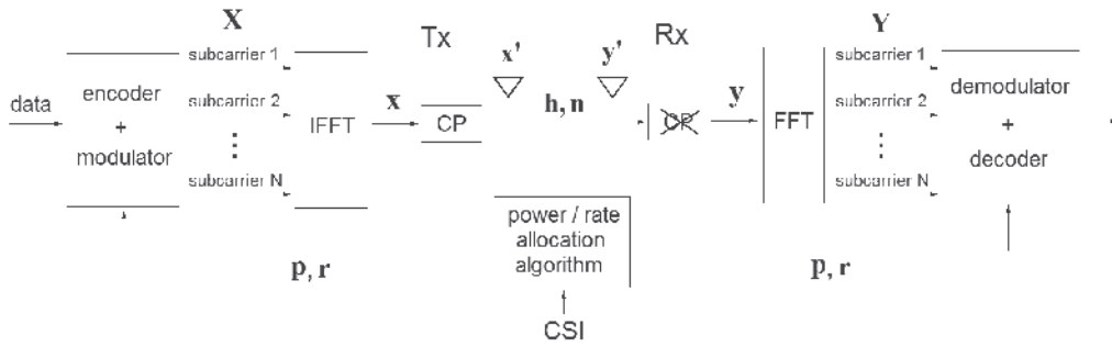
Fig. 1. Single-user OFDM system with power and rate adaptation.
