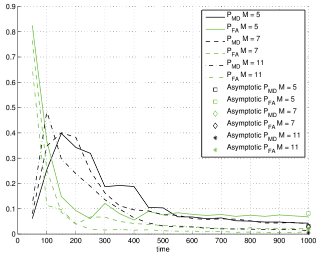
Fig. 12. Data fusion scheme considering sequential analysis decision from each sensor ( P_{M,I} = 0.3, P_{F,I} = 0.1 ).
