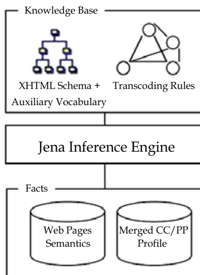
Fig. 3. Architecture of the Jena inference system
