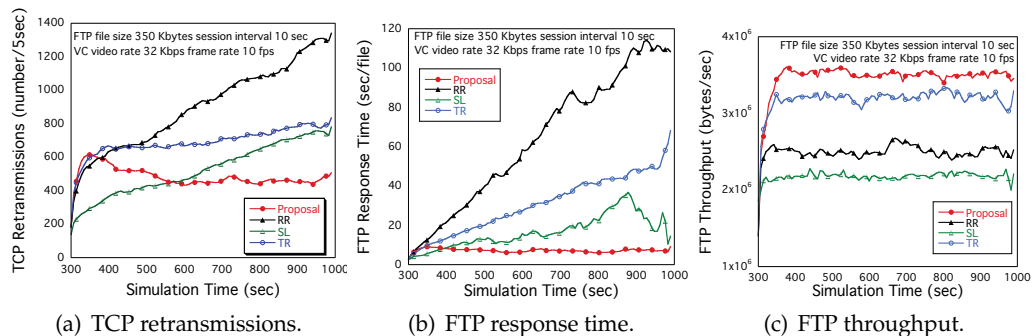
Fig. 16. Transition of TCP and FTP on FTP file size 350K bytes.
