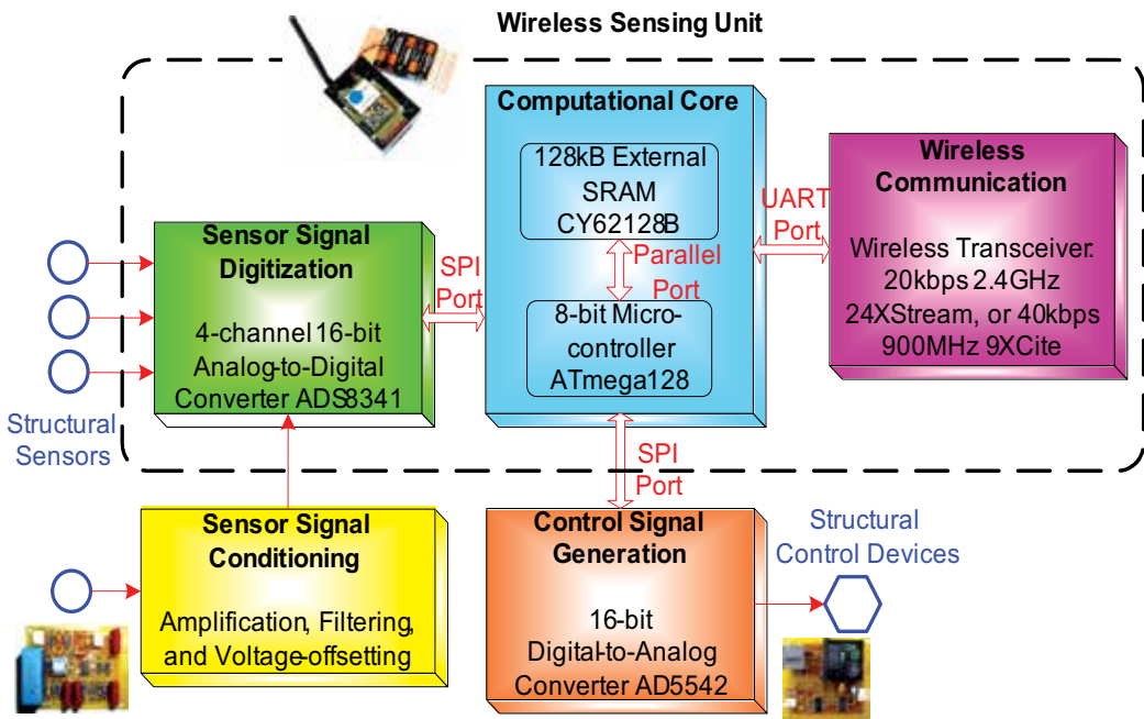
Fig. 1. Functional diagram detailing the hardware design of the wireless sensing unit. Additional off-board modules can be interfaced to the wireless sensing unit to condition sensor signals and issue control commands
