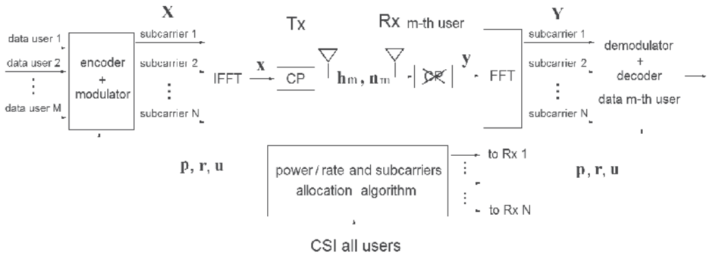
Fig. 2. Multi-user OFDM system with adaptive resources allocation.
