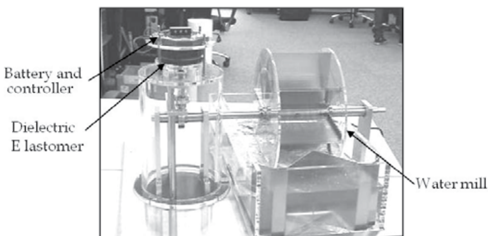
Photo 7. Water mill generator using dielectric elastomer
