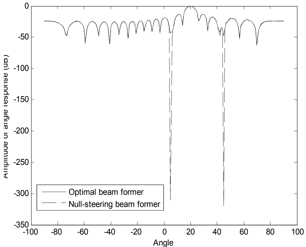
Fig. 19. Angle responses of optimal and null-steering schemes
