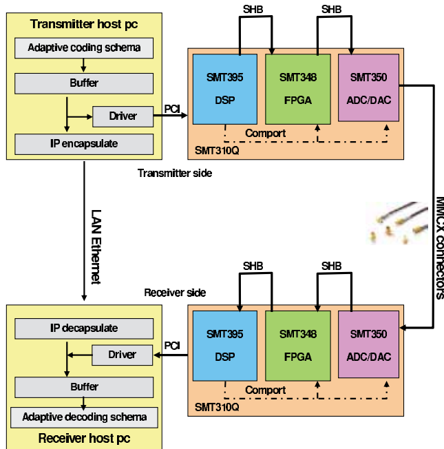
Fig. 4. Transmitter and receiver overview
