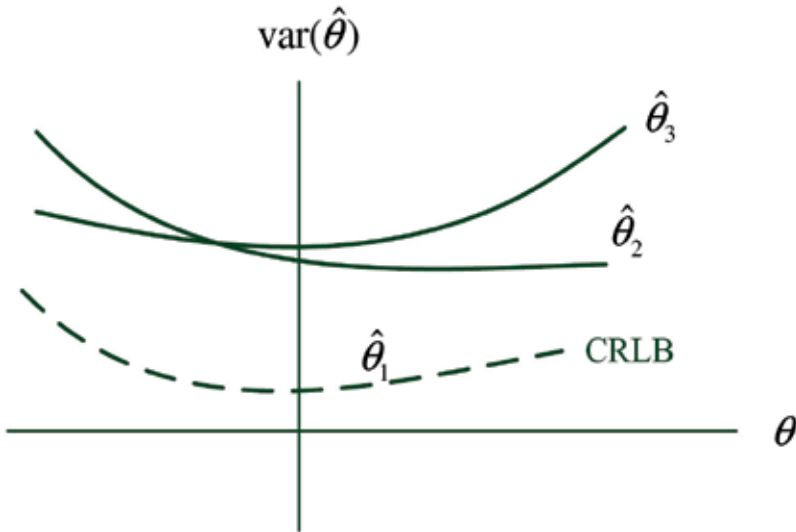
Fig. 1. \hat{\theta}_1 MVU and efficient
