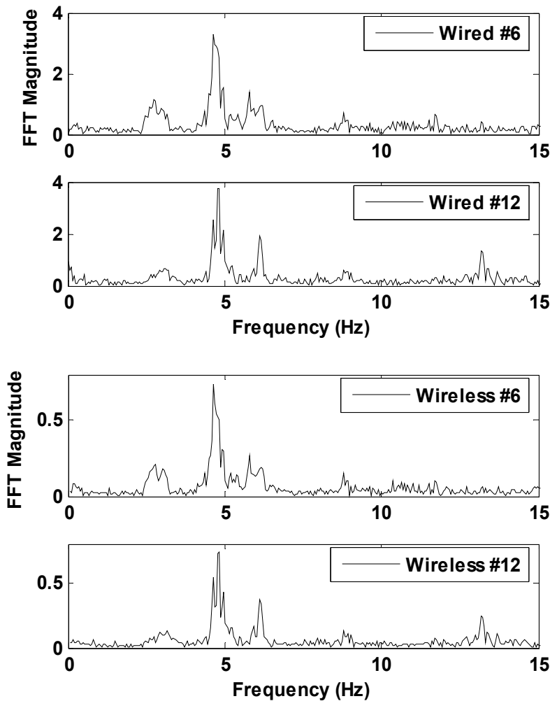
(b) Comparison between FFT to the wired data, as computed offline by a computer, and FFT to the wireless data, as computed online by the wireless sensing units
