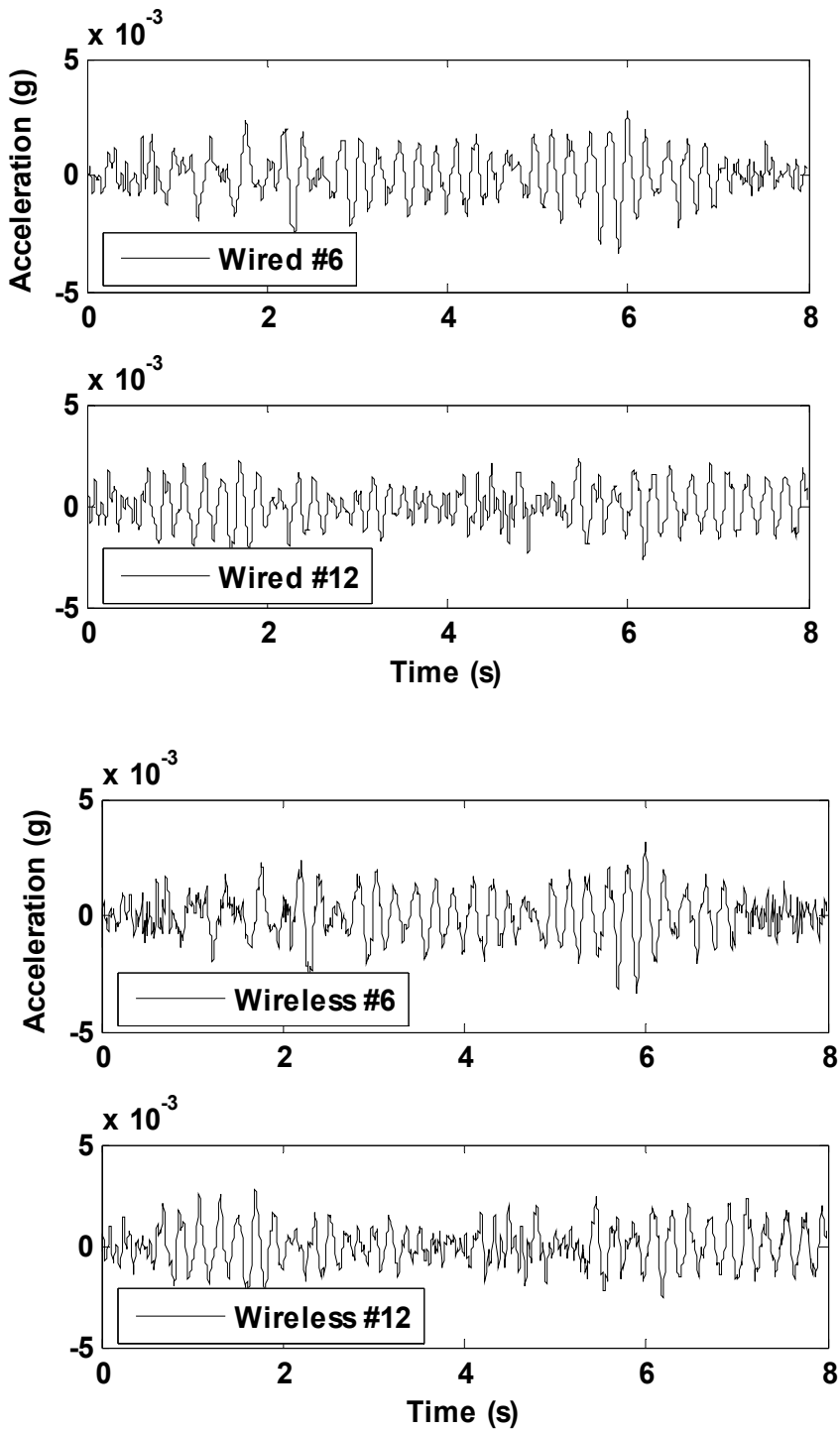
(a) Comparison between wired and wireless time history data
