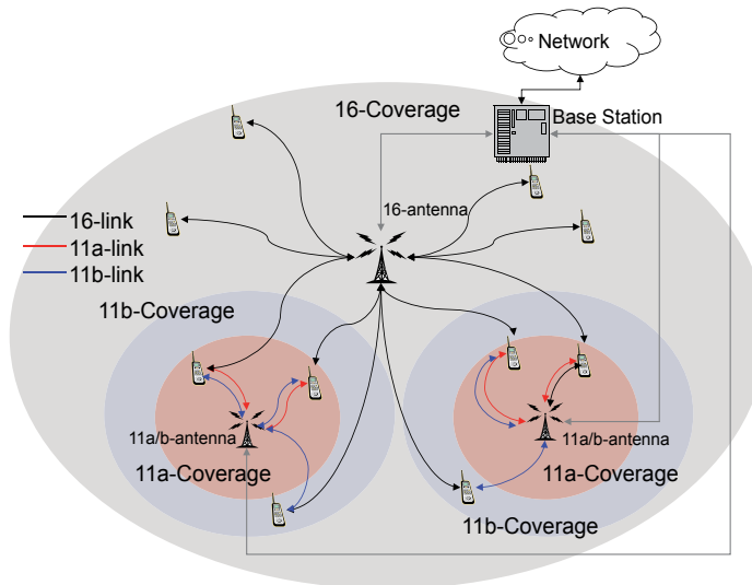
Fig. 1. Assumed wireless access network.
