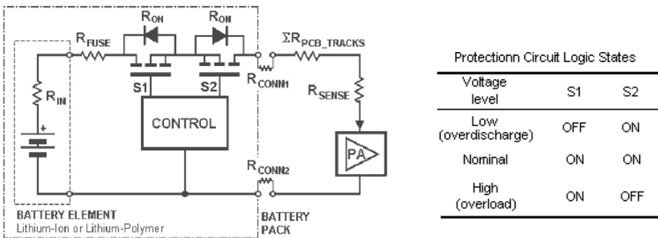
Fig. 3. Detail of an Ion-Lithium battery internal protection circuit and its true table
