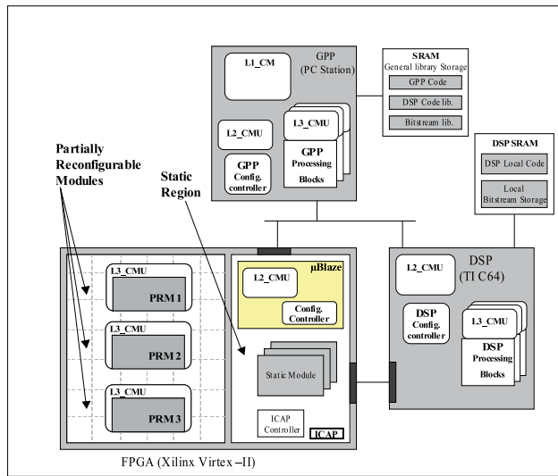
Fig. 8. example of the hierarchical configuration management mapping
