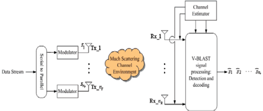
Fig. 12. Block diagram of V-BLAST systems
