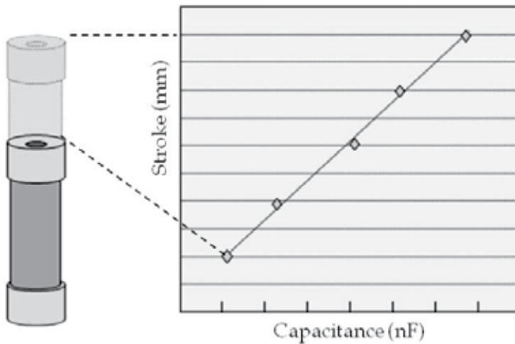
Fig. 6. Linear relation between capacitance and stroke of actuator (Kornbluh et al., 2004b)
