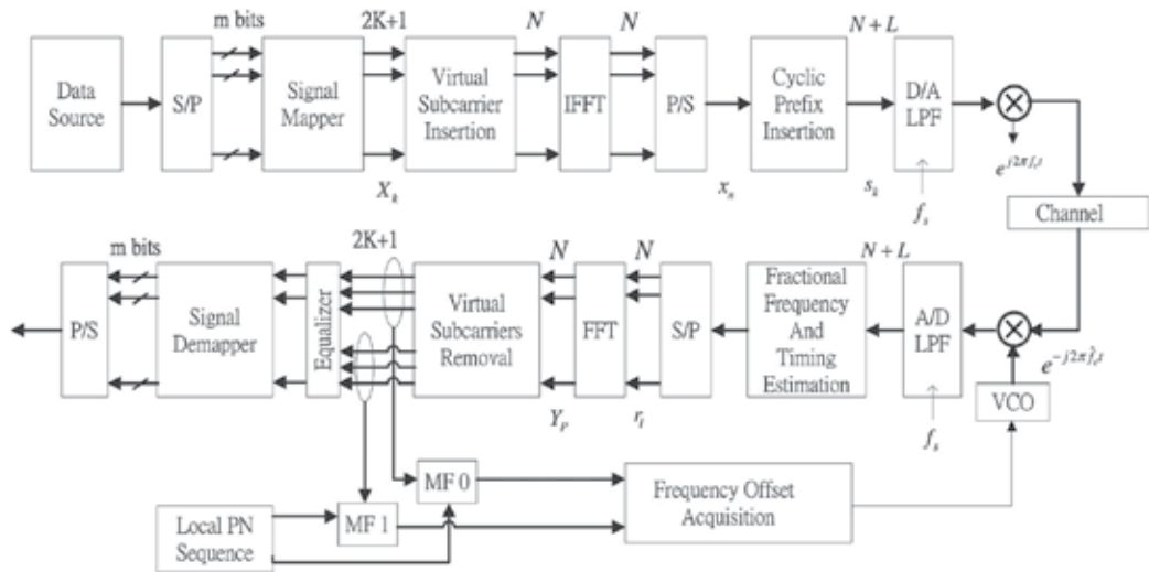
Fig. 8. The OFDM transceiver (Lin, 2006a)
