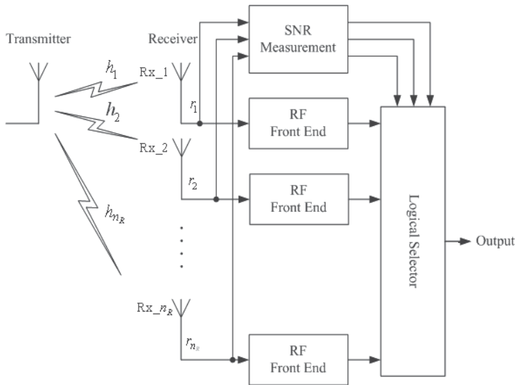
Fig. 1. Block diagram of selection combining scheme
