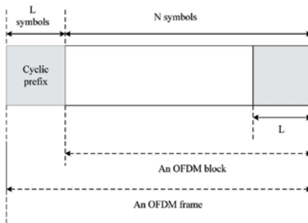
Fig. 3. An OFDM symbol with a cyclic prefix
