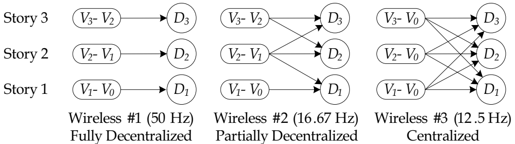
Fig. 16. Various decentralized and centralized information feedback
