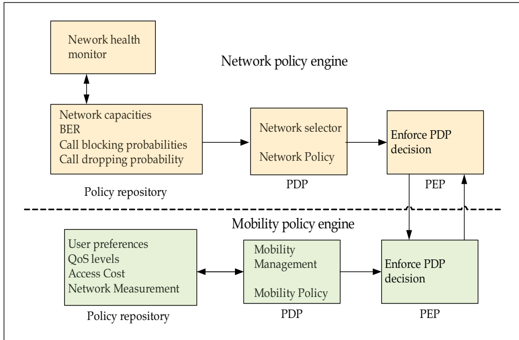
Fig. 4. Policy-based admission control framework
