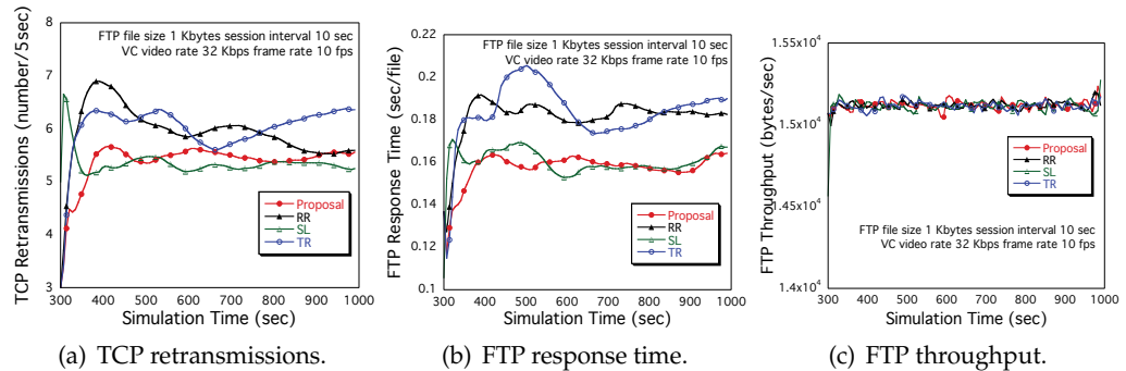
Fig. 12. Transition of TCP and FTP on FTP file size 1K bytes.
