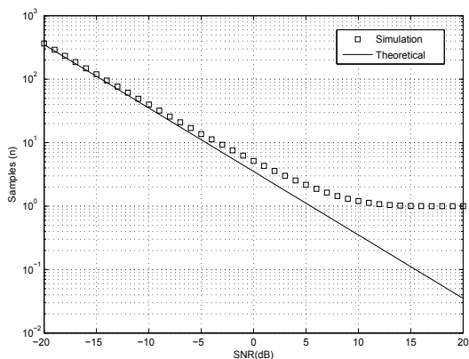
Fig. 8. Average Number of Samples for Detection in Sequential Analysis
