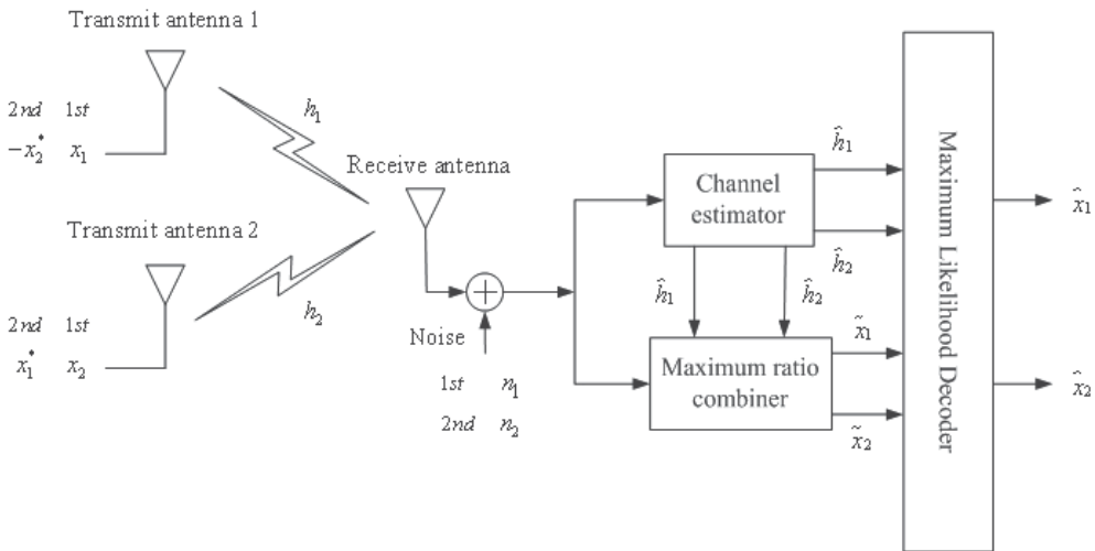
Fig. 5. Block diagram of Alamouti's space-time encoder
