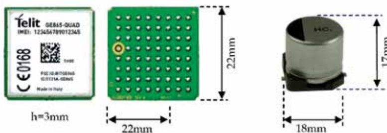
Fig. 4. Comparison between a communication module and the capacitor it requires
