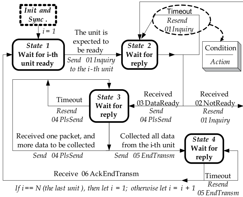
(a) State diagram of the server
