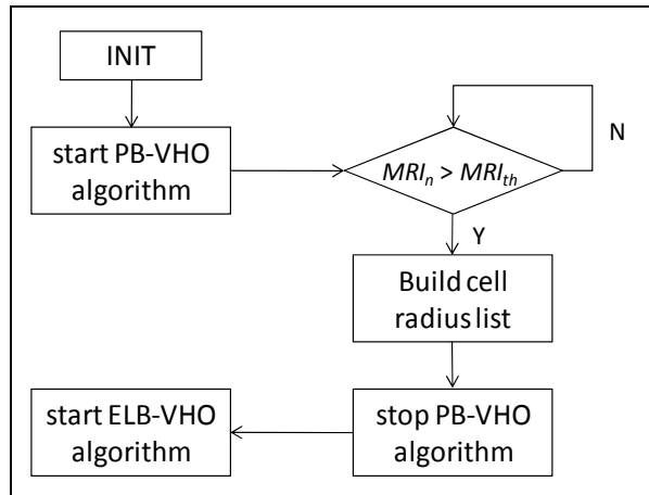
Fig. 7. Flowchart of hybrid vertical handover algorithm
