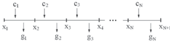
Fig. 20. Scheme of a DP problem showing the system states ( \mathbf{x}_k ), controls ( \mathbf{c}_k ) and costs ( g_k ) at different stages
