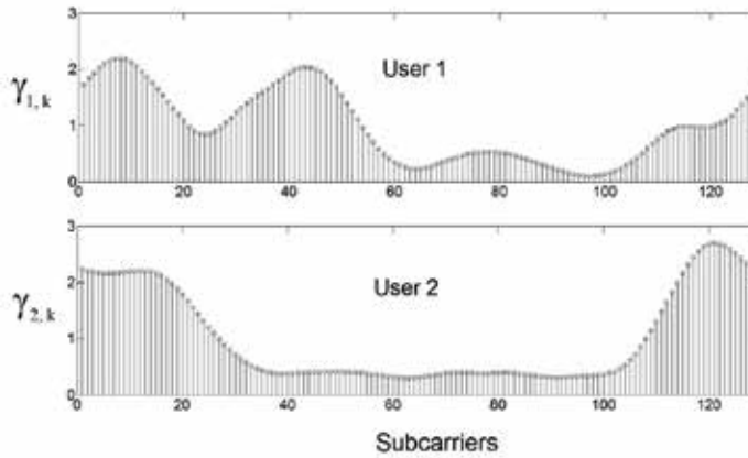
Fig. 7. Normalized subchannel gains at the OFDM subchannels.
