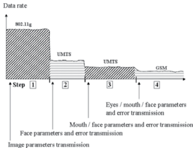
Fig. 9. Standard adaptation as function of the video compression
