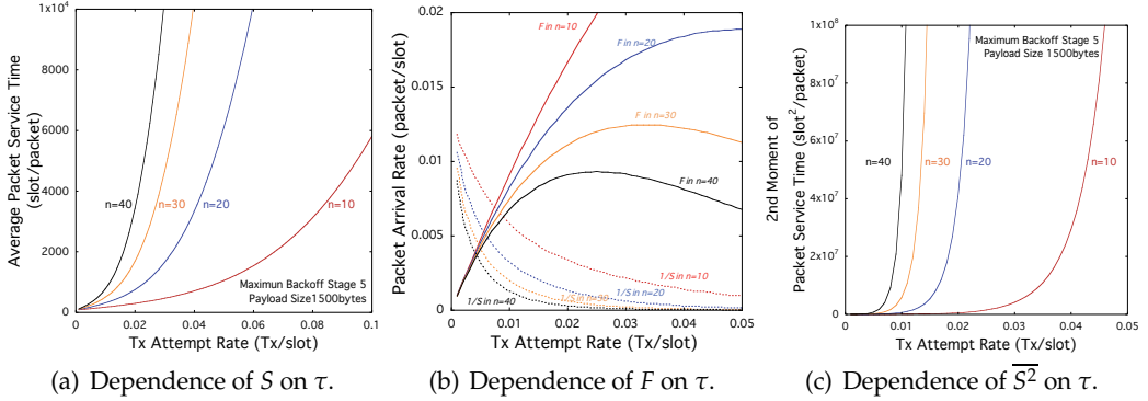
Fig. 4. Dependence of each element on \tau .
