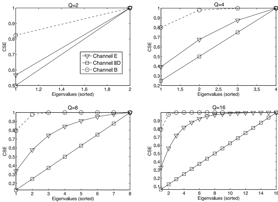
Fig. 3. Cumulative eigenvalue spread for Models B and E from (Erceg, 2003) and iid channel for different group sizes.
