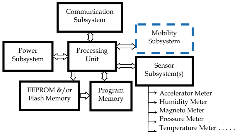
Fig. 1. Block diagram of wireless sensor node
