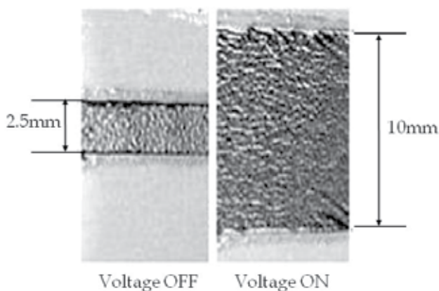
Photo 1. Acrylic elastomers showing 380% linear strain
