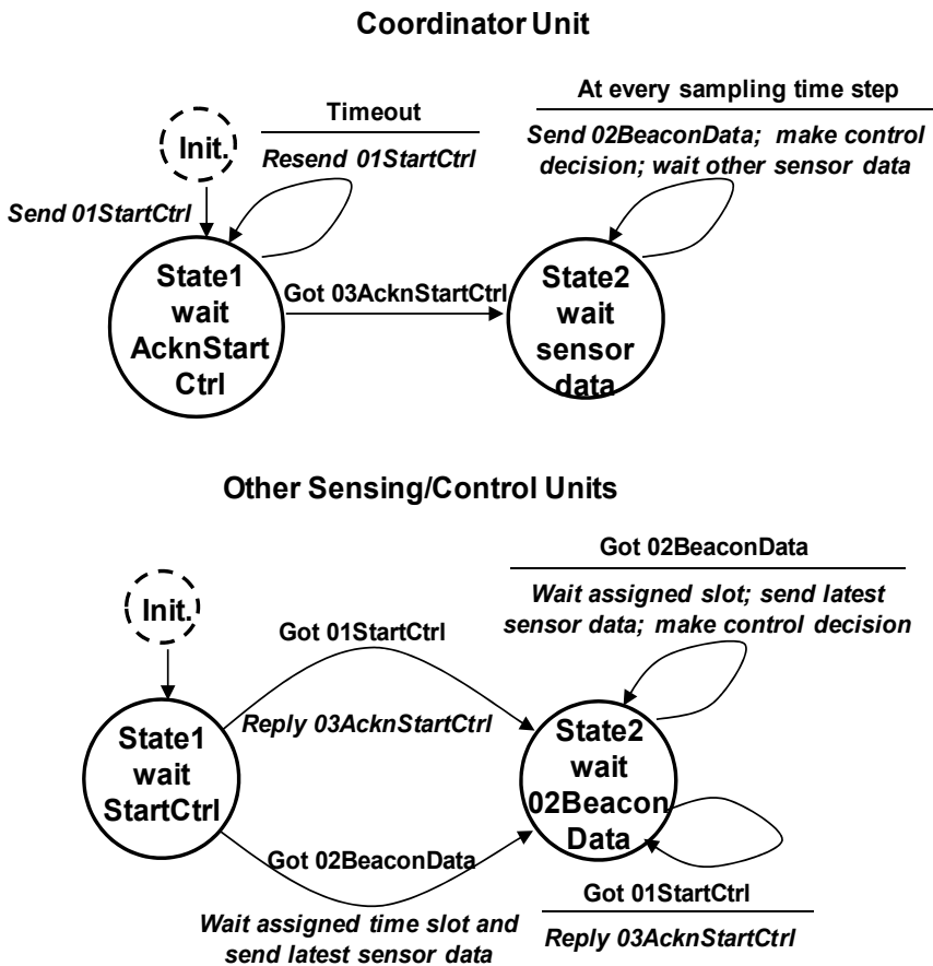
Fig. 12. Communication state diagram of a coordinator unit and other sensing/control units in one wireless subnet
