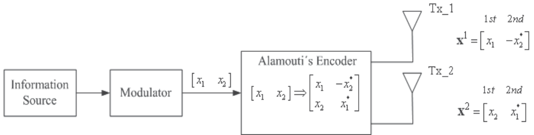
Fig. 4. Block diagram of Alamouti's space-time encoder
