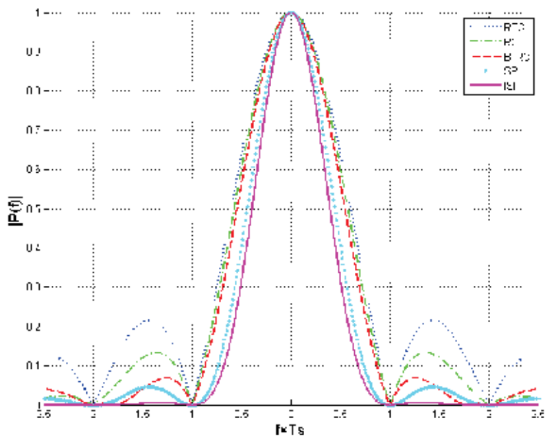
Fig. 5. Comparison of REC, RC, BTRC, SP, and ISP spectrums
