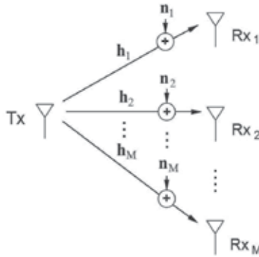
Fig. 3. M-users broadcast broadband channel.
