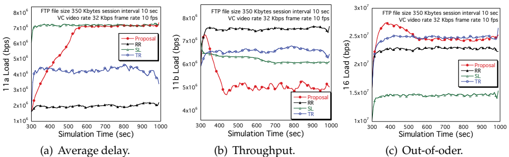
Fig. 15. Distributed traffic load to each wireless system on FTP file size 350K bytes.
