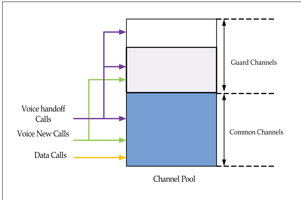
Fig. 3. Guard channel reservation based scheme for voice and data services
