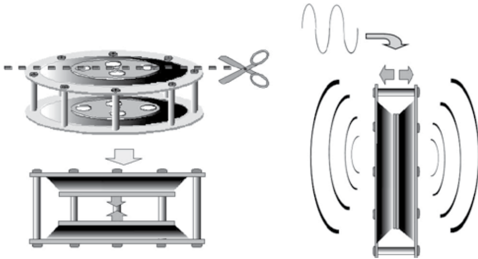
Fig. 5. Structure of speaker using dielectric elastomer (The black shaped part is dielectric elastomer) (Chiba et al., 2007a)
