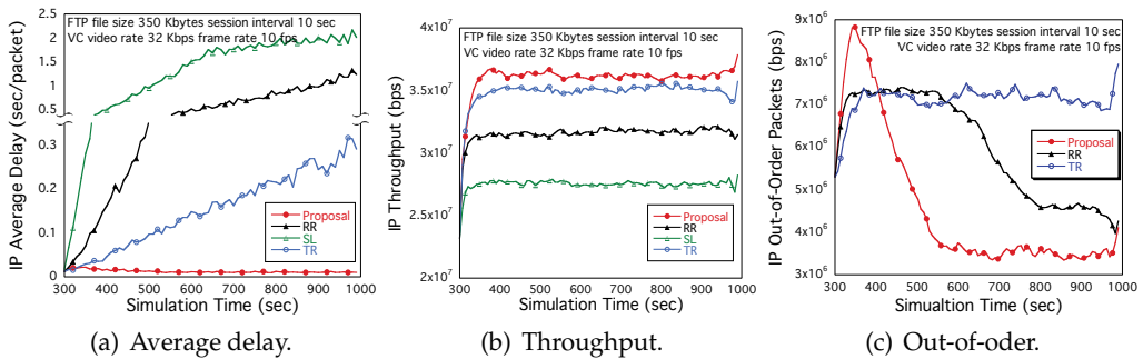
Fig. 14. Transition of IP on FTP file size 350K bytes.
