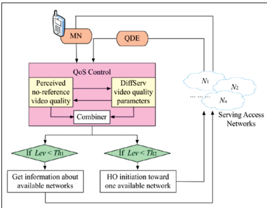
Fig. 3. Proposed network architecture for QoS-based handover
