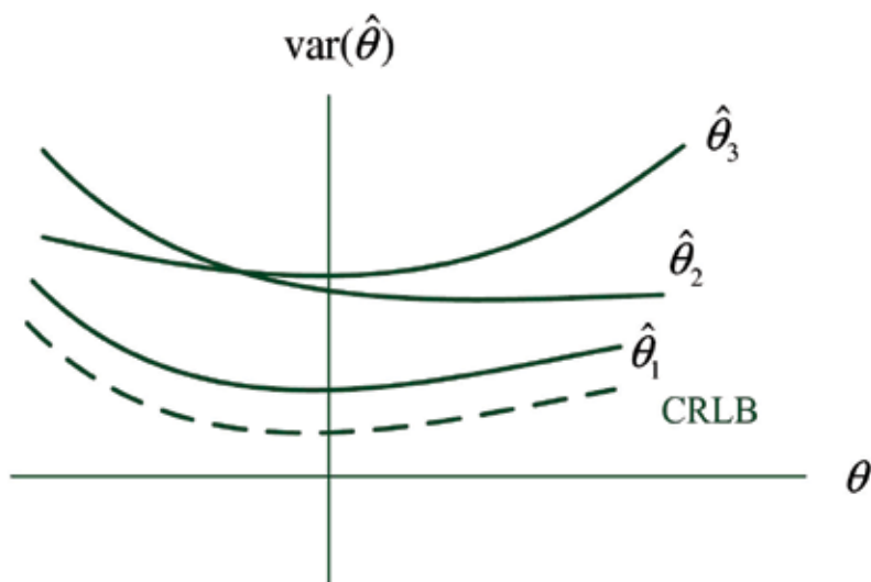
Fig. 2. \hat{\theta}_1 MVU and not efficient
