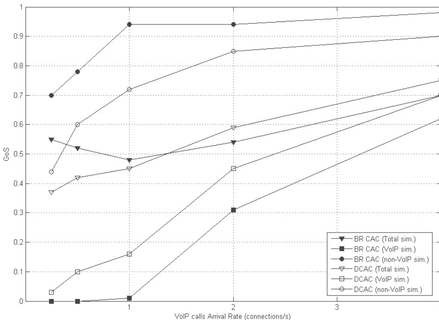
Fig. 8. GoS vs. VoIP Calls Arrival Rate (proposed Bandwidth Reservation (BR) CAC vs. proposed DCAC)
