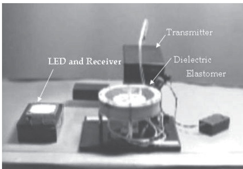
Photo 5. Small scale power generation device & LED controlled by wireless signals
