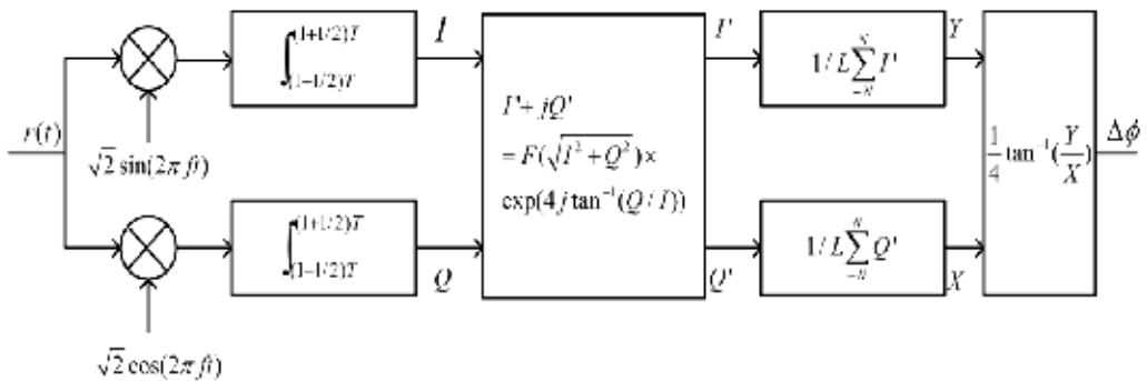
Fig. 8. Feed-forward NDA
