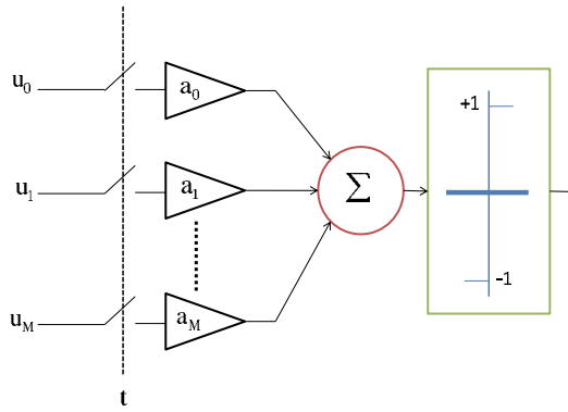
Fig. 11. System model of data fusion system
