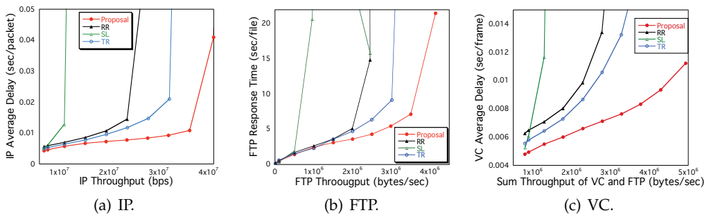
Fig. 18. Dependence of delay on throughput.
