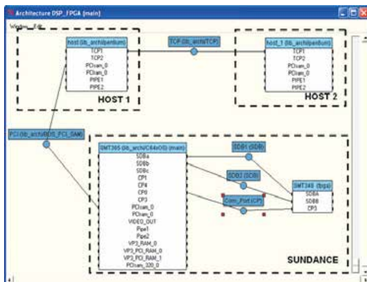
Fig. 10. SynDEX model
