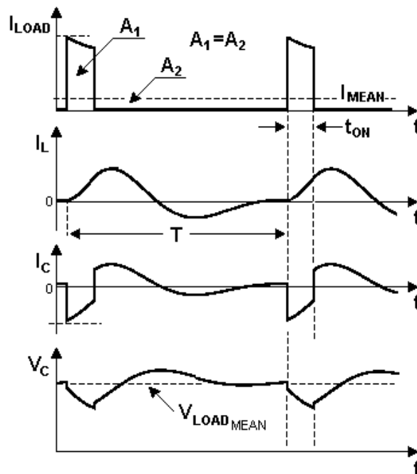
Fig. 18. Current and voltage for the power supply of a wireless system with LC filtering
