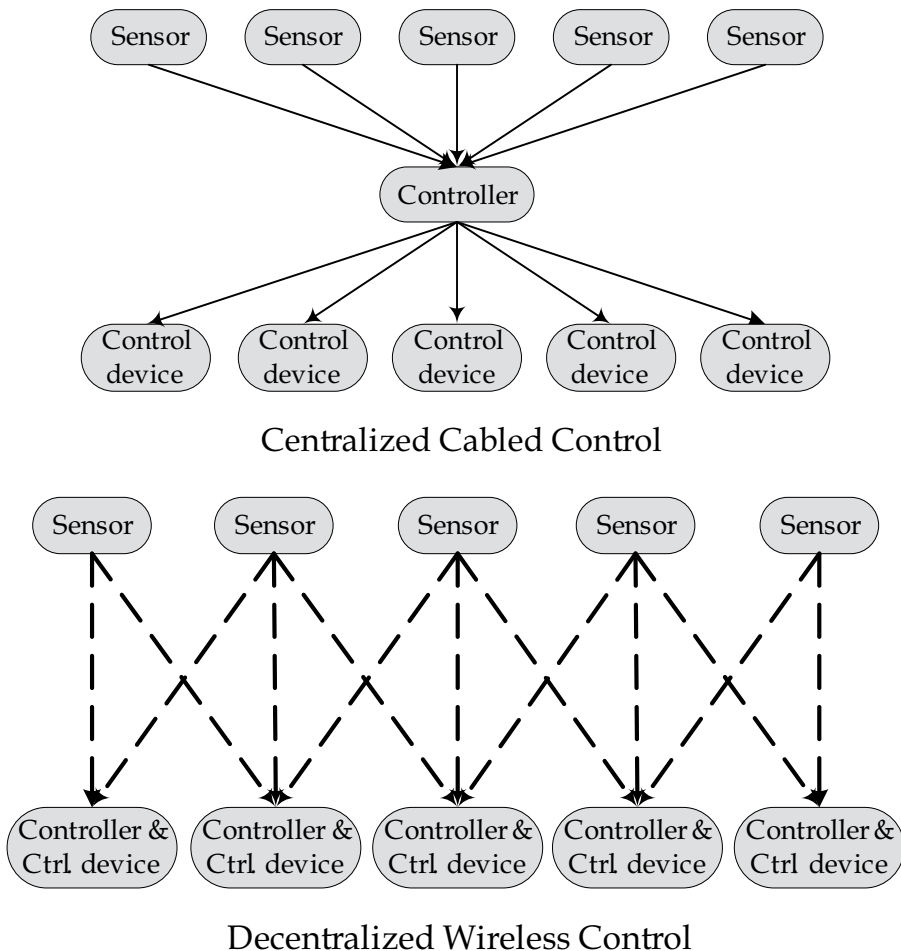
Fig. 10. Centralized and decentralized control systems
