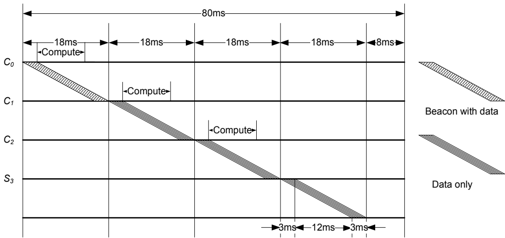
Fig. 14. Communication sequence in a wireless structural control network
