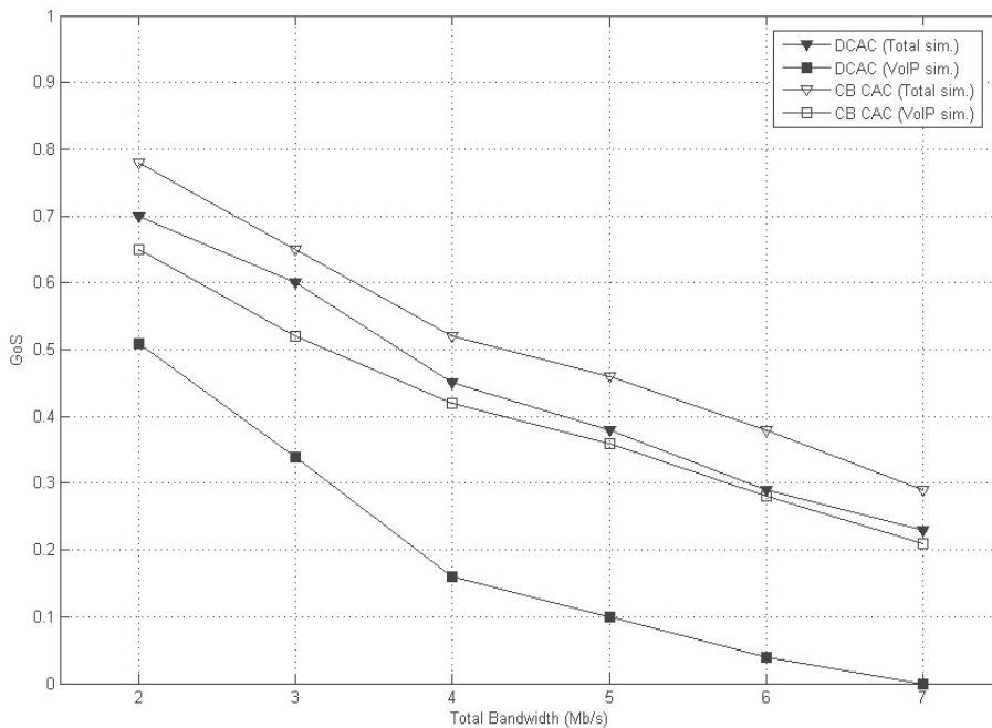
Fig. 9. GoS vs. Total System's Bandwidth (proposed DCAC vs. Capacity-based (CB) CAC)
