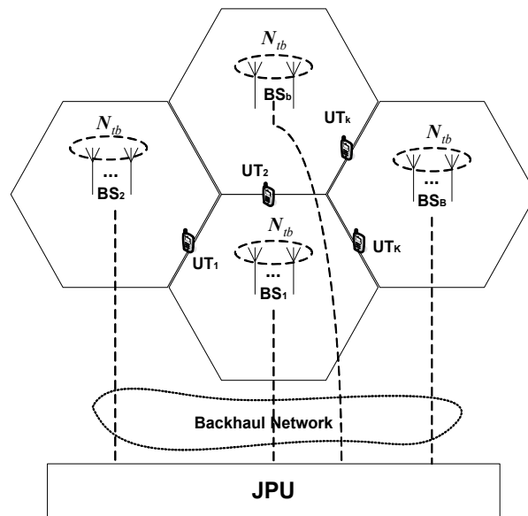
Fig. 2. Multi-cell system overview
