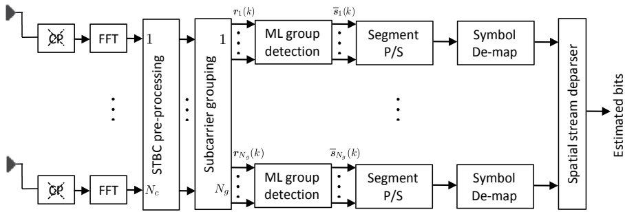
Fig. 2. Receiver architecture for MIMO-GO-CDM.
