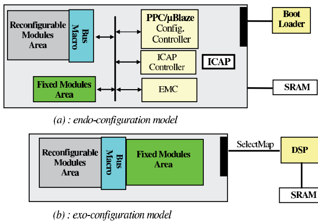
Fig. 6. Exo and Endo FPGA configuration
