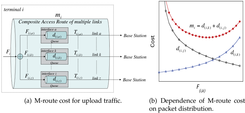
Fig. 5. M-route for upload traffic.
