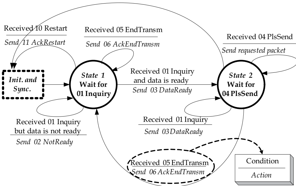
(b) State diagram of a wireless sensing unit.
