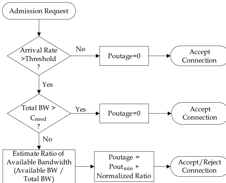
Fig. 5. Dynamic connection admission control (flowchart)
