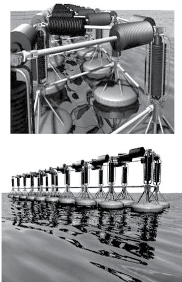
Fig. 14. Conceptual rendering of wave power generator system using dielectric elastomers
