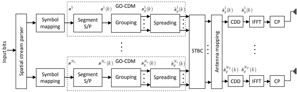
Fig. 1. Transmitter architecture for MIMO GO-CDM.
