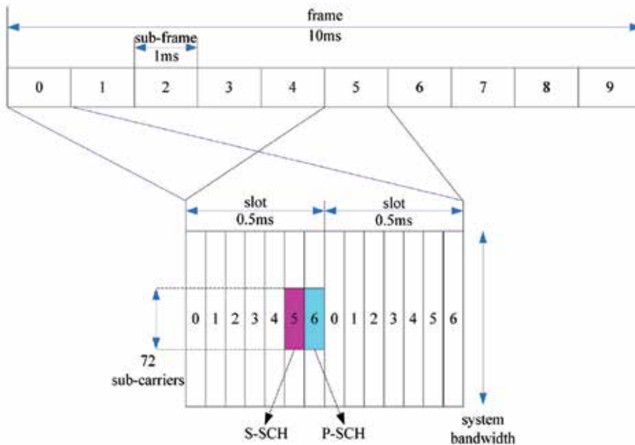
Fig. 9. LTE frame structure
