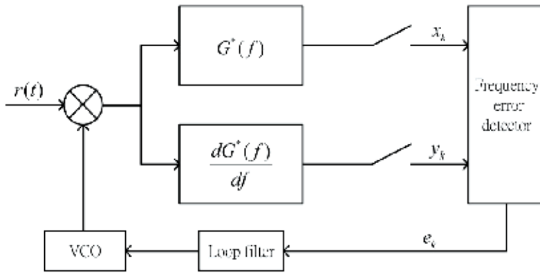
Fig. 5. NDA loop algorithm
