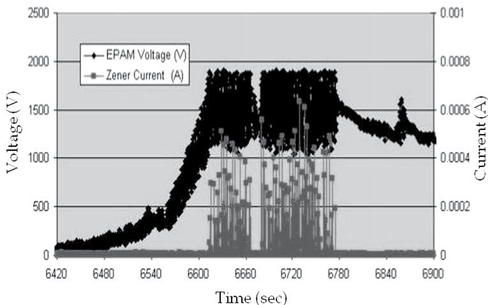
Fig. 11. Electricity generated by ten centimeter-high waves
