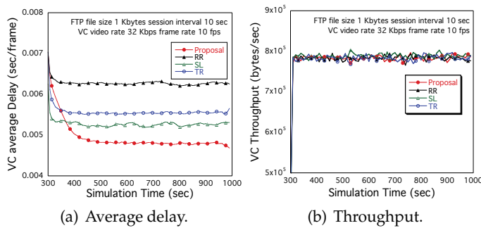
Fig. 13. Transition of VC on FTP file size 1K bytes.
