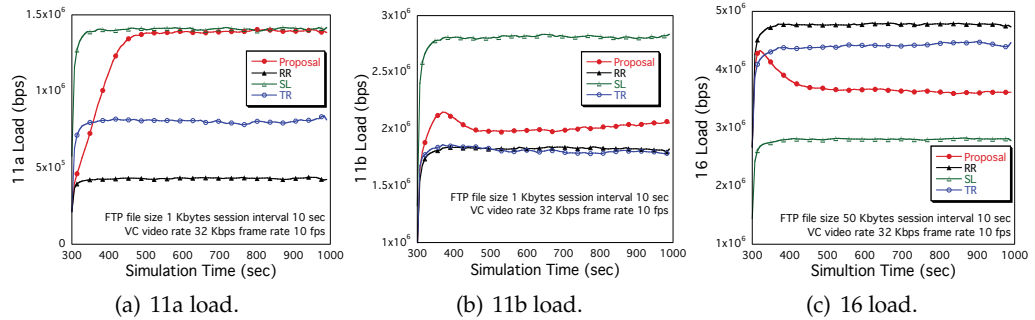
Fig. 11. Distributed traffic load to each wireless system on FTP file size 1K bytes.
