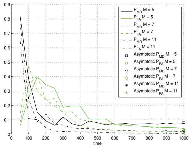
Fig. 13. Data fusion scheme considering sequential analysis decision from each sensor ( P_{M,I} = 0.1, P_{F,I} = 0.3 ).
