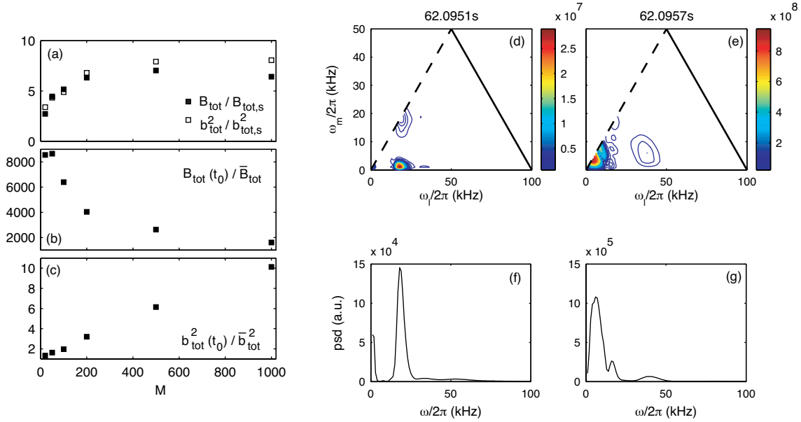
Figure 5. (Colour) Left: effect of the number of samples on the calculation of higher order spectra. (a) ratio of the total bicoherence b_{tot}^2 ( \square ) and of the total bispectrum B_{tot} ( \blacksquare ) to the corresponding quantities, b_{tot,s}^2 and B_{tot,s} calculated over the surrogate series. (b) ratio of the total bispectrum B_{tot} computed at the time t_0 where it is maximum to the value \bar{B}_{tot} computed in a 4 ms time window before t_0 . (c) same as (b) but for the total bicoherence b_{tot}^2 . Right-top: Bispectrum of the magnetic perturbations, calculated over 200 samples, measured approximately 800 \mu s (d) and 200 \mu s (e) before the ELM. Right-bottom: power spectral density (psd) of magnetic perturbations, arbitrary units, averaged over 200 samples, computed 800 \mu s (f) and 200 \mu s (g) before the ELM.
