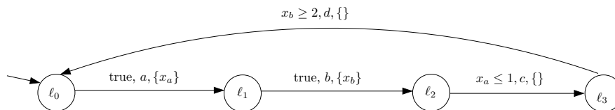
FIGURE 3.2. A timed automaton with more than one clock.
