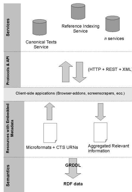
Figure 5: Separation of logical layers in the proposed linking framework between primary and secondary sources.
