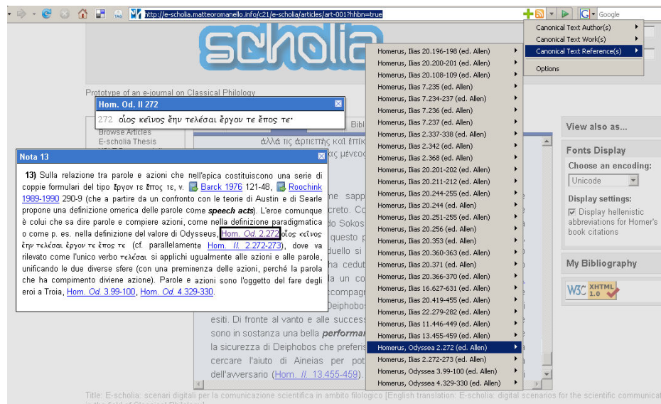
Figure 4: Screenshot of E-scholia prototype of an advanced e-journal on classical philology. Canonical texts references (1) becomes dynamically links to the full-text of the passage referred to which is retrieved from some CTS repository available on the Web. Furthermore an extended version of Operator extension for Mozilla Firefox allows to detect the meaning of microformatted references and to perform upon them some actions on the client-side (3).
