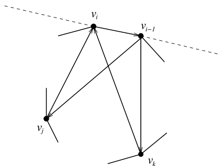
FIGURE 1. A convex polygon.
