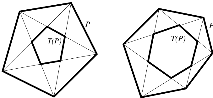
FIGURE 2. The pentagram map.
