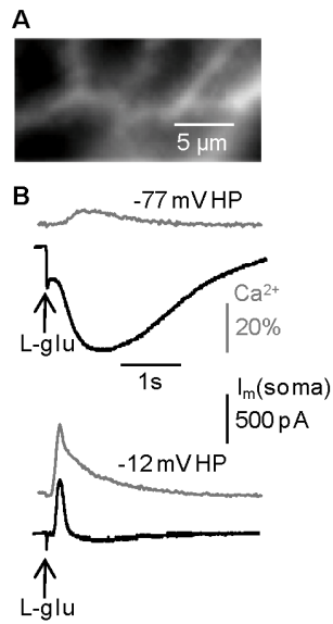
FIGURE 3. \text{Ca}^{2+} signals mediated by mGluR1 activation and elicited by L-glutamate photorelease in cerebellar Purkinje neurons. (A) Fluorescence image of a sub-region of a PN filled with Oregon Green BAPTA-5N. (B) Somatic membrane current (black traces) and \text{Ca}^{2+} signals (gray traces) from the region in A and mediated by mGluR1 activation and elicited by L-glutamate photorelease; left: signals at -77 mV holding potential (HP); right: signals at -12 mV holding potential.
