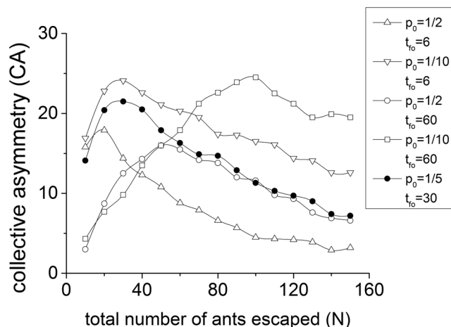
Fig. 7. CA vs. N of alarm pheromone model. The solid dots denote the best-fit simulation result with the following parameters: p_0 = 1/5 and t_{fo} = 30 seconds. The others denote 4 combinations of different parameters when p_0 is assigned a value of 1/2 and 1/10 , and t_{fo} is assigned a value of 6 and 60 seconds. This demonstrates that the initial increasing and then decreasing pattern is robust. All the points are averaged over 1000 runs.
