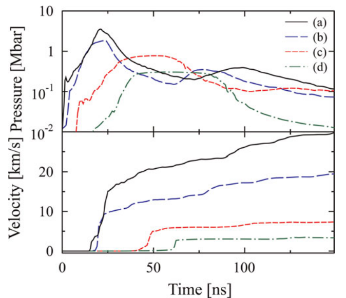
Fig. 3. (Color online) Rear surface velocity and front surface pressure histories for different cases described in Table 1.
