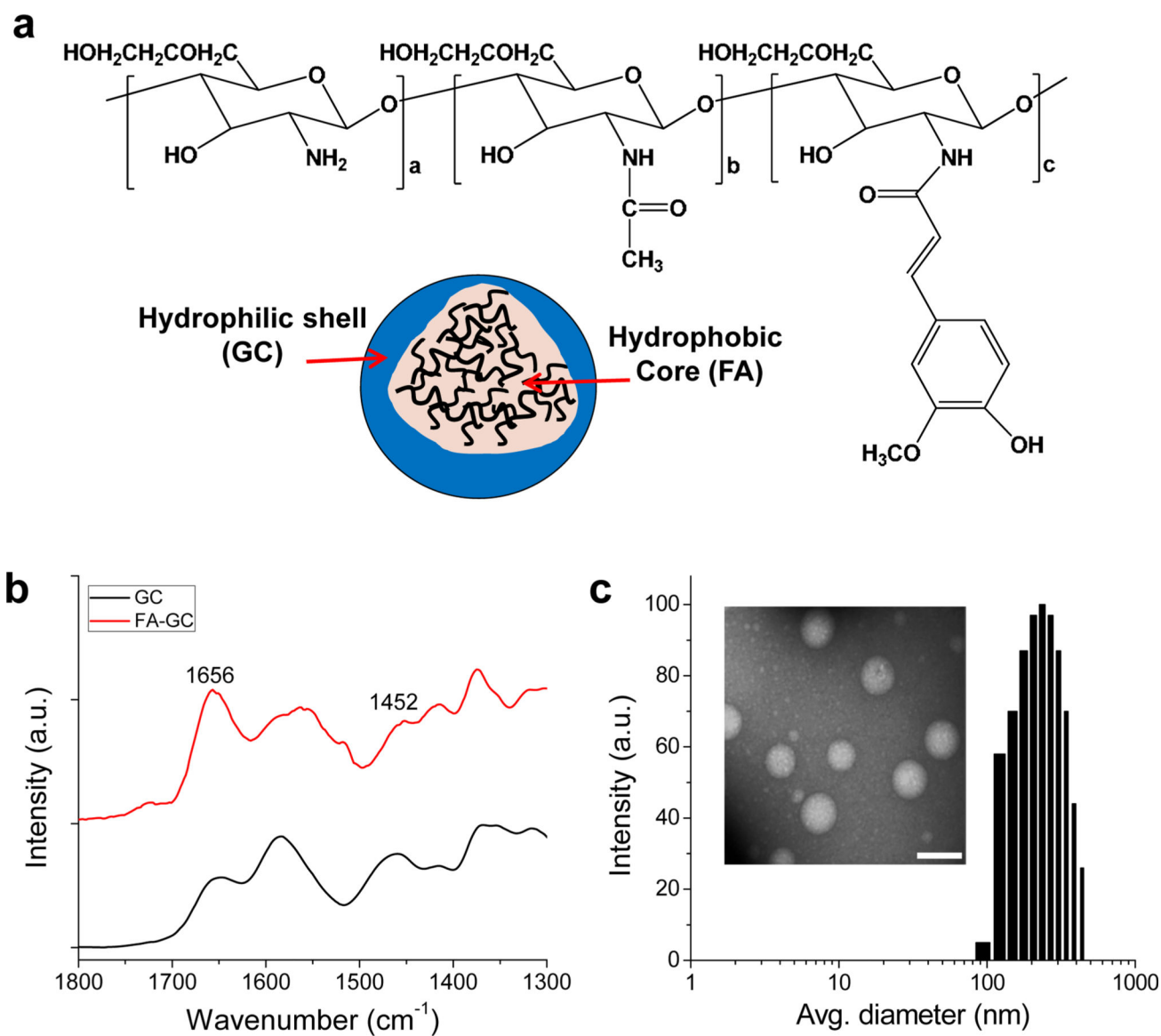
Figure 1. FA-GC nanoparticles
