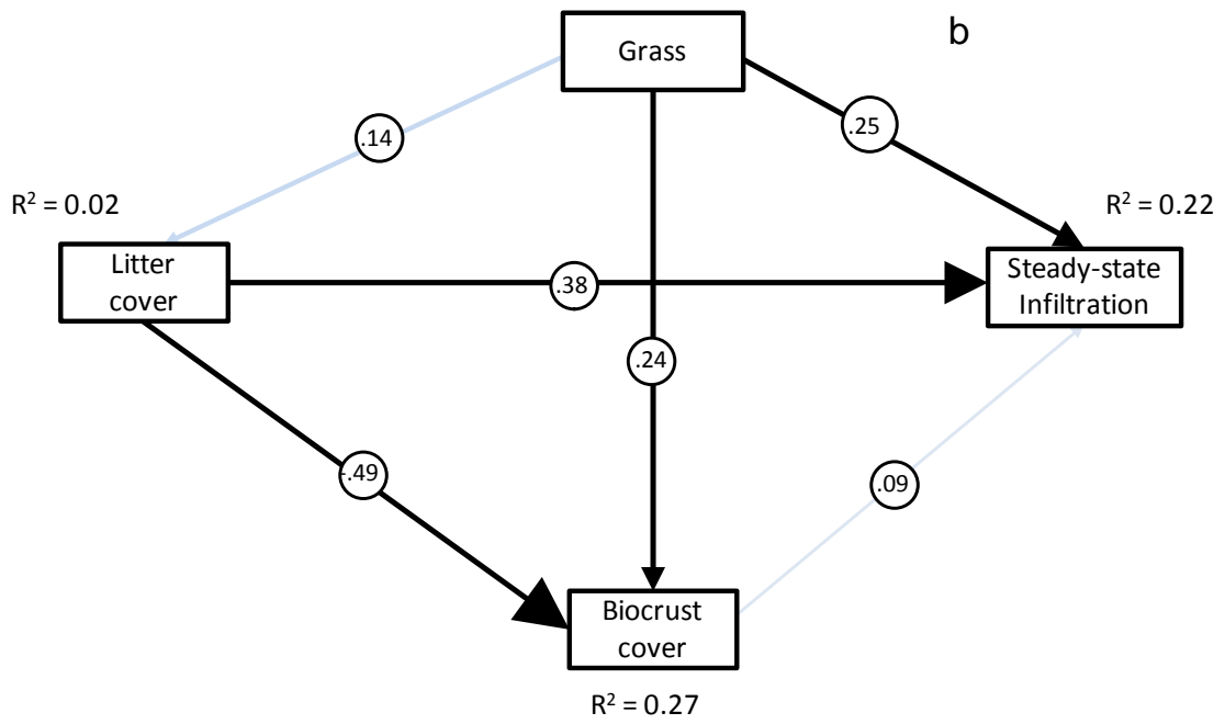
53 Figure 3. Structural Equation Models for shrubland (a) and grassland (b).
