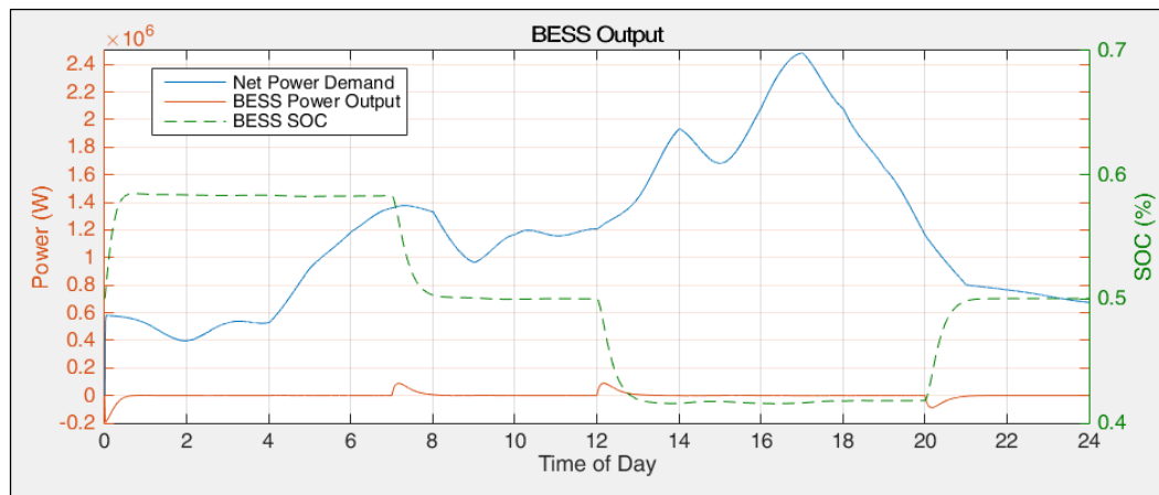
Figure 6.5.12: BESS Power Output vs SOC, Grid-Connected
