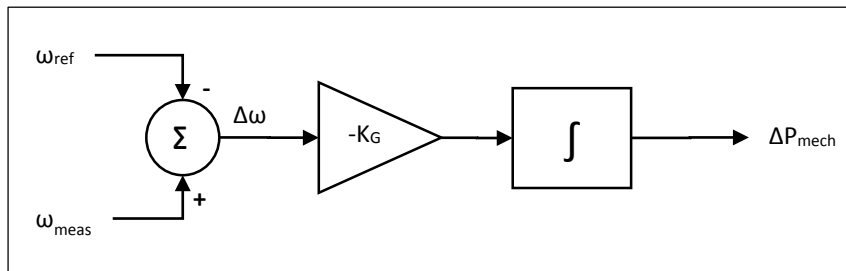
Figure 3.3.1: Isochronous Control
