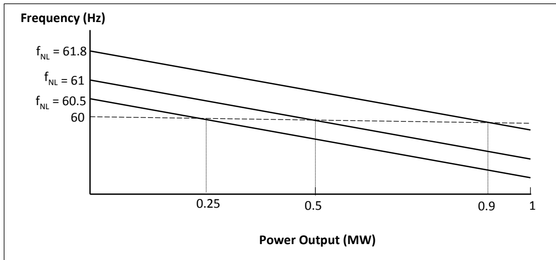
Figure 3.3.5: Adjusting No-Load Frequency
