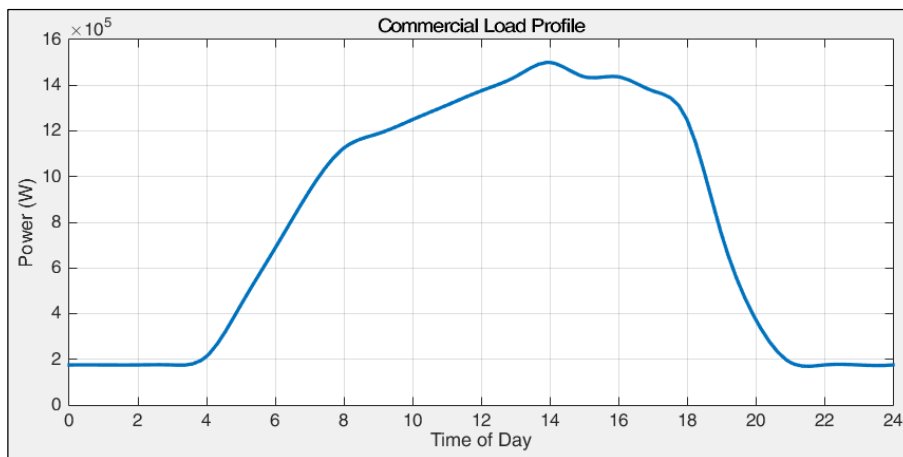
Figure 6.4.8: Commercial Load Profile
