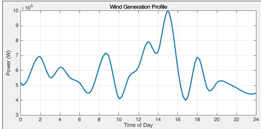
Figure 6.4.12: Wind Turbine Generation Profile for the city of Key Biscayne (3/20/2009 @ 60m)
