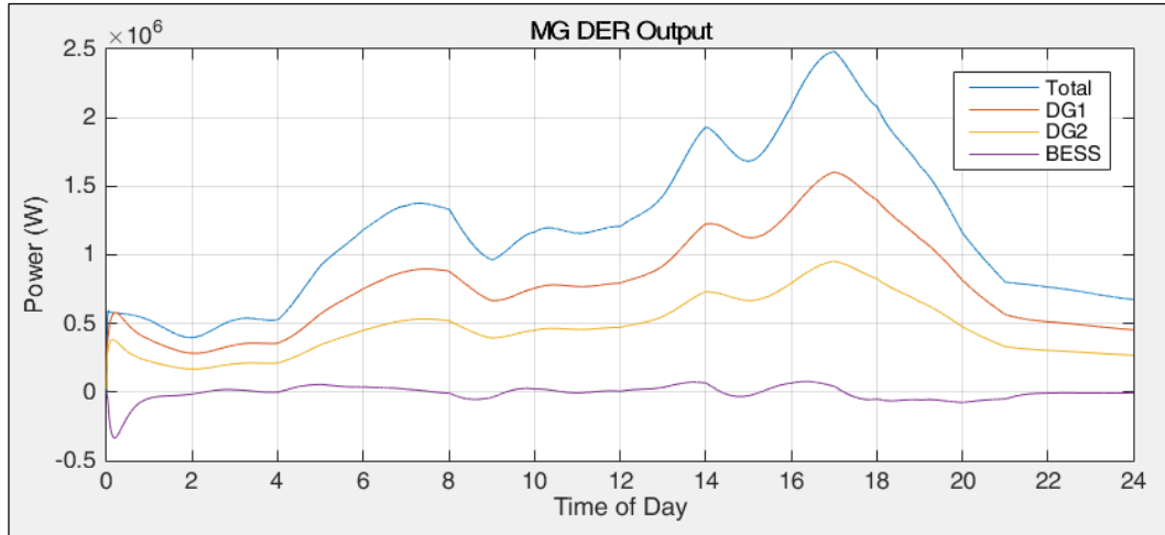
Figure 6.5.3: MG DER Output, Islanded
