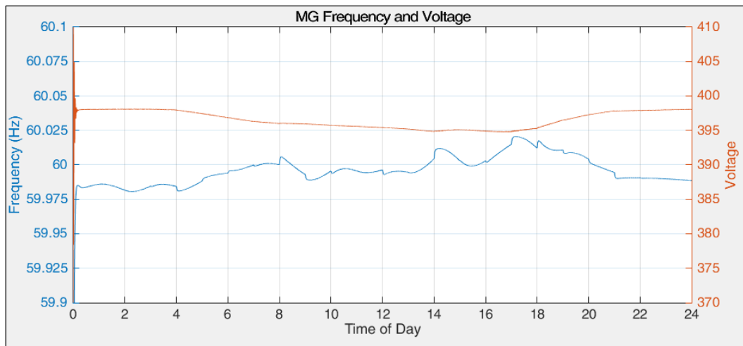
Figure 6.5.7: MG Frequency and Voltage, Islanded
