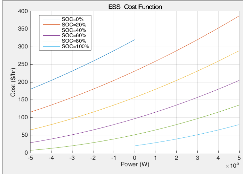
Figure 4.3.1: Energy Storage System Cost Function
