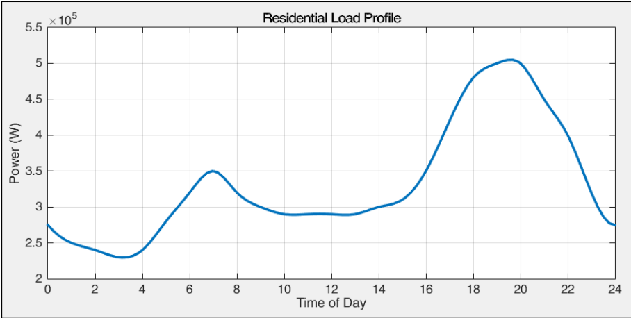
Figure 6.4.10: Residential Load Profile
