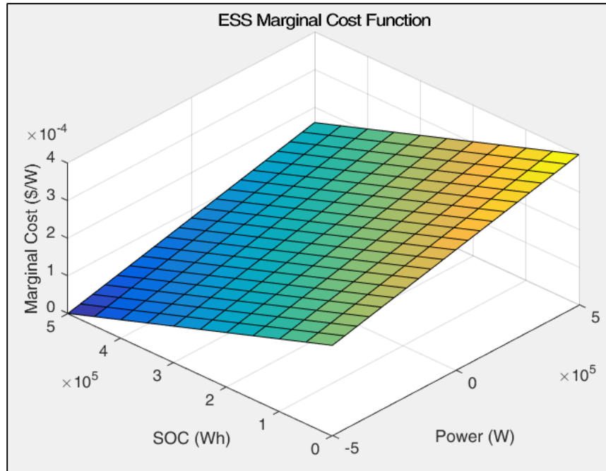
Figure 4.3.4: Energy Storage System Marginal Cost Function Surface
