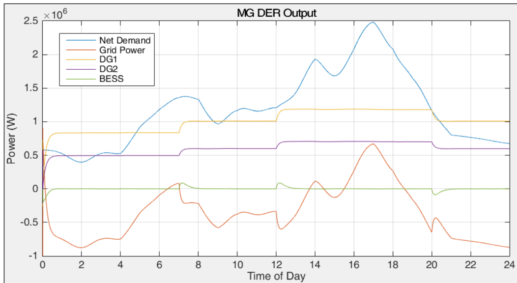
Figure 6.5.9: MG DER Output, Grid-Connected
