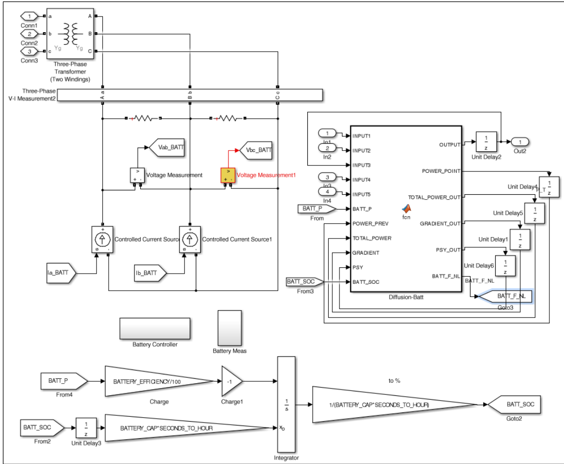
Figure 6.4.6: Simulink BESS Subsystem
