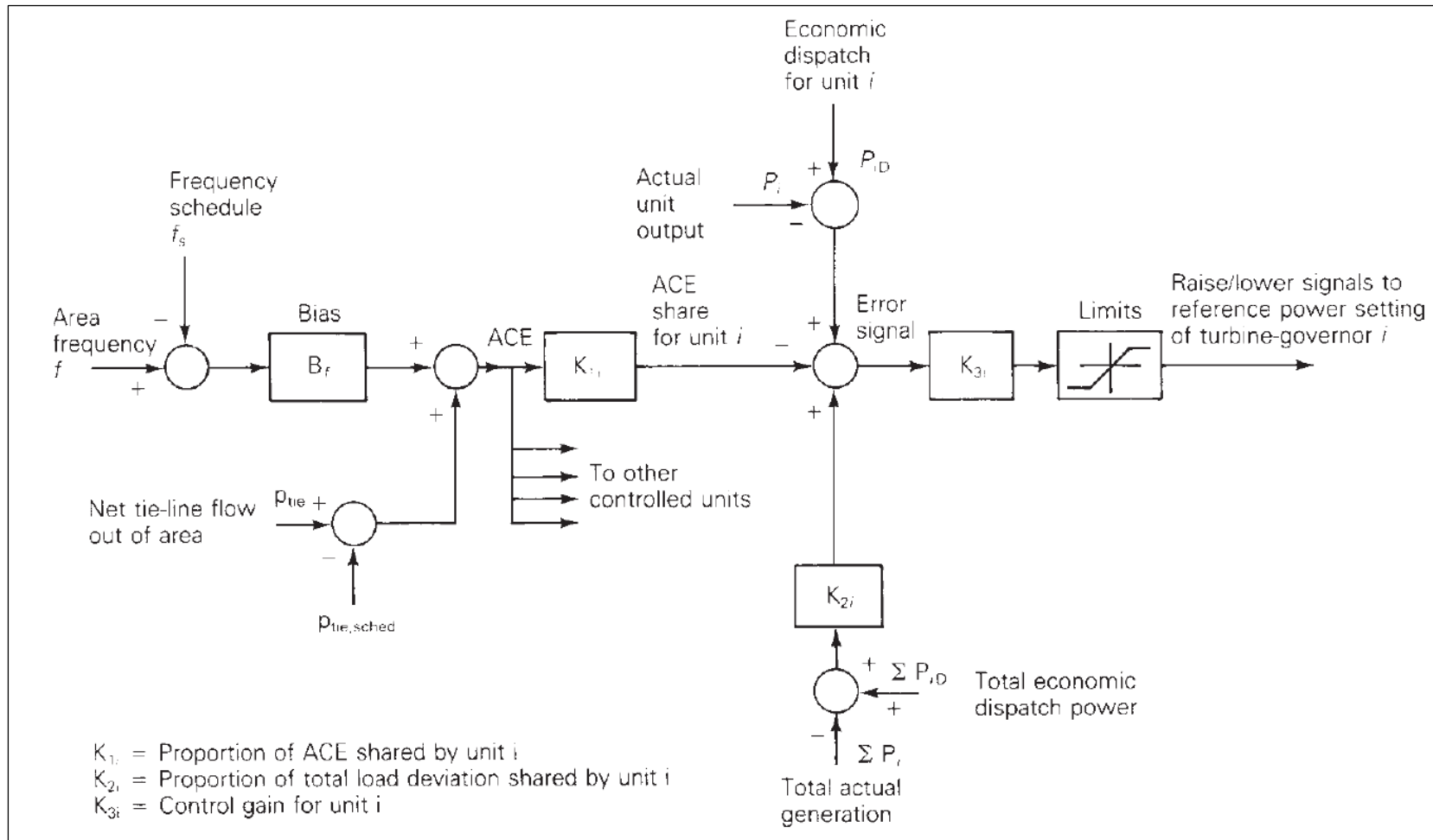
Figure 3.2.1: Automatic Generation Control [27]
