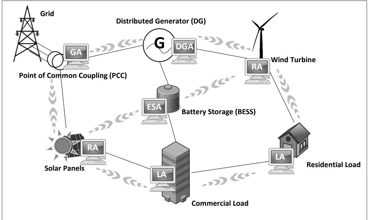
Figure 4.3.5: Microgrid MAS Agent Assignments
