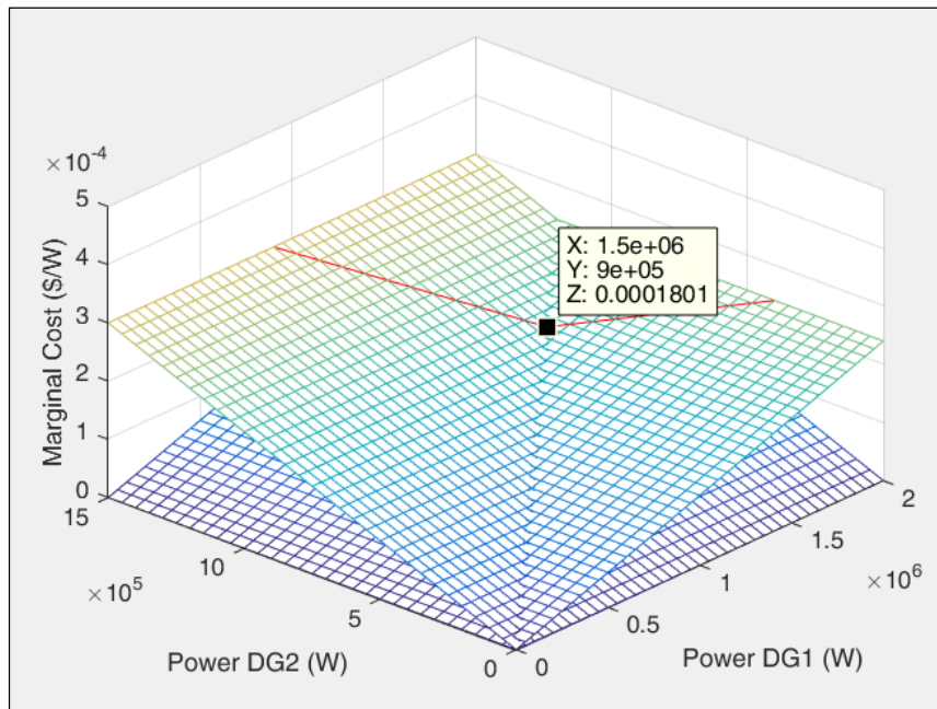
Figure 5.4.4: Islanded MG Marginal Cost Functions ED
