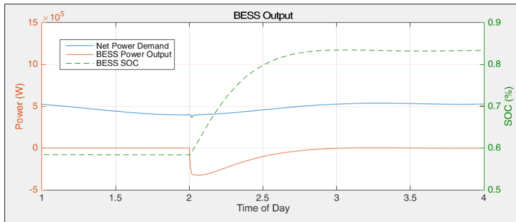
Figure 6.5.15: BESS Power Output vs SOC, Islanding
