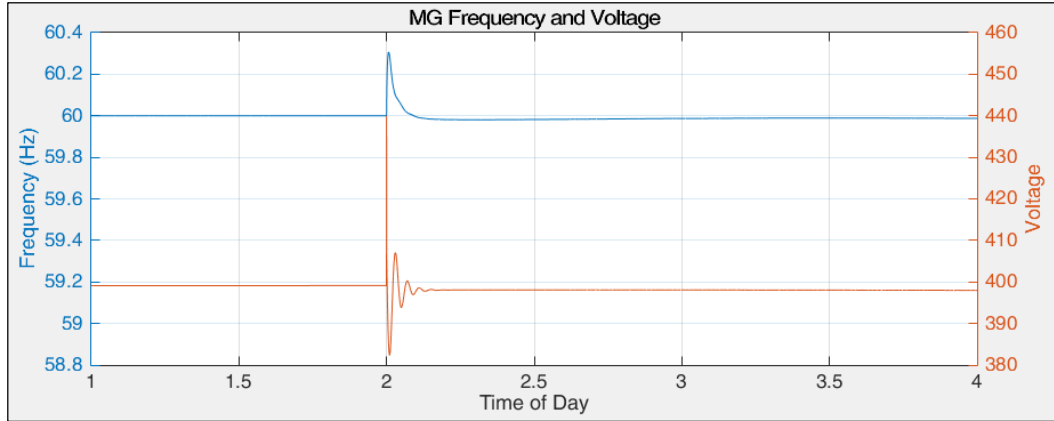
Figure 6.5.16: MG Frequency and Voltage, Islanding
