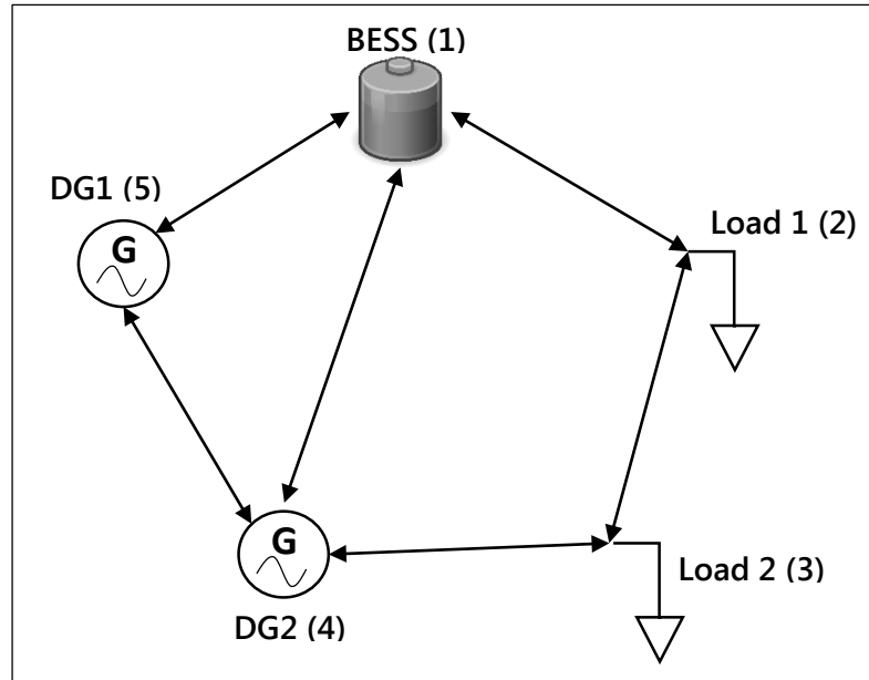
Figure 6.6.6: Experimental MG Network Topology
