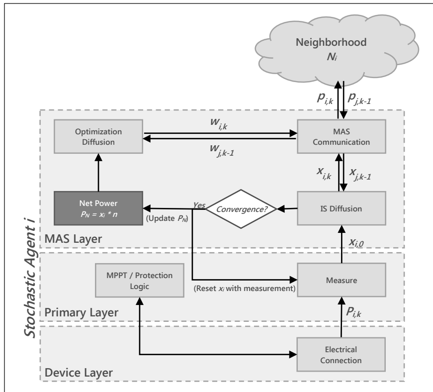
Figure 6.2.1: Stochastic Agent Block Diagram
