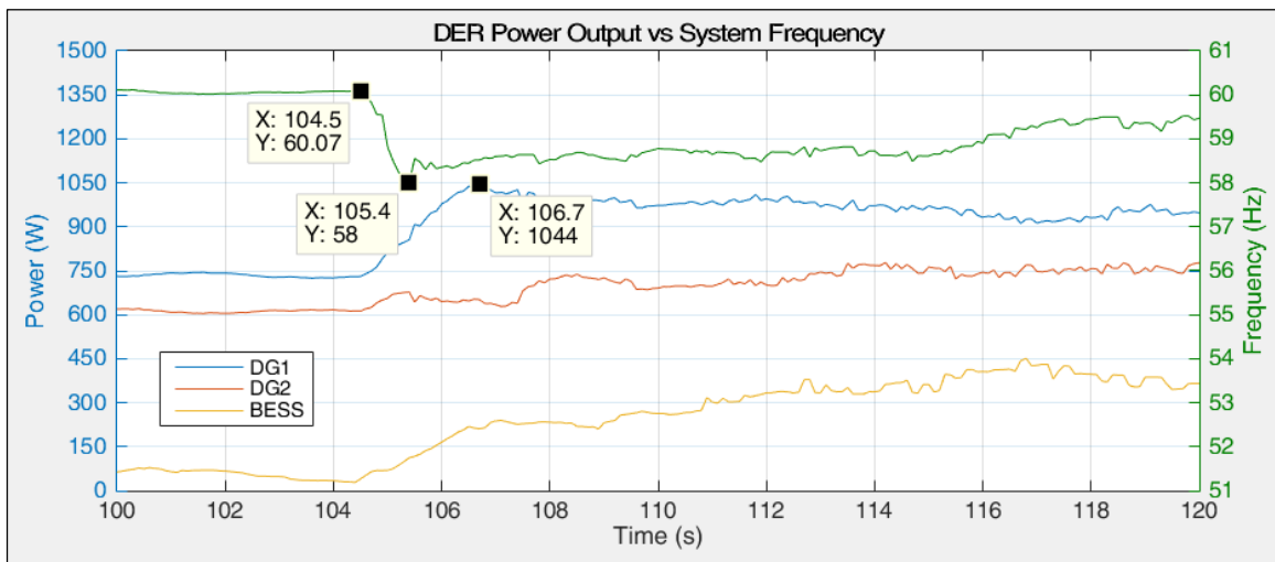
Figure 6.7.4: Experimental DER Output vs Frequency, Close-Up
