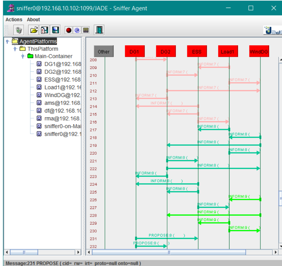
Figure 6.3.4: JADE Sniffer, PROPOSE message on IS convergence
