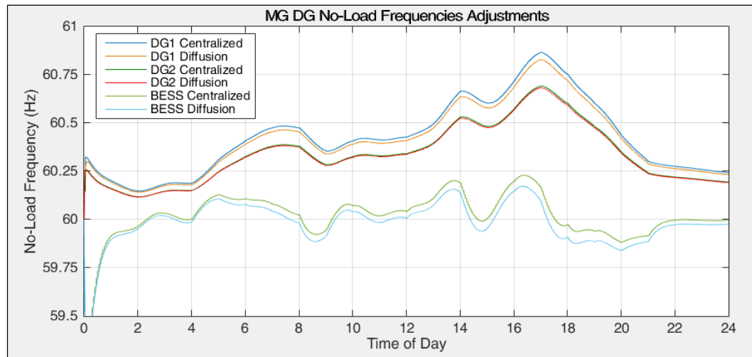
Figure 6.5.4: DER No-Load Frequency Adjustments, Islanded
