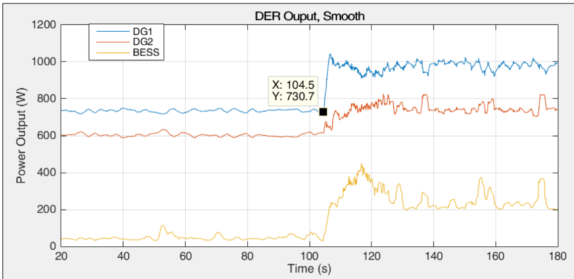
Figure 6.7.3: Experimental DER Output, Filtered
