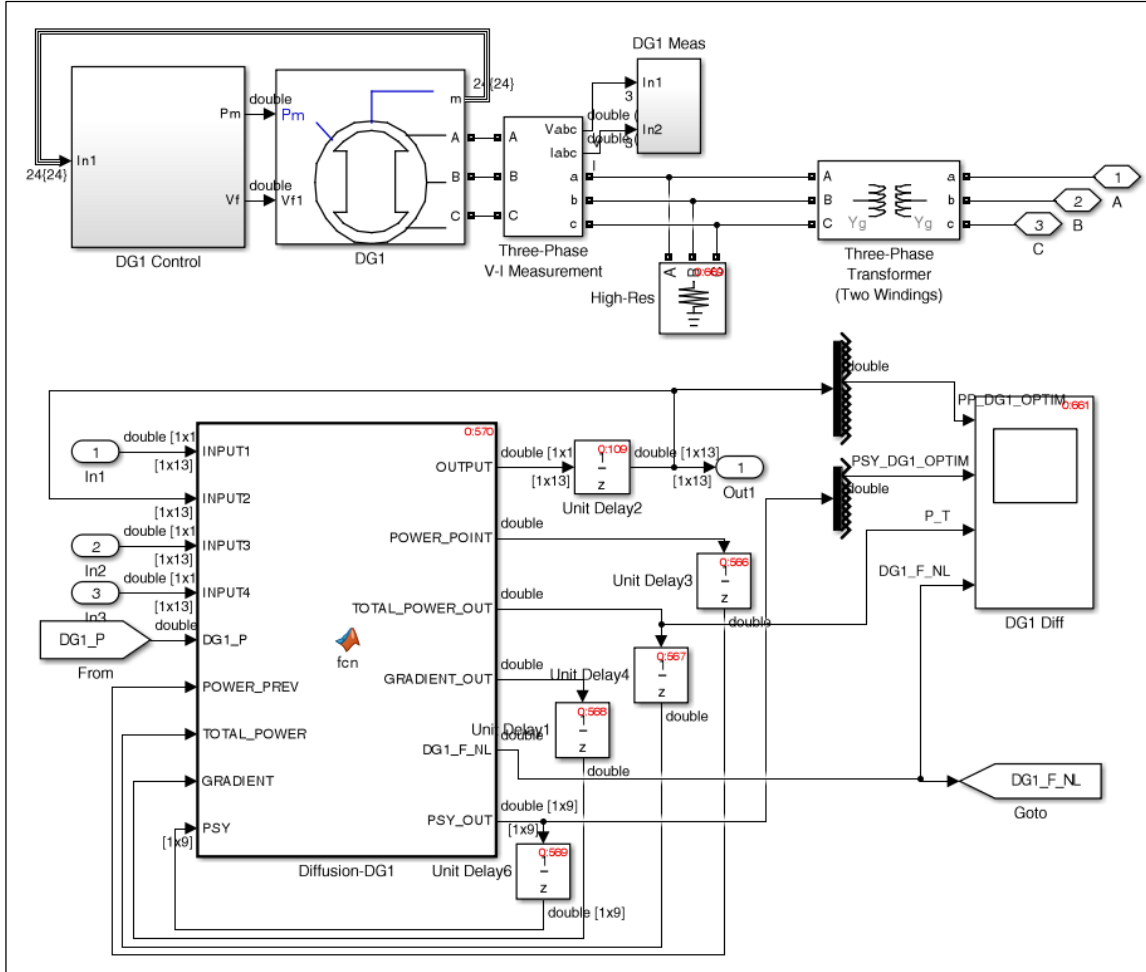
Figure 6.4.4: Simulink DG Subsystem
