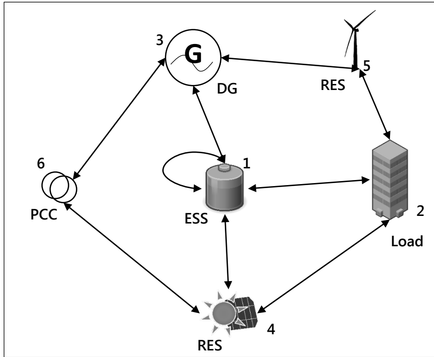
Figure 5.1.1: MG Network Node Layout
