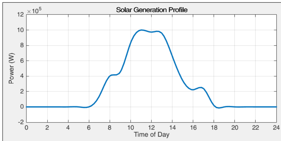
Figure 6.4.13: Solar PV Generation Profile for the city of Key Biscayne (3/20/2009)
