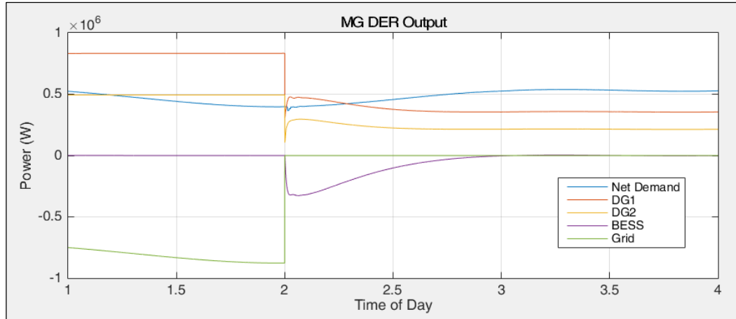
Figure 6.5.14: MG DER Output, Islanding
