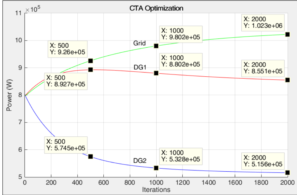
Figure 5.4.8: Grid-Connected MG CTA Diffusion, \mu = 1e8
