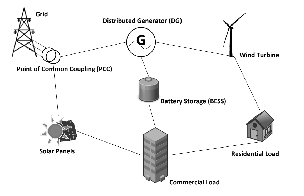
Figure 2.3.1: Hypothetical 7-Node Microgrid
