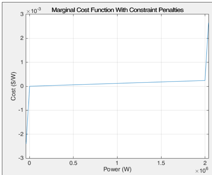
Figure 5.4.11: Fossil Fuel Generator Marginal Cost Function with Constraint Penalties
