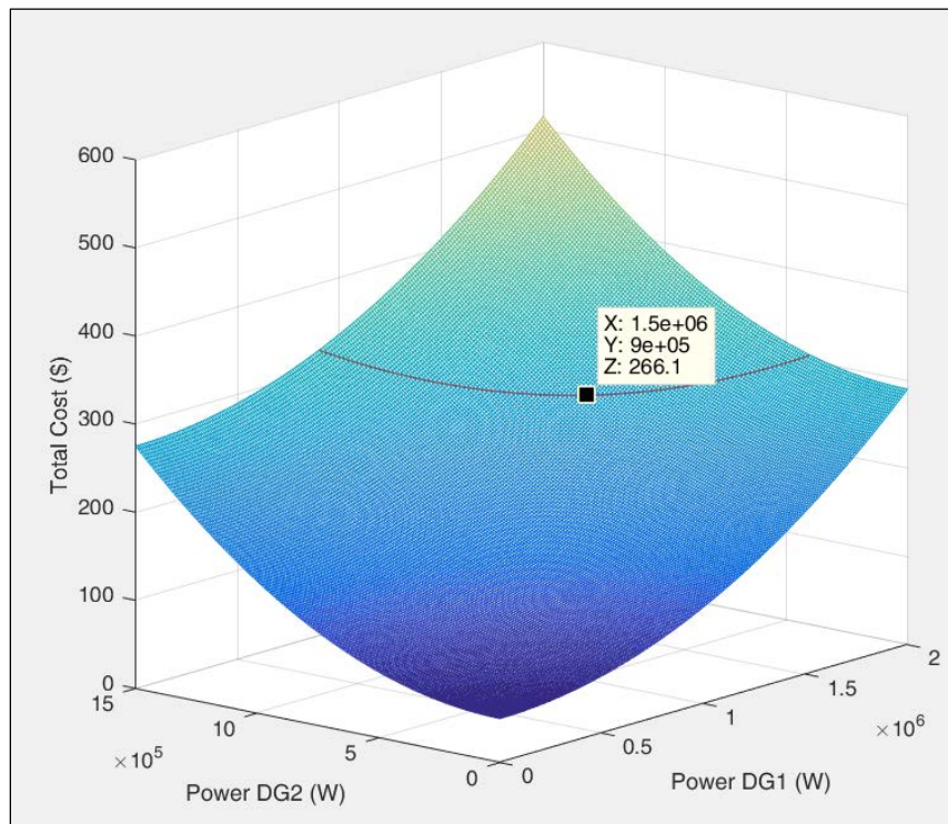
Figure 5.4.3: Islanded MG Cost Functions ED
