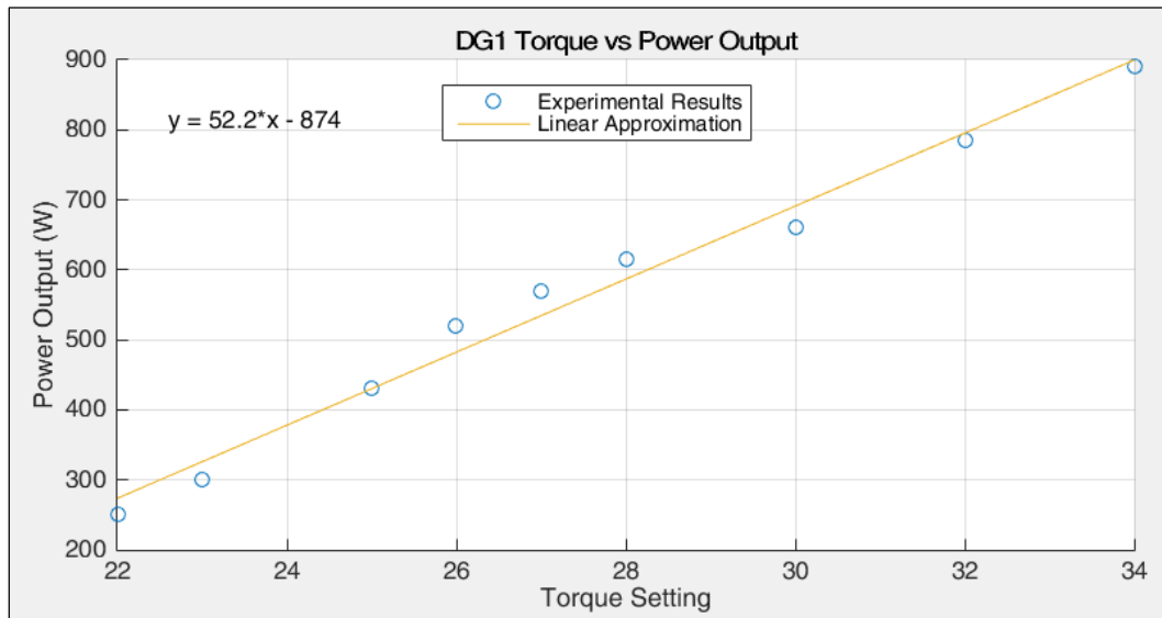
Figure 6.6.4: DG1 Torque vs Power Output
