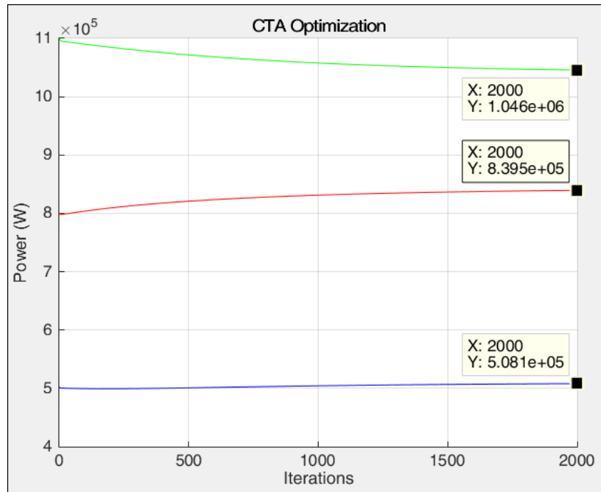
Figure 5.4.9: Grid-Connected MG CTA Diffusion, \mu = 1e8
