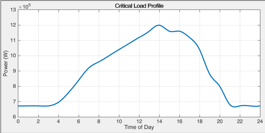
Figure 6.4.9: Critical Load Profile
