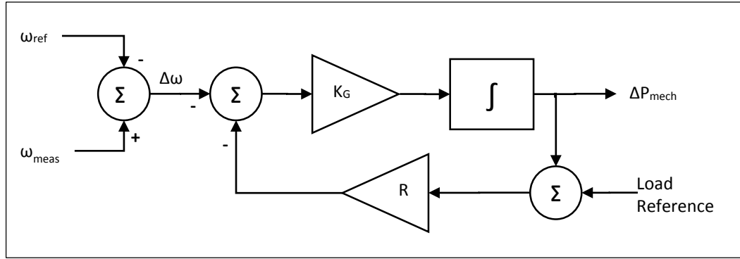
Figure 3.3.4: Droop Control
