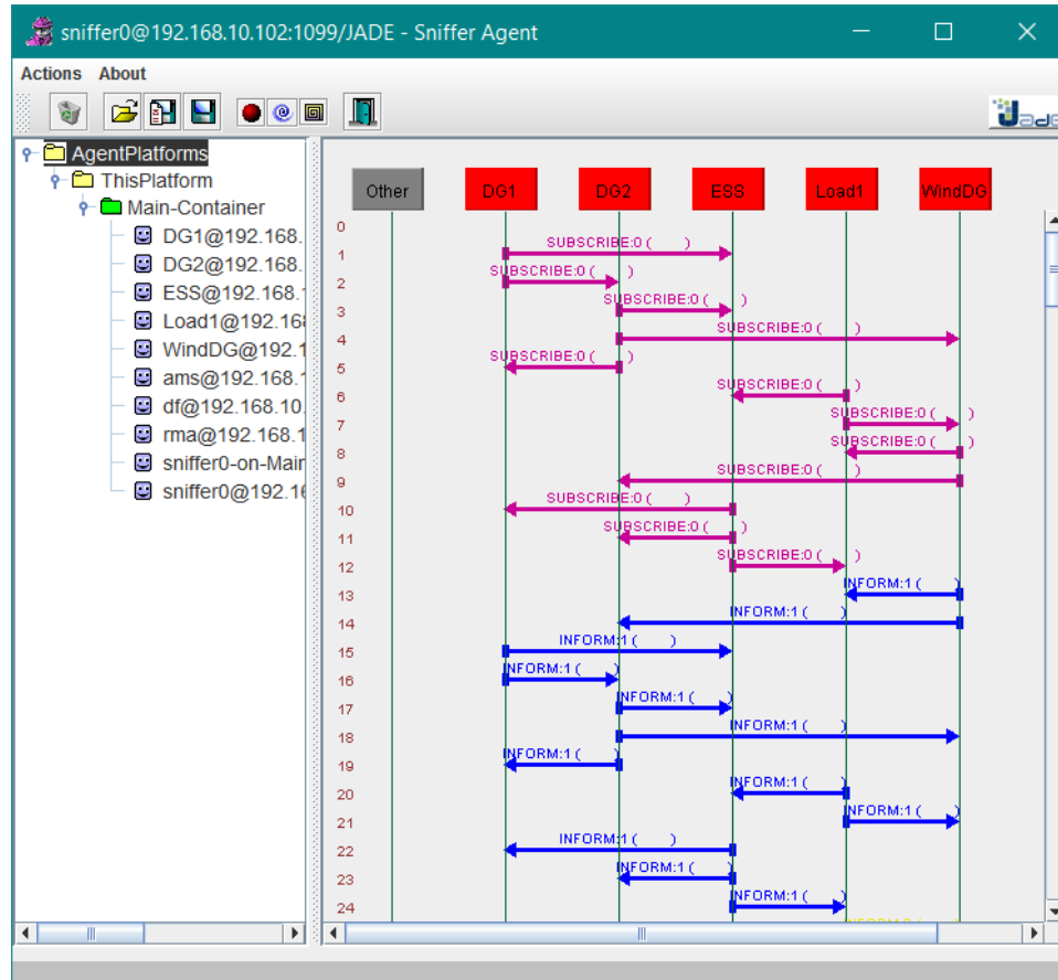
Figure 6.3.3: JADE Sniffer, Initial SUBSCRIBE and INFORM messages
