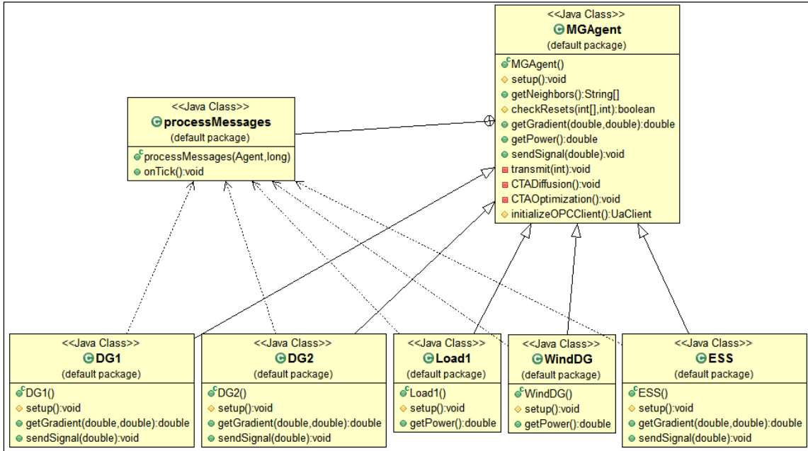
Figure 6.3.1: Multi-Agent System Java Implementation using JADE
