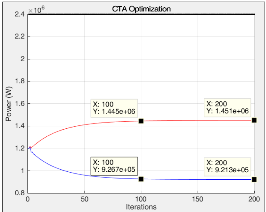
Figure 5.4.7: Islanded MG CTA Diffusion, \mu = 8e8
