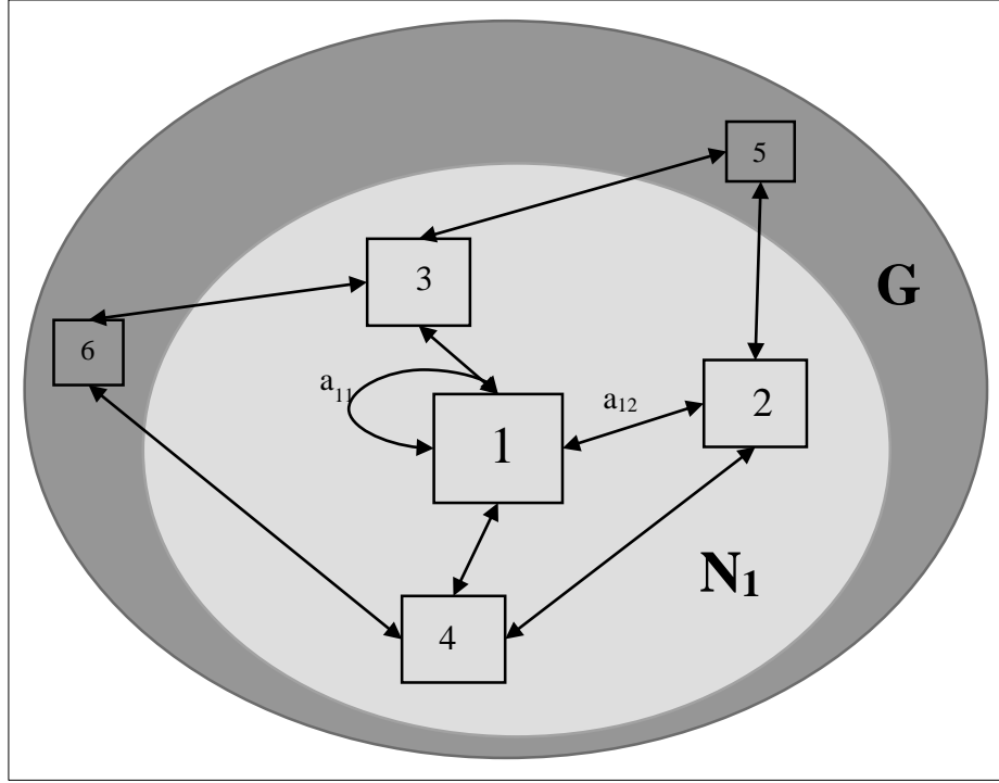
Figure 4.2.1: Graph Example
