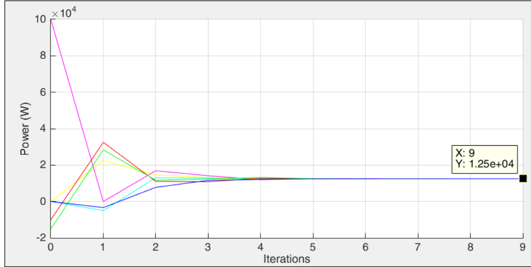
Figure 5.2.1: Diffusion Convergence
