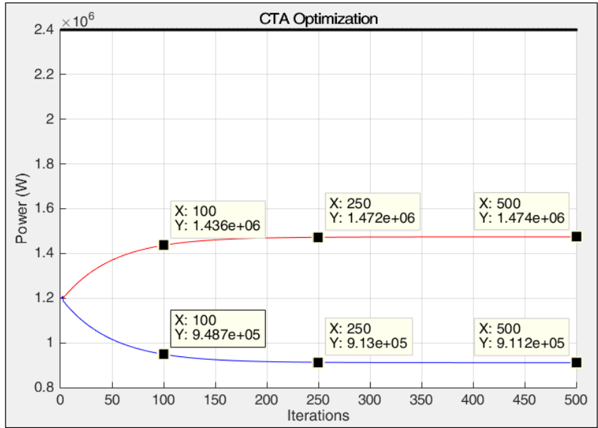
Figure 5.4.6: Islanded MG CTA Diffusion, \mu = 4e8
