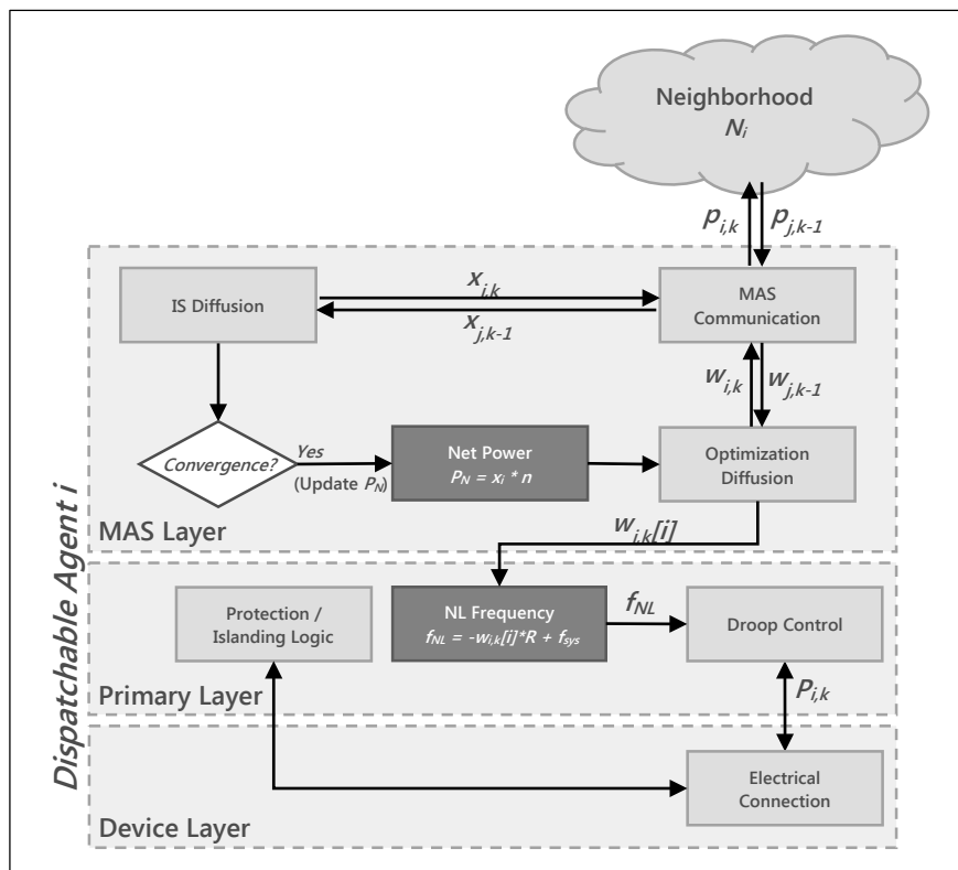
Figure 6.2.2: Dispatchable Agent Block Diagram
