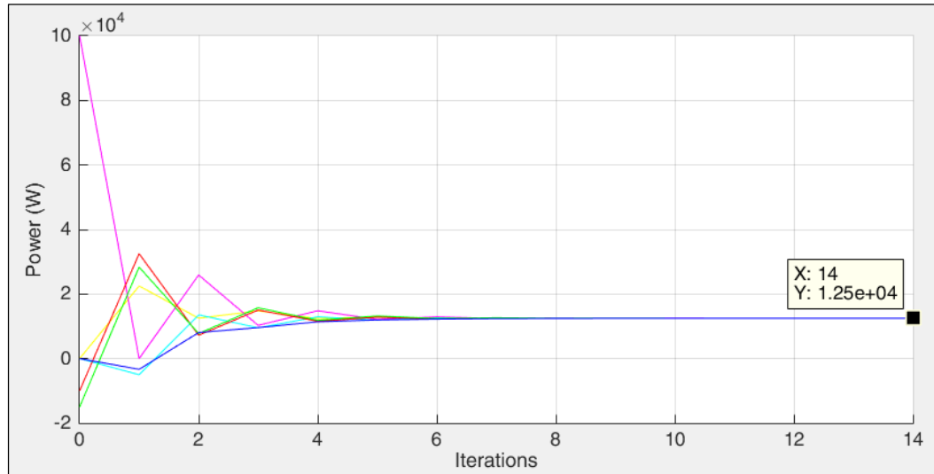
Figure 5.1.2: Consensus Convergence
