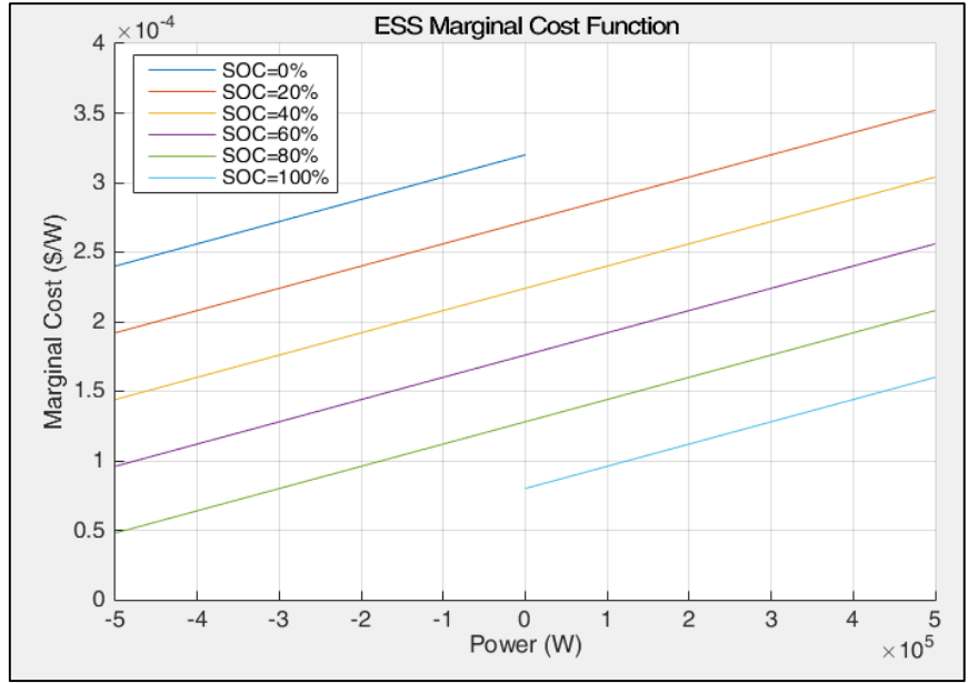
Figure 4.3.2: Energy Storage System Marginal Cost Function
