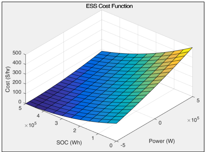
Figure 4.3.3: Energy Storage System Cost Function Surface
