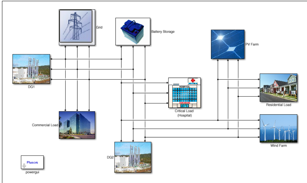
Figure 6.4.2: Simulink MG Model
