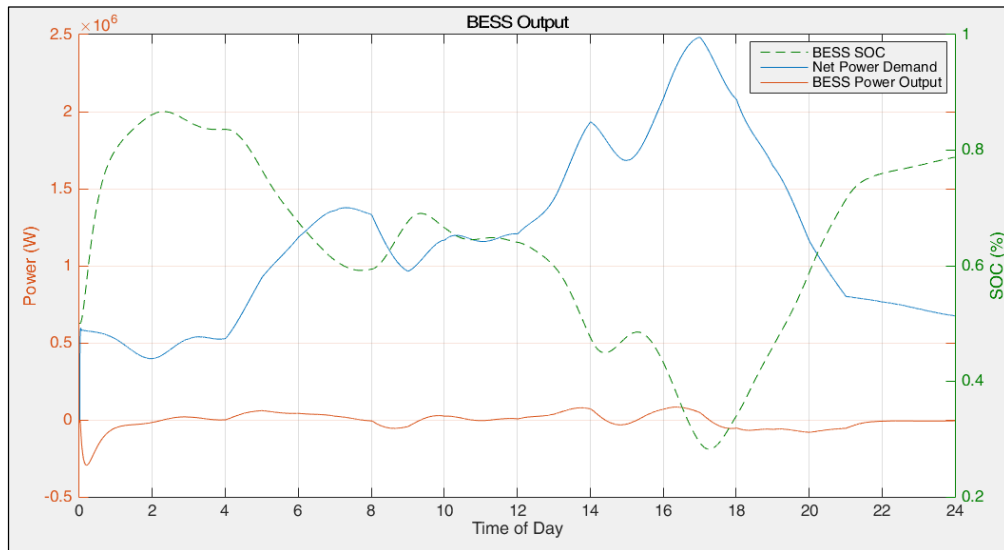
Figure 6.5.6: BESS Power Output vs SOC, Islanded
