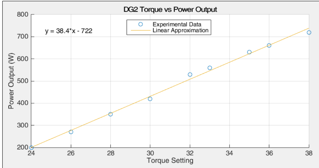
Figure 6.6.5: DG2 Torque vs Power Output
