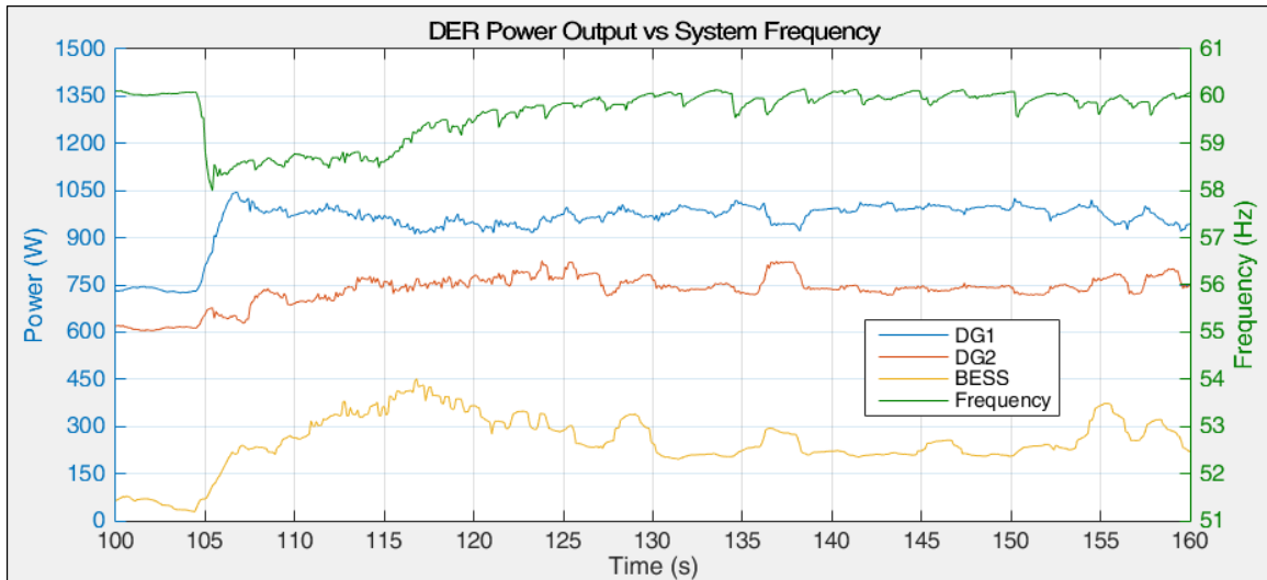
Figure 6.7.5: Experimental DER Output vs Frequency, Zoom-Out
