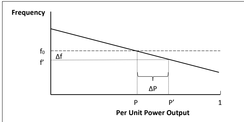
Figure 3.3.2: Speed-Droop Characteristic
