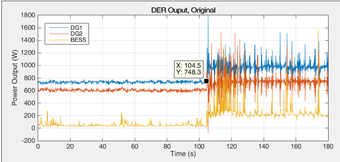
Figure 6.7.2: Experimental DER Output, Original
