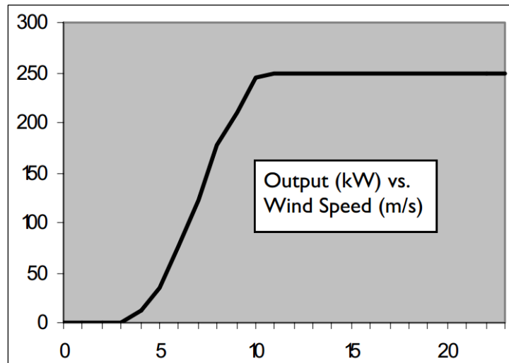
Figure 6.4.11: Inerjy EcoVert 250 Output Power vs Windspeed [40]
