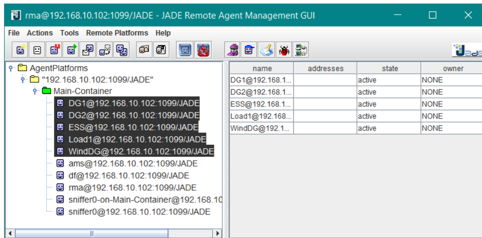
Figure 6.3.2: JADE Graphical User Interface
