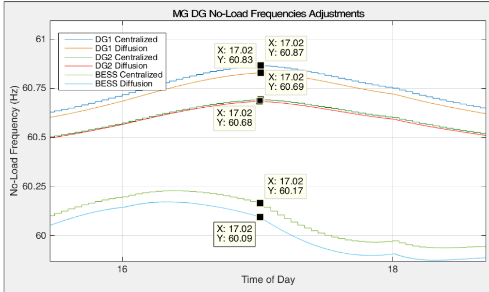
Figure 6.5.5: DG No-Load Frequency Adjustments, Islanded, Close-up
