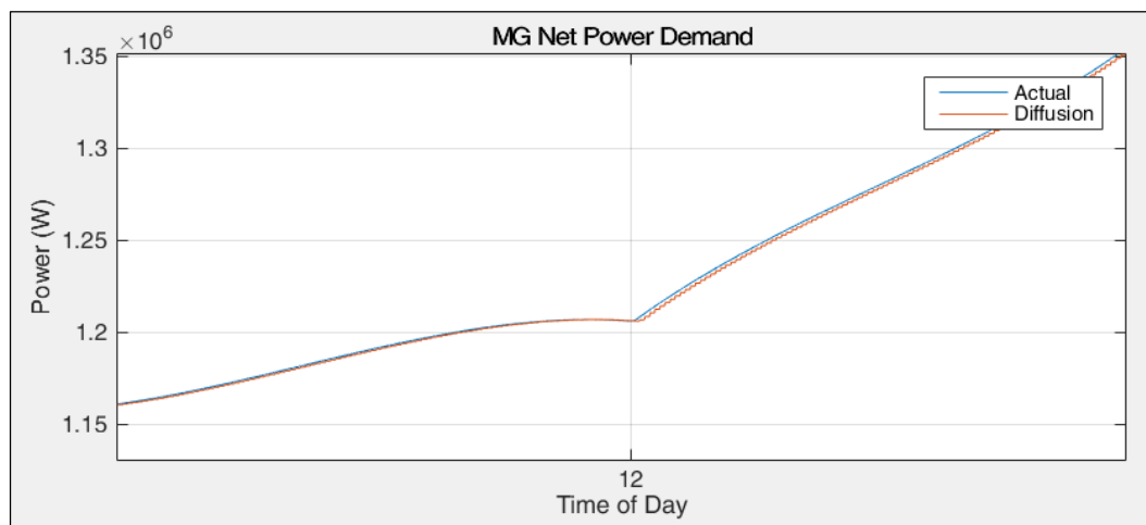
Figure 6.5.2: MG Net Power Demand, Actual vs Diffusion, Close-up
