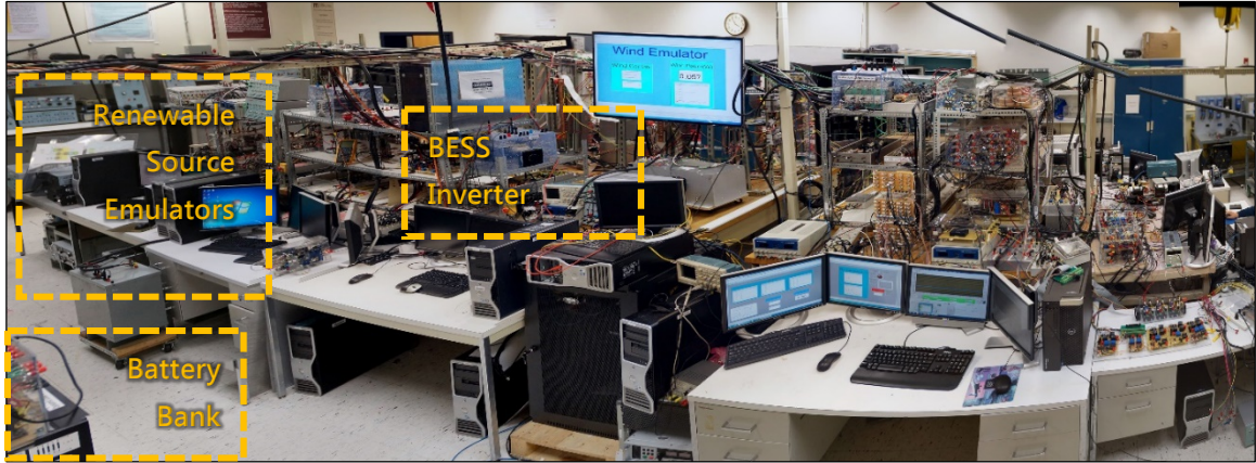
Figure 6.6.2: Smart Grid Testbed, Direct Current Side
