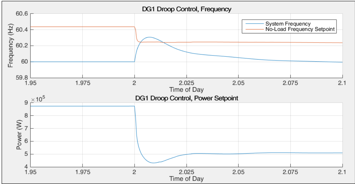
Figure 6.5.17: DG1 Droop Control, Islanding
