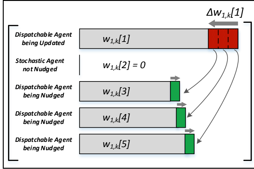
Figure 5.4.2: Nudge Methodology
