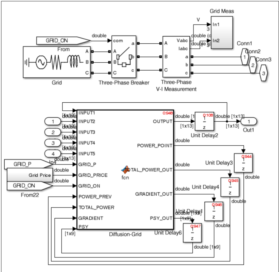
Figure 6.4.3: Simulink Grid Subsystem
