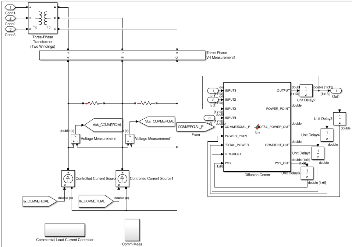
Figure 6.4.7: Simulink Stochastic Subsystem
