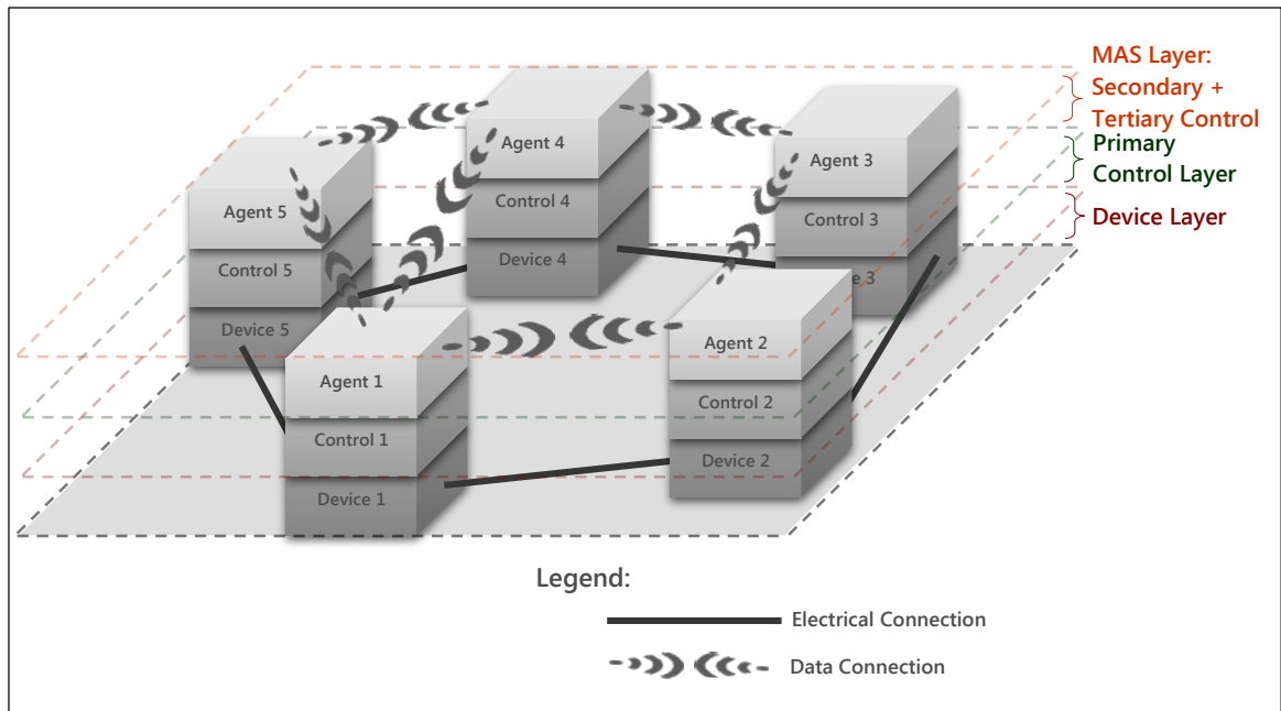
Figure 6.1.1: Control System Framework
