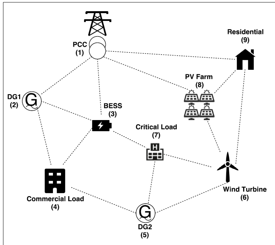
Figure 6.4.1: Hypothetical MG for Simulation
