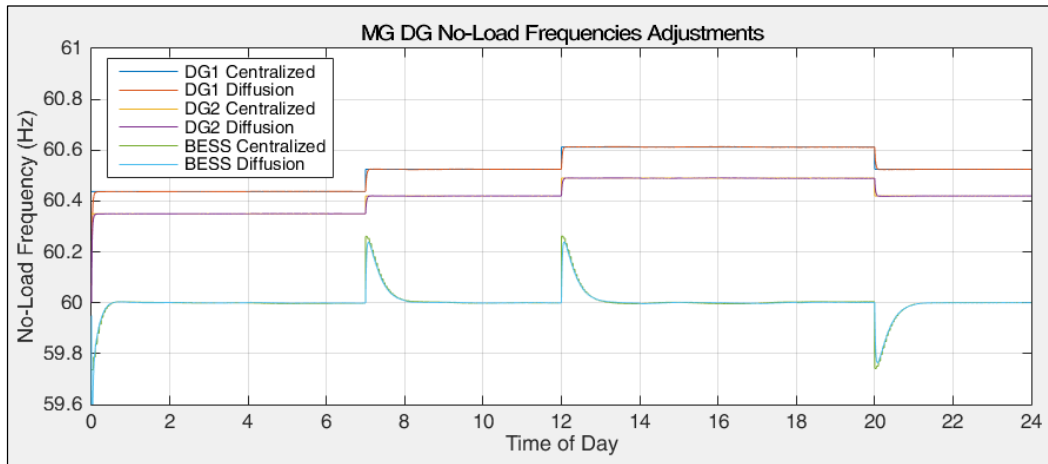
Figure 6.5.10: DER No-Load Frequency Adjustments, Grid-Connected
