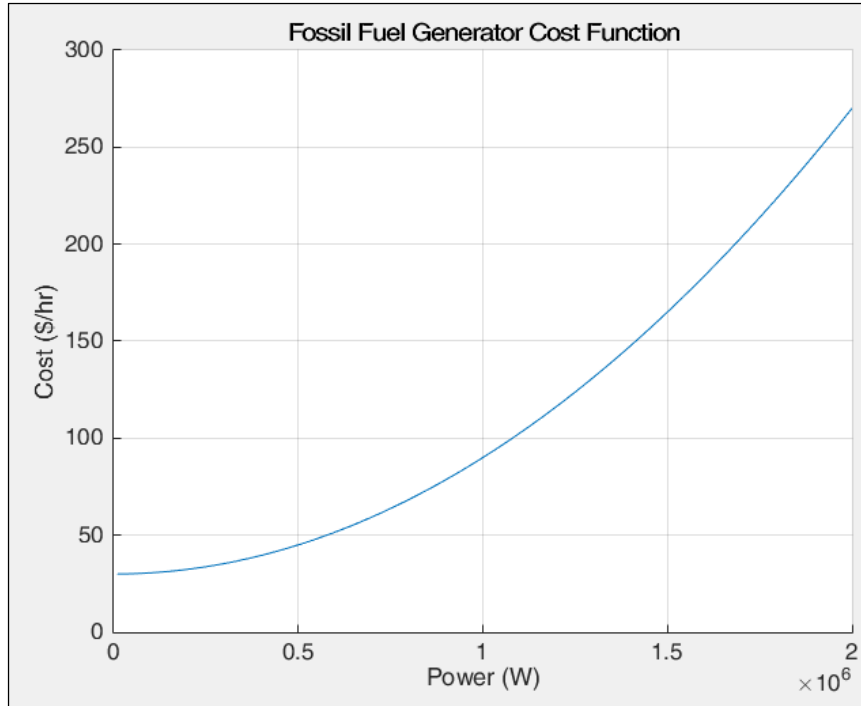
Figure 3.1.1: Typical Fossil Fuel Generator Cost Function
