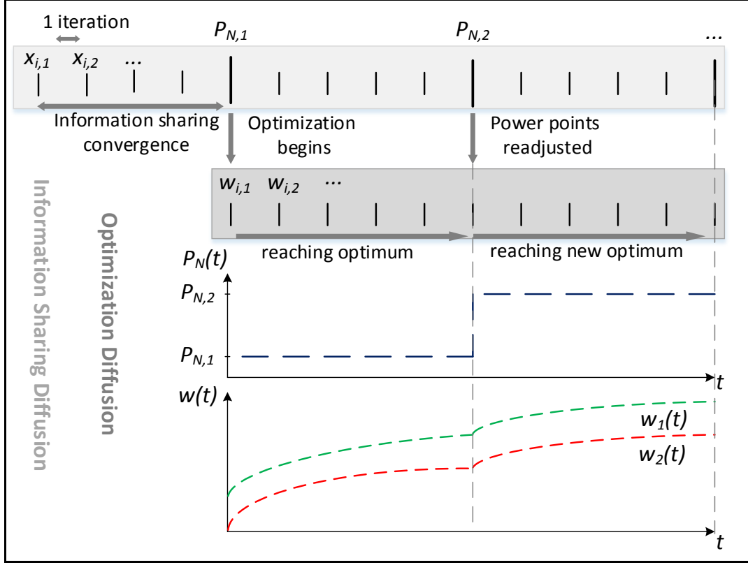
Figure 5.4.1: Two-Step Diffusion Methodology
