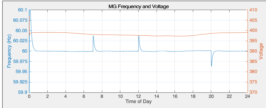
Figure 6.5.13: MG Frequency and Voltage, Grid-Connected
