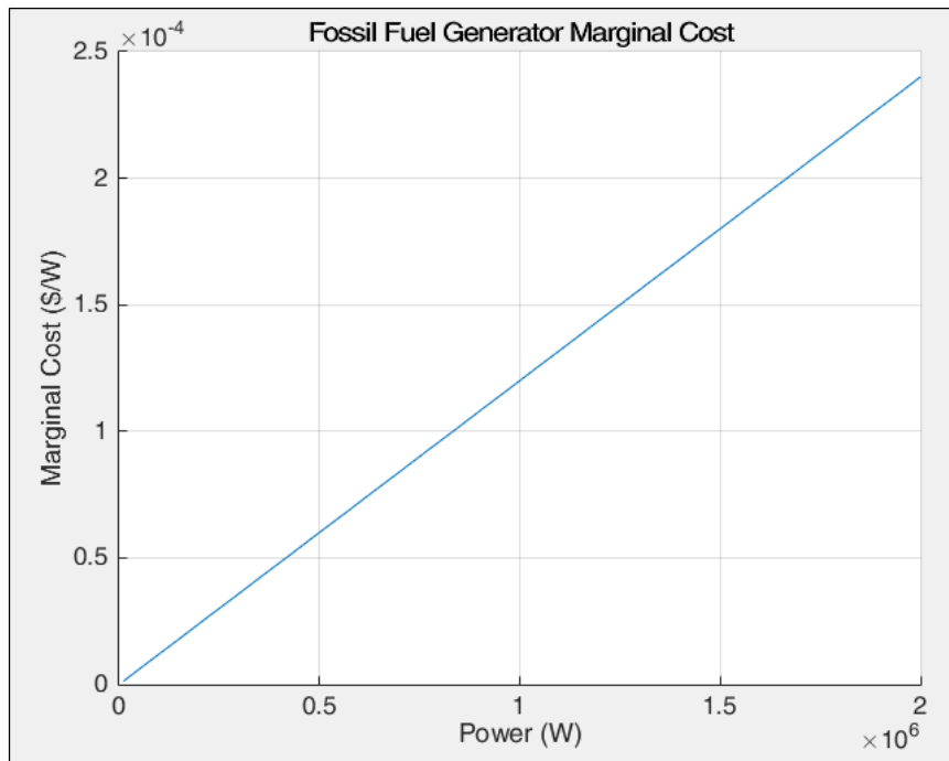
Figure 3.1.2 Typical Fossil Fuel Marginal Cost Function
