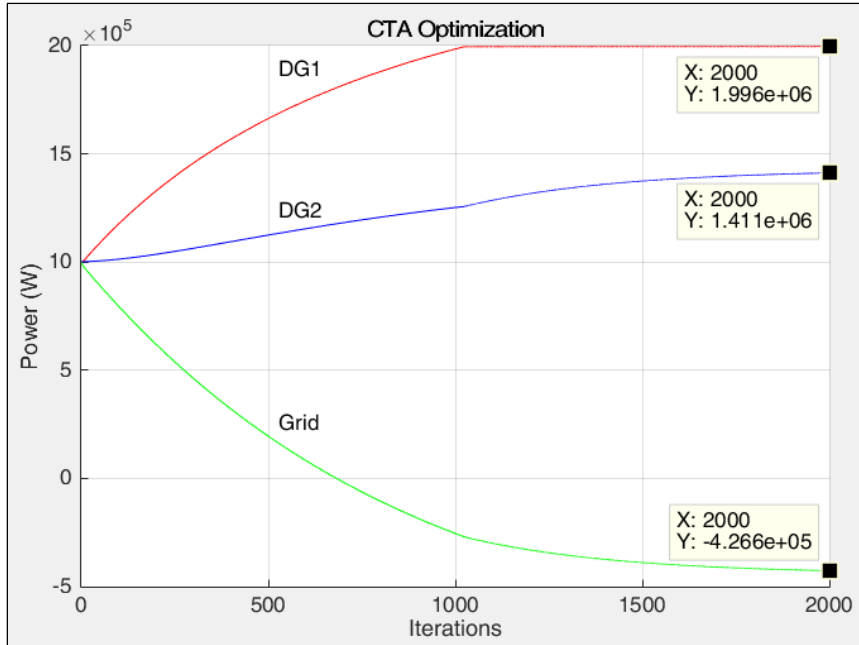
Figure 5.4.12: Grid-Connected MG CTA Diffusion w/Constraints, \mu = 1e8
