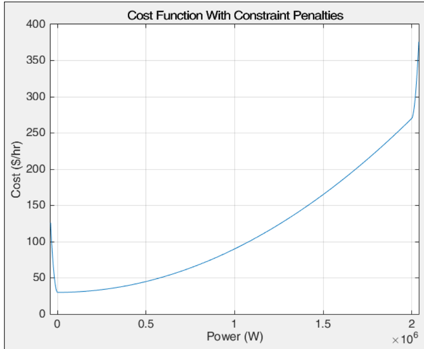
Figure 5.4.10: Fossil Fuel Generator Cost Function with Constraint Penalties
