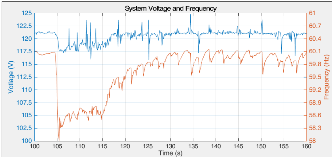
Figure 6.7.6: Experimental System Voltage and Frequency
