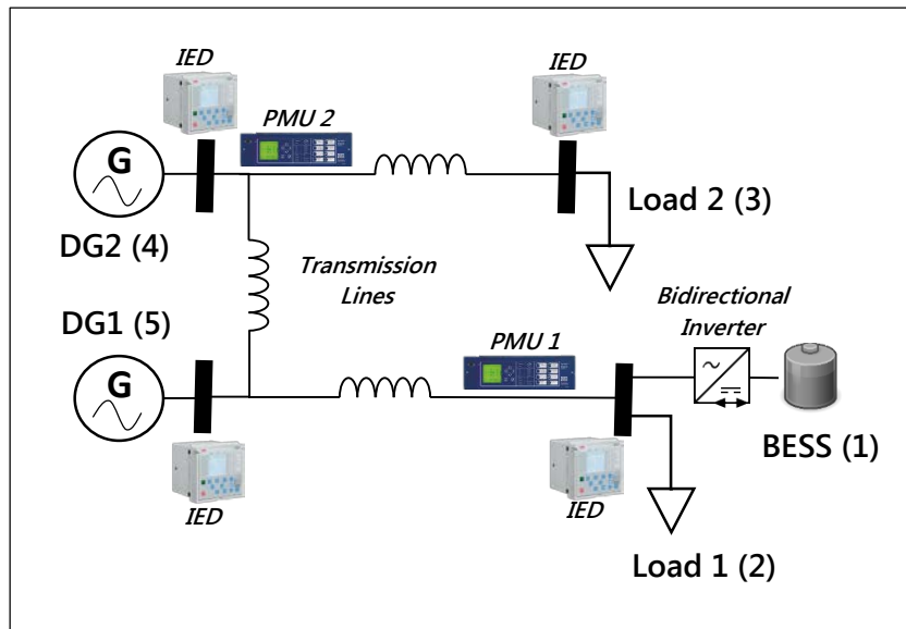
Figure 6.6.3: Experimental MG Physical Layout
