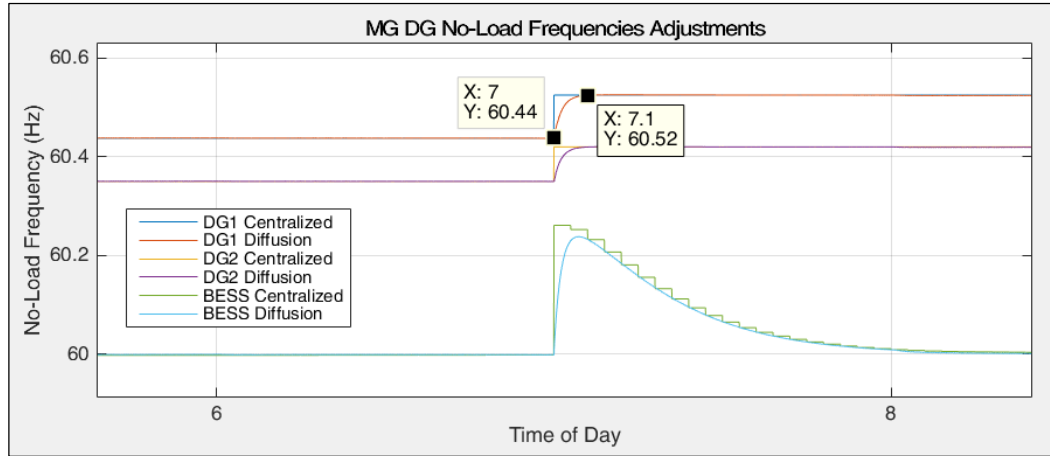
Figure 6.5.11: DER No-Load Frequency Adjustments, Grid-Connected, Close-Up
