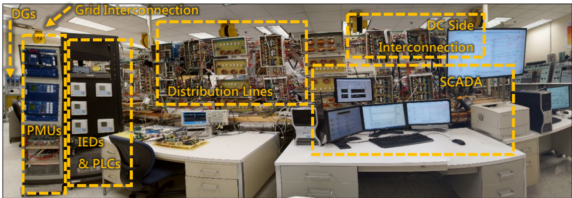
Figure 6.6.1: Smart Grid Testbed, Alternating Current Side
