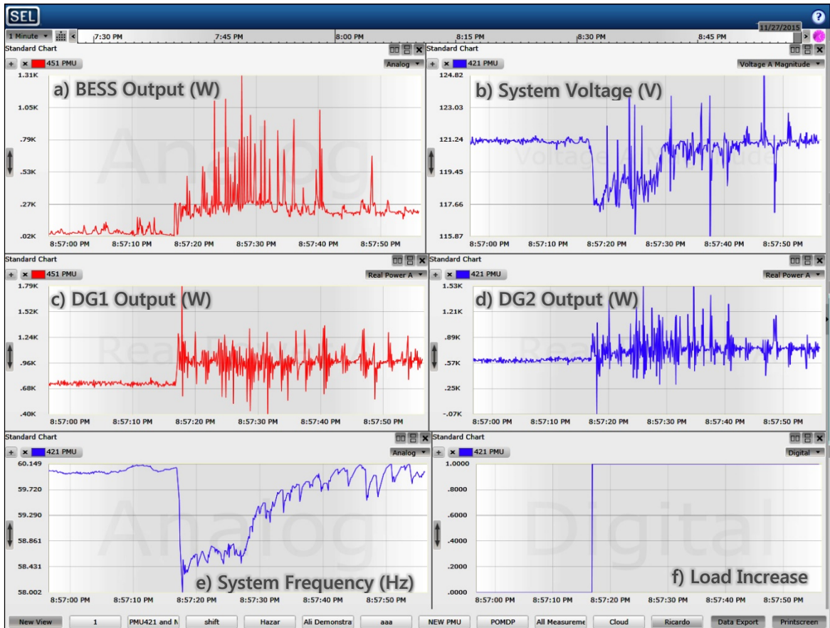
Figure 6.7.1: PMU Experimental Output
