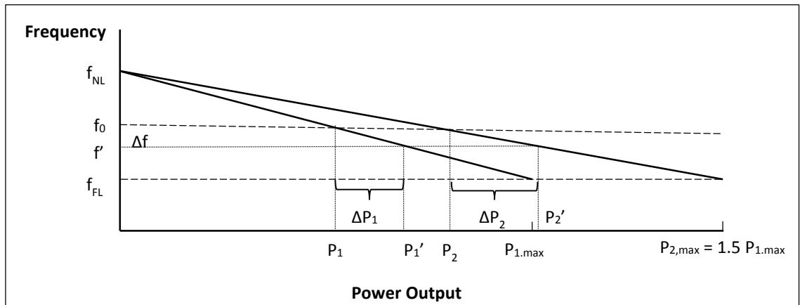
Figure 3.3.3: Speed-Droop Characteristic, Two Generators
