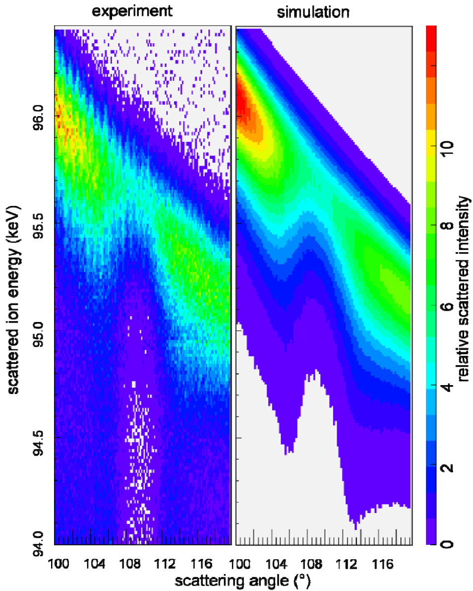
Fig. 4 Two-dimensional map of scattered ion intensities as a function of scattering angle and scattered ion energy around the [011] blocking dip (at 109.5^\circ ) for [\bar{4}11] incidence of 100 keV H^+ ions on Cu(111). The raw experimental data are compared with the theoretical simulation.
