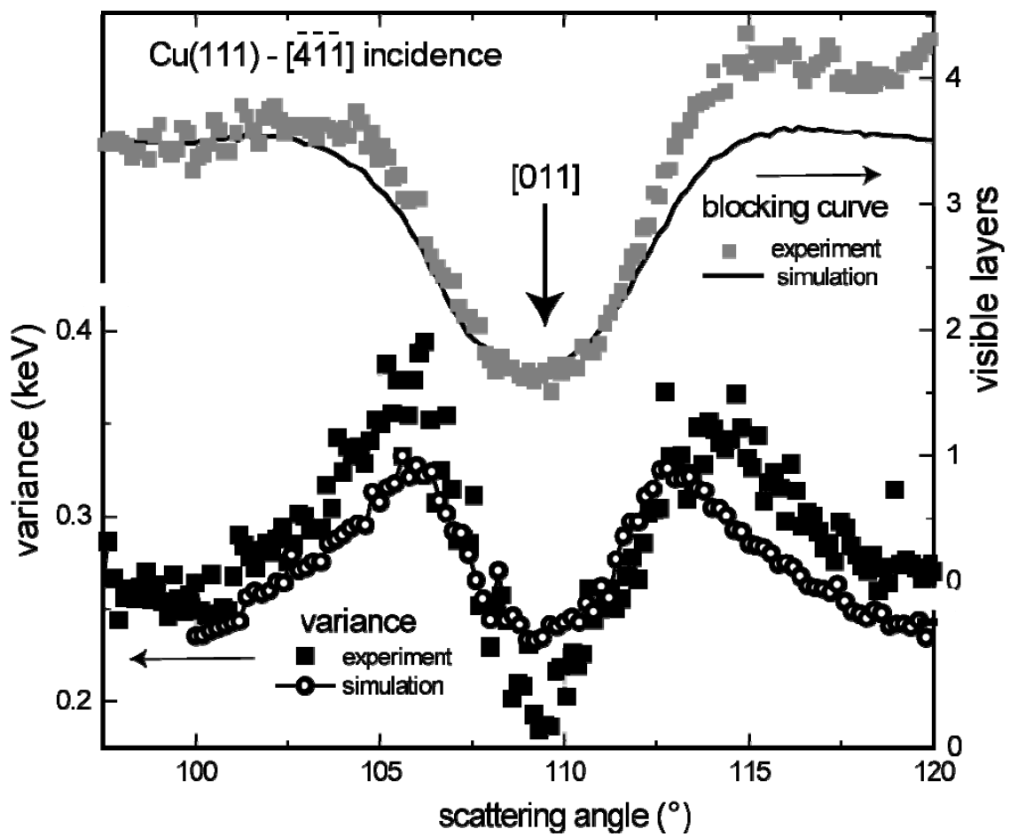
Fig. 1 Scattering angle dependence of the scattered ion intensity, and the width (variance) of the peak in the scattered ion energy spectrum for [\bar{4}\bar{1}\bar{1}] incidence of 100 keV H^+ ions. The blocking dip at 109.5^\circ corresponds to emission along [011] .
