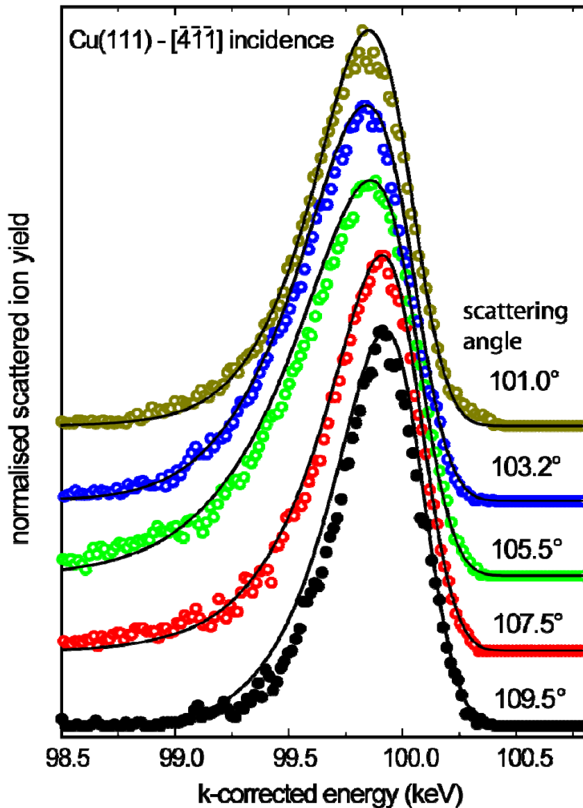
Fig. 3 Comparison of the experimental (circles) and theoretical (full line) scattered ion energy spectra for [\bar{4}\bar{1}\bar{1}] incidence of 100 keV H^+ ions on a Cu(111) surface at different scattering angles in the [\bar{2}11] azimuth. The [011] blocking direction is at 109.5^\circ . Energies have been offset by the kinematic elastic recoil energy and peak intensities are normalised to the same value to aid comparison of peak shapes and relative energies.
