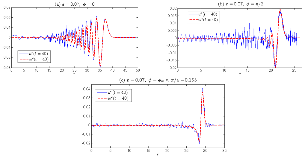
Figure 7: Solutions u^\varepsilon and w^\varepsilon for \varepsilon = 0.07 at t = 40 for the laminated geometry (4.12) along three rays: (a) \phi = 0 . (b) \phi = \pi/2 . (c) \phi = \phi_m \approx \pi/4 - 0.153 .
