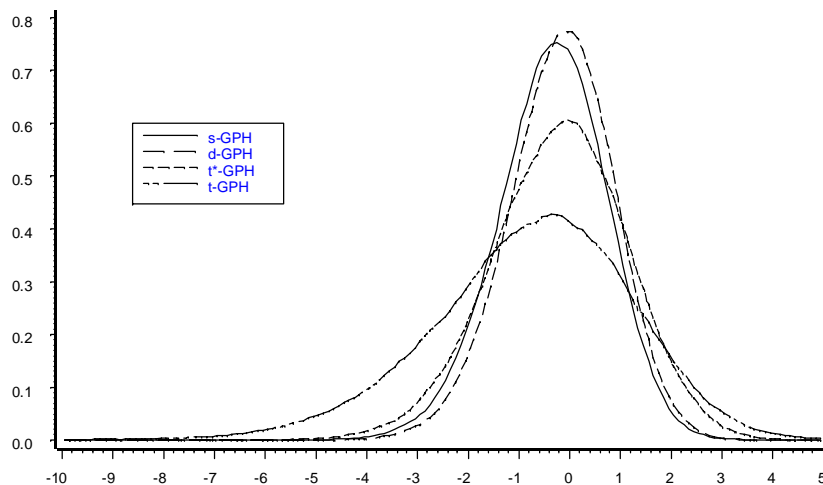
Figure 1: Estimated density of s-GPH, d-GPH, t-GPH and t*-GPH under the null hypothesis of no cointegration with T=1000 and n=T^{0.6}
