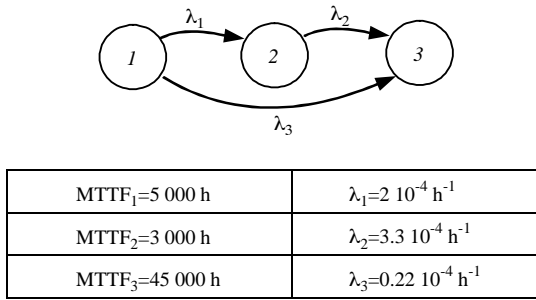
Fig. 19. T SENSOR reliability MC model.
