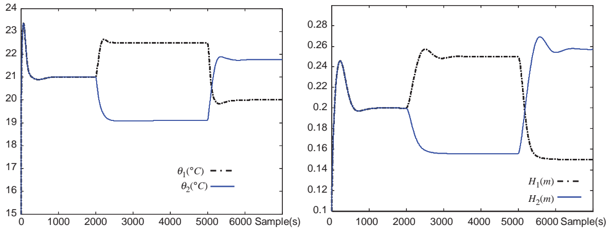
Figure 5. Dynamic evolution of local output variables in the fault-free case.
