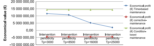
Fig. 21. Financial performances of the Sol after different maintenance strategies applied to valves.
