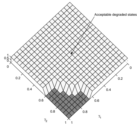
Fig. 2. Acceptable degraded states based on reliability evaluation.
