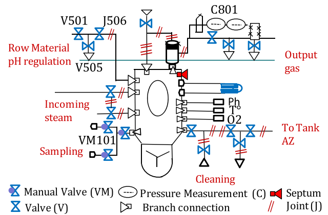
Fig. 11. Part of the production harvest system.
