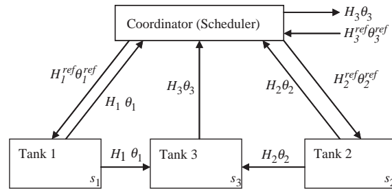
Figure 3. Physical decomposition of the heating system.
