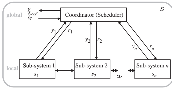
Figure 1. General scheme of hierarchical structure.
