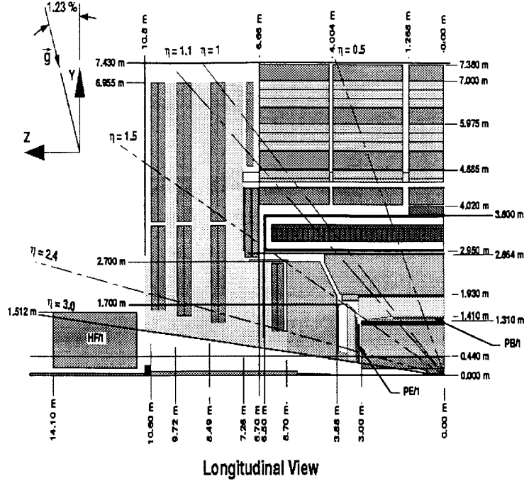
Figure 1: Longitudinal view of CMS detector.
