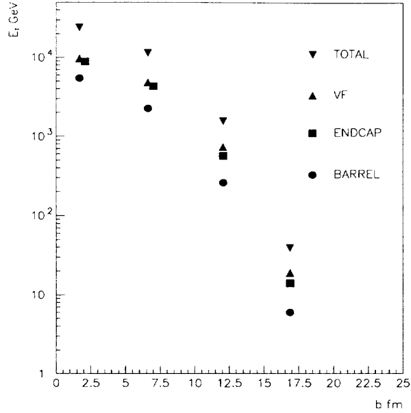
Figure 2: Expected dependence of the detected transverse energy on the impact parameter of Pb - Pb collisions.
