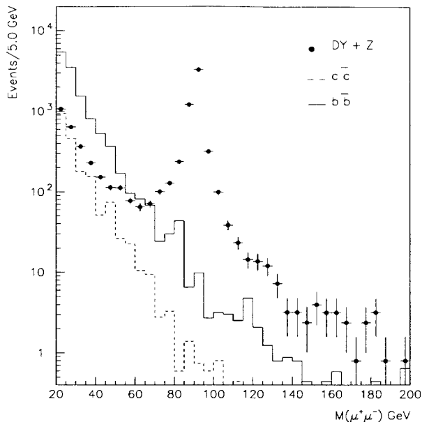
Figure 4: Invariant mass spectra of \mu^+\mu^- pairs for muons with P_T > 5 GeV/c.
