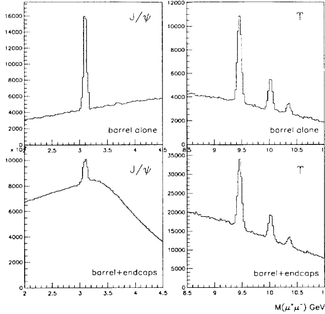
Figure 3: Dimuon mass spectra for J/\psi and \Upsilon mass regions in different parts of detector.
