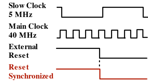
Figure 12: Chronogram of reset activation
