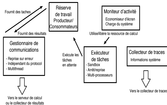
FIG. 4. Architecture du Worker
