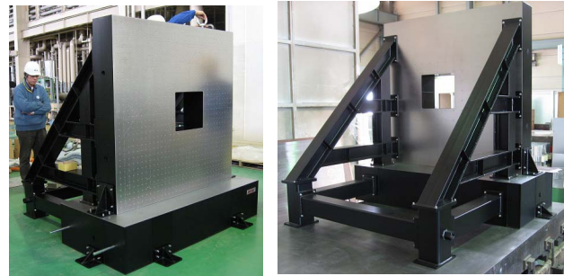
Figure 3: Vertical table with a horizontal table and bars for supporting them. They are views from the mount side (left) and the back side (right). The square hole on center is for mounting the vacuum chamber.
