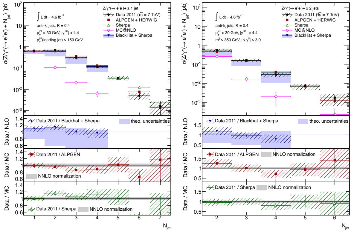
(c) p_{\text{T}}(\text{leading jet}) > 150 GeV
