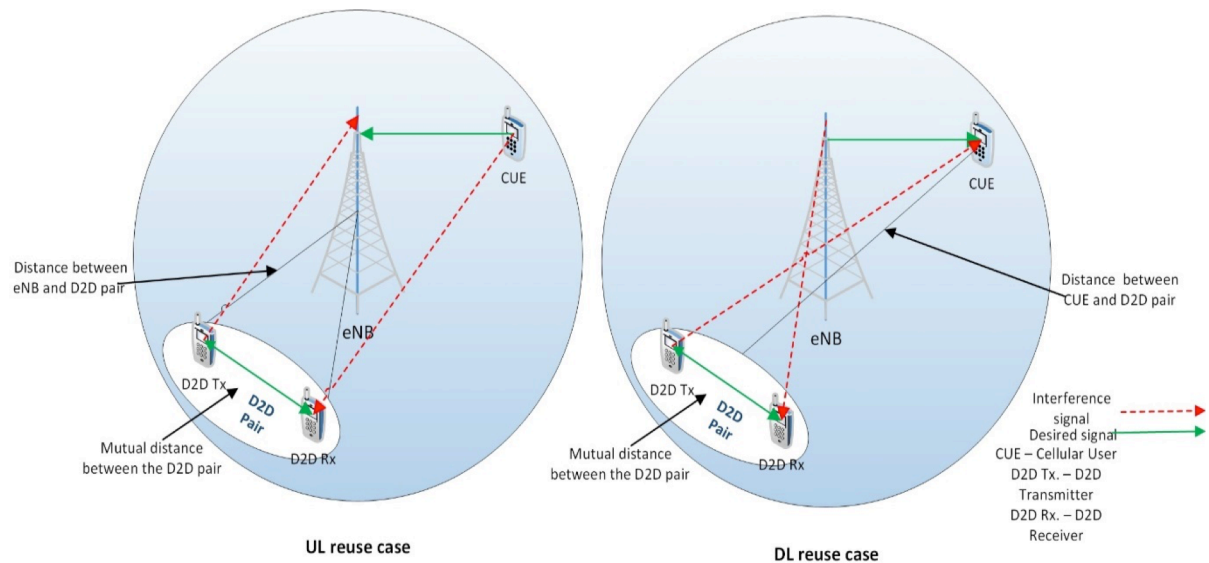
Fig. 11. D2D Power control model.
