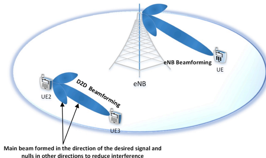
Fig. 12. Schematic representation of beamforming with eNB and D2D users equipped with multiple antenna elements.
