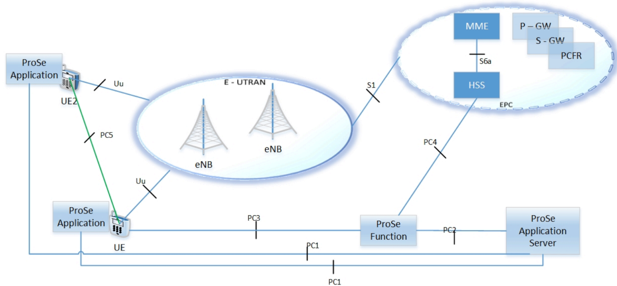
Fig. 8. Schematic representation of D2D enhanced LTE architecture.
