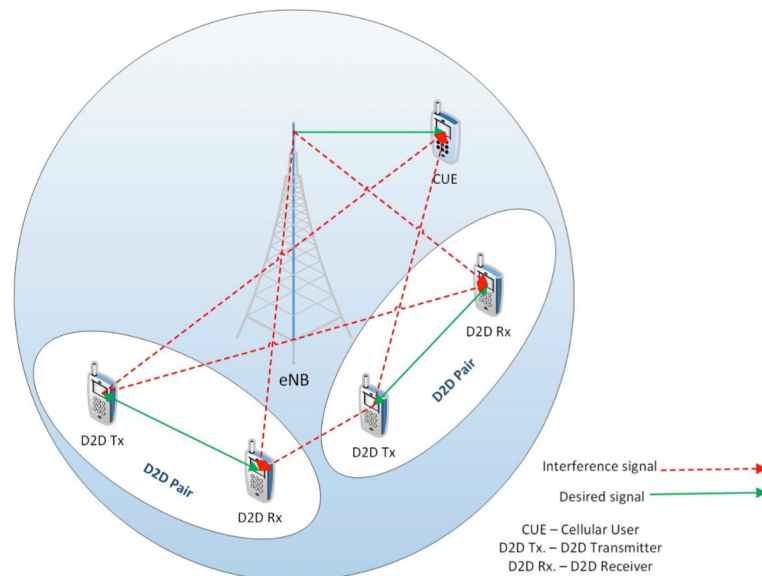
Fig. 10. Interference scenario of D2D and cellular links under downlink resource reuse.
