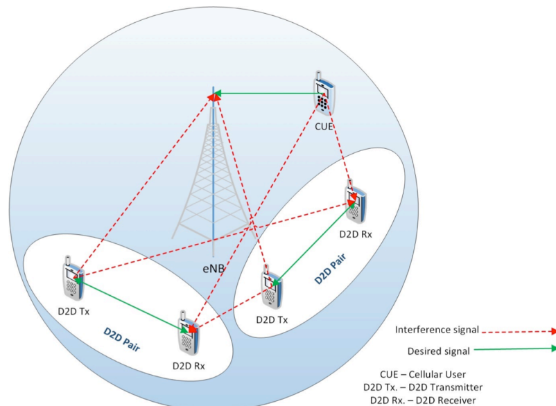
Fig. 9. Interference scenario of D2D and cellular links under uplink resource reuse.
