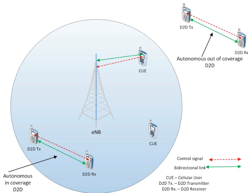
Fig. 7. Device – controlled discovery and session setup procedures.
