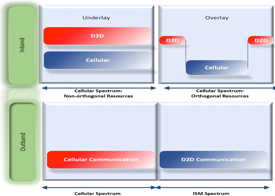
Fig. 5. Schematic frequency band occupancy of D2D communication in cellular networks.
