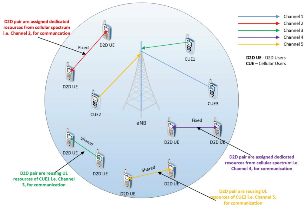
Fig. 4. A single cell comprising of multiple cellular links, and D2D links using different D2D communication modes.
