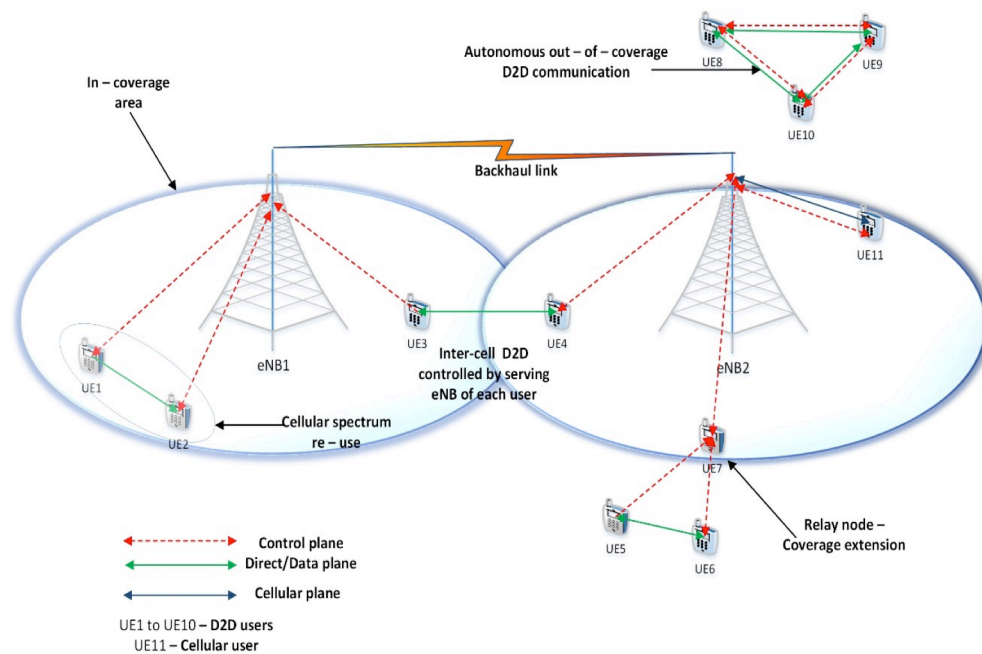
Fig. 2. Illustration of D2D-enabled cellular network concepts and use-cases.
