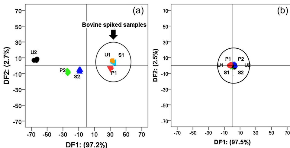
Fig. 6. Discriminant function plots showing a clear discrimination of all proteins as unique protein clusters for both MIP modified GCE (a) and non-imprint control NIPs (b). Surine™ (U), plasma (P) and serum (S) samples spiked with a mixture of all three proteins (Bhb, HHb, PHb; 100 \mu\text{g mL}^{-1} each, are noted as U1, P1 and S1 respectively); Samples spiked with a mixture in the absence of the original BHb template (HHb, PHb; 100 \mu\text{g mL}^{-1} each, are noted as U2, P2 and S2 respectively). For demonstrative purposes, Both MIP and NIP plots were kept at the same scale to illustrate the profiling pattern recognition effect.
