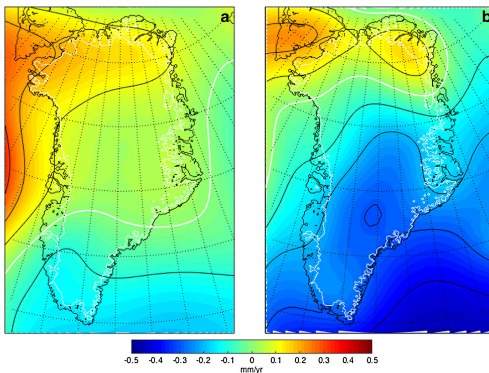
Fig. 4 Comparison of present rates of GIA-related geoid height variation in Greenland calculated using the deglacial chronology and viscoelastic Earth structure of [24] (Huy3), a , and b the ICE-6G_C (VM5a) global deglacial history and Earth model VM5a [25, 70]. White lines on the plots denote the zero contour between areas of geoid uplift (subsurface mass input) and subsidence (subsurface mass output). Geoid height trends are contoured every 0.1 mm/year
