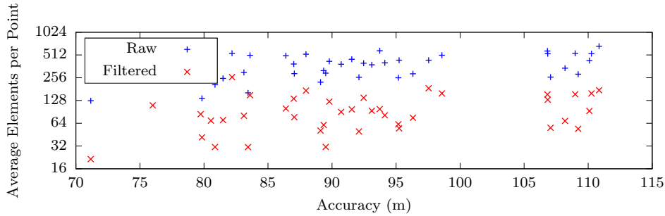
Figure 10: Effect of accuracy on number of elements, pre- and post-filtering, for different users' data.
