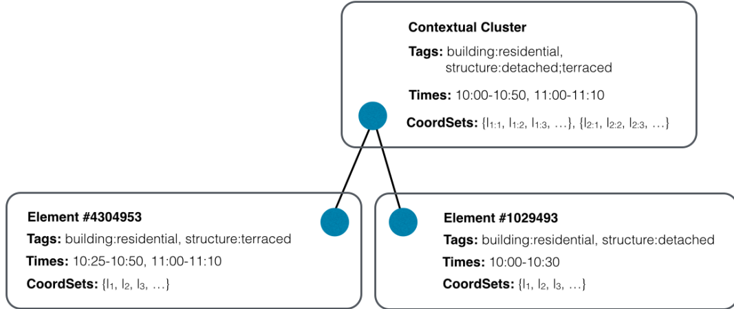
Figure 5: Cluster merging example.
