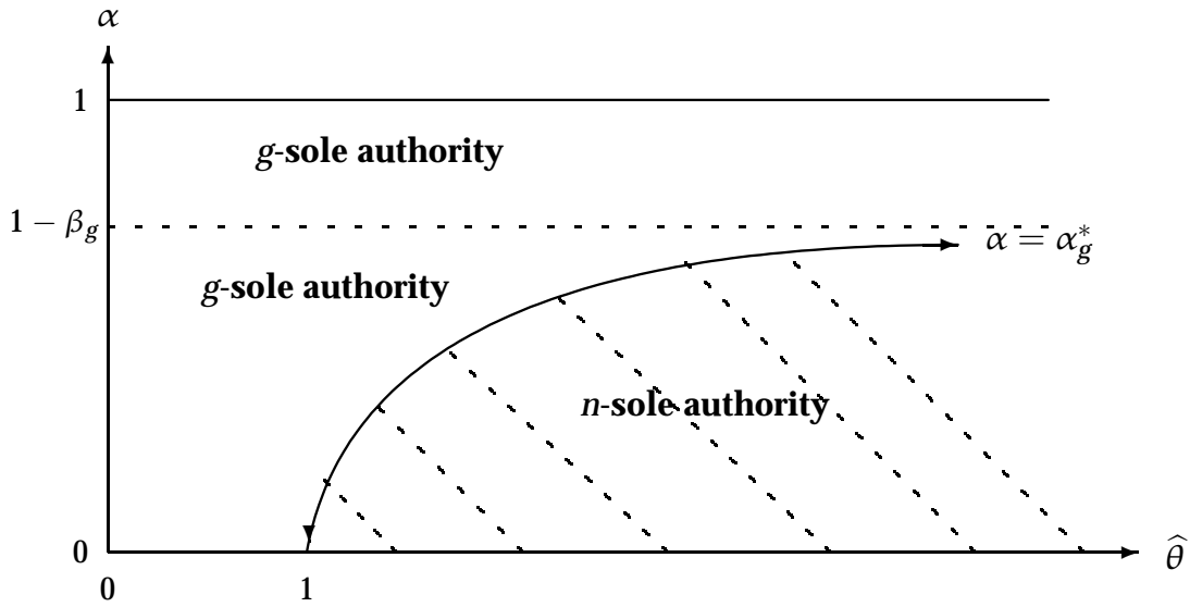
FIGURE 1. An illustration of Proposition 2.
