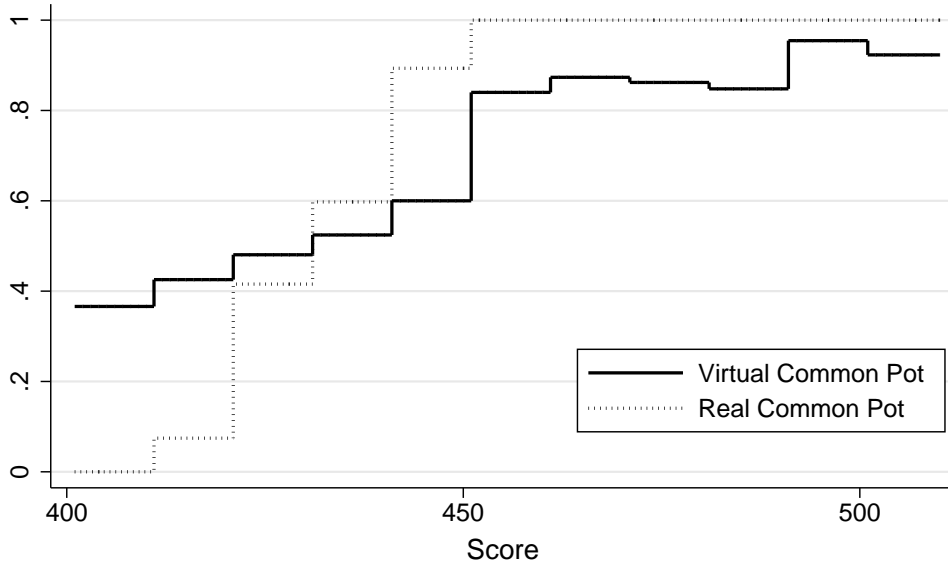
Figure 1: Treatment propensity
