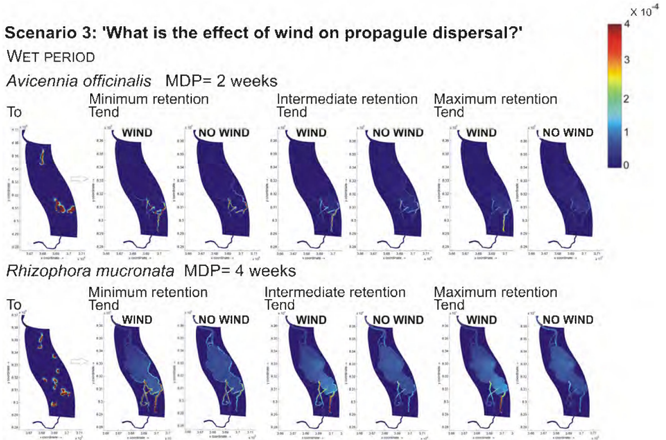
Fig. 7. Results of scenario 3 (the effect of “additional wind”) showing the distribution plots of propagules of Avicennia officinalis and Rhizophora mucronata . Scale is applicable to all distribution patterns. Red, yellow and light blue colours indicate a high, medium and low concentration of propagules respectively.
