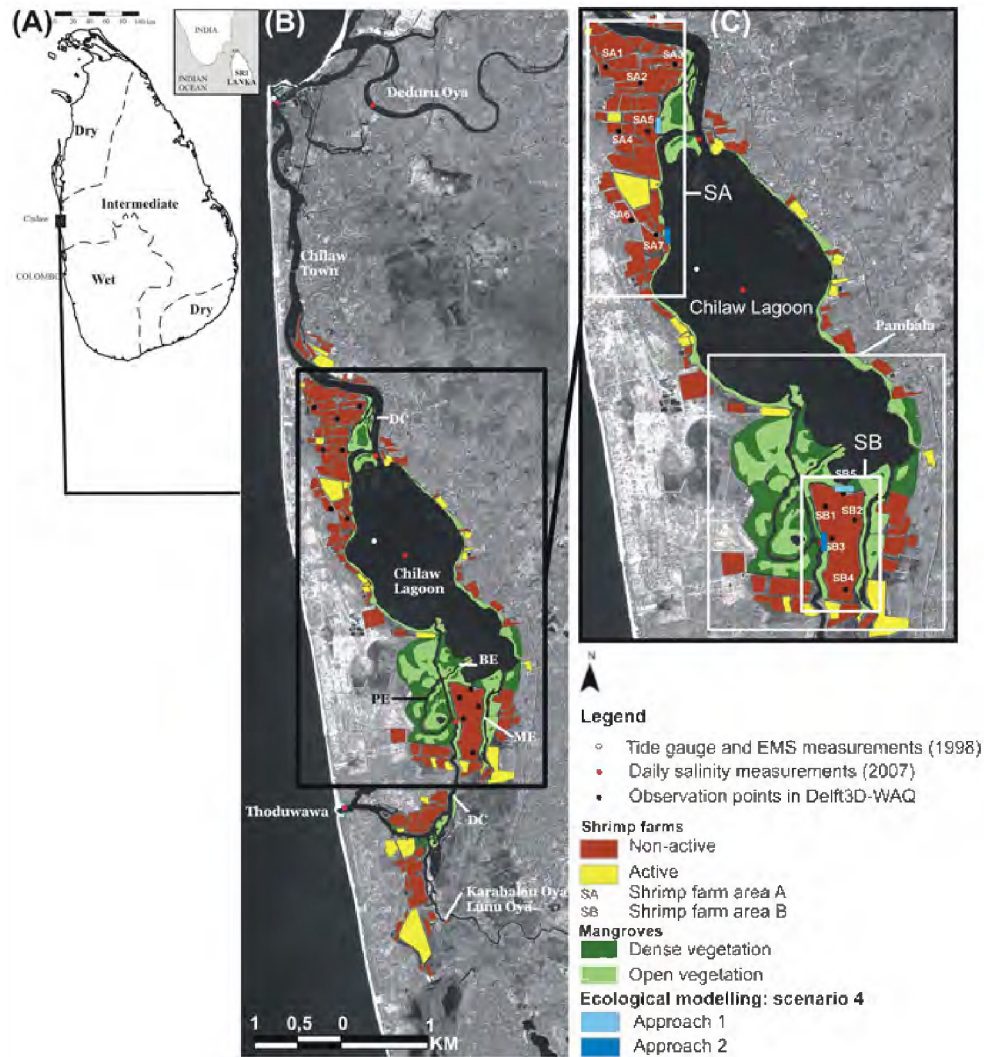
Fig. 1. (A) Representation of Sri Lanka (Daoudou-Guebas et al., 2000). (B) an IKONOS image (2002) showing the Pambala–Chilaw Lagoon Complex. (C) Indication of the water level and salinity measurements points (both in 1998 and 2007), the observation points in Delft3D-WAQ within shrimp farm area A and B, the active and non-active shrimp farms, the dense and open mangrove vegetation and the channels. Locations of outer dike removal (approach 1 and 2) are also indicated. EMS = Environmental Monitoring System. DC = Dutch Canal. PE = Pol Ela, ME = Marambettiya Ela, BE = Bate Ela.
