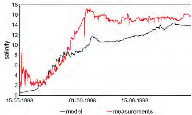
Fig. 3. Validation of the hydrodynamic model: presentation of the salinities measured in the field (red) versus the salinities generated by the model (black).
