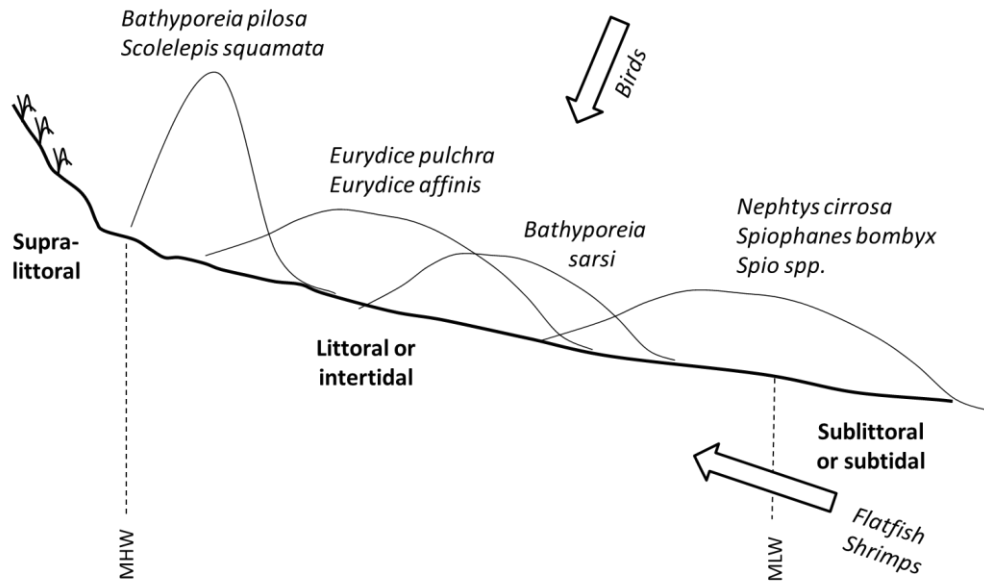
Figure 4: Zonation pattern of different Belgian macrobenthic species (adapted from Van Tomme 2013, originally adapted from Speybroeck 2007); MHW: mean high water level; MLW: mean low water level
