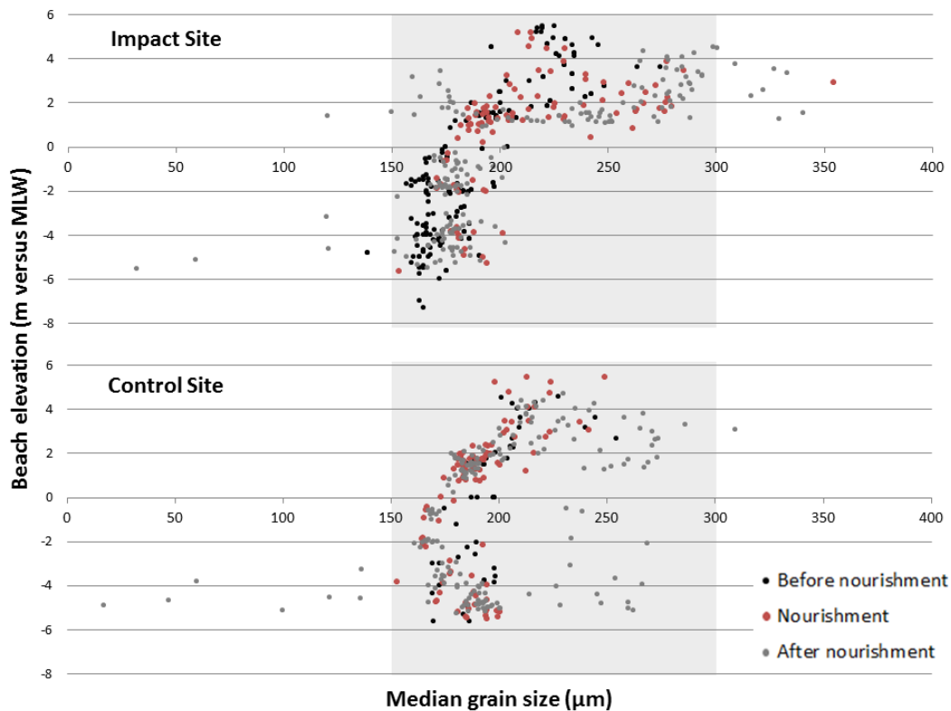
Figure 4: Beach elevation (m versus MLW) versus median grain size ( \mu\text{m} ) of the impact site (top) and the control site (bottom) before (2008; black), during (2009; red) and after the nourishment (2010, 2011 and 2012: grey); the grey area indicates the normal range of median grain size found on Belgian beaches
