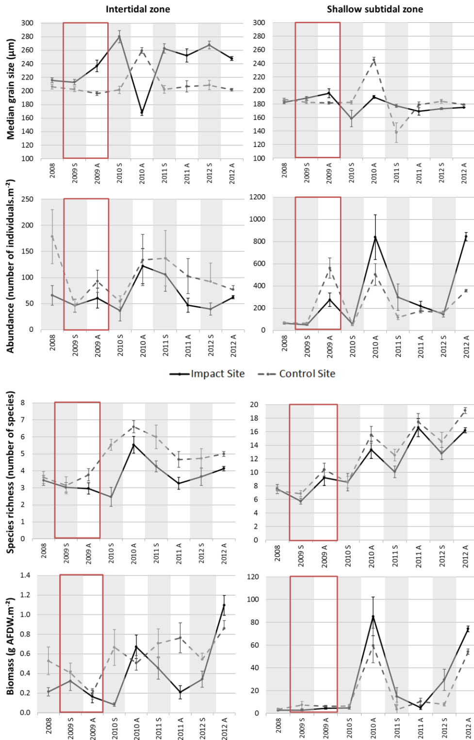
Figure 6: Mean median grain size ( \mu\text{m} ), species richness (number of species), abundance (number of individuals \cdot\text{m}^{-2} ) and biomass (g AFDW \cdot\text{m}^{-2} ) of the impact (black line) and control site (grey dotted line) per year with standard error, for the intertidal (left) and shallow subtidal zone (right) separately
