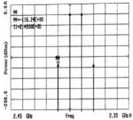
Fig. 2. Two-tone output spectrum without second harmonic injection.
