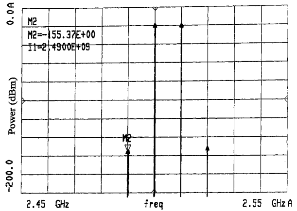
Fig. 8. Two-tone output spectrum with optimized difference-frequency injection.
