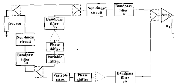
Fig. 1. Amplifier circuit with the injection of the second harmonic into the amplifier and predistortion circuit
