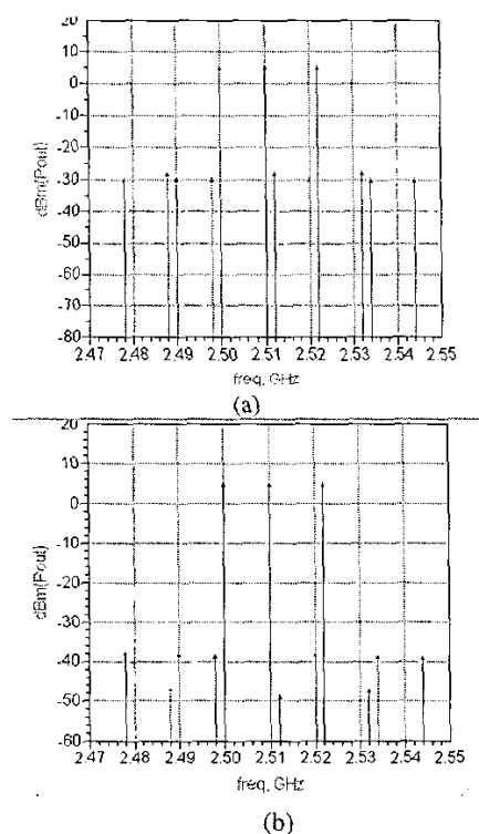
Fig. 5. The simulated output power of fundamental signals and IM3 products for three analog signals at input power 5 dB below 1-dB compression point: (a) without applying the linearization technique; (b) with applying linearization technique.
