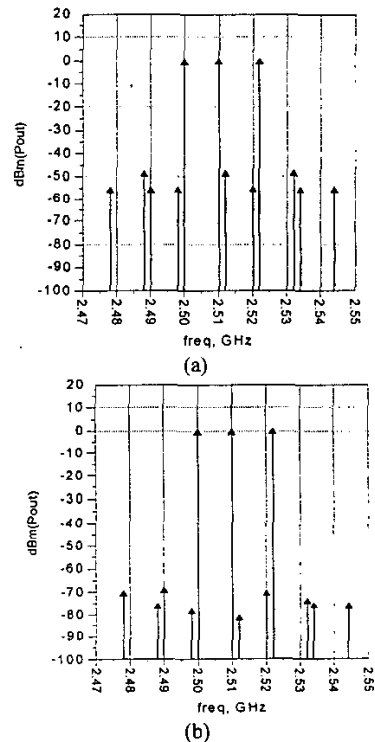
Fig. 4. Output spectrum: (a) without applying linearization technique; (b) after correction of -40^\circ deviation from optimal phase in the main injection path of IM2 signals
