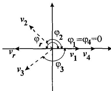
Fig. 3. Phasor diagram
