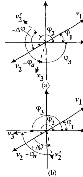
Fig. 2. Phasor diagram relates to: (a) minus; (b) plus deviation from optimal phase of the second harmonics
