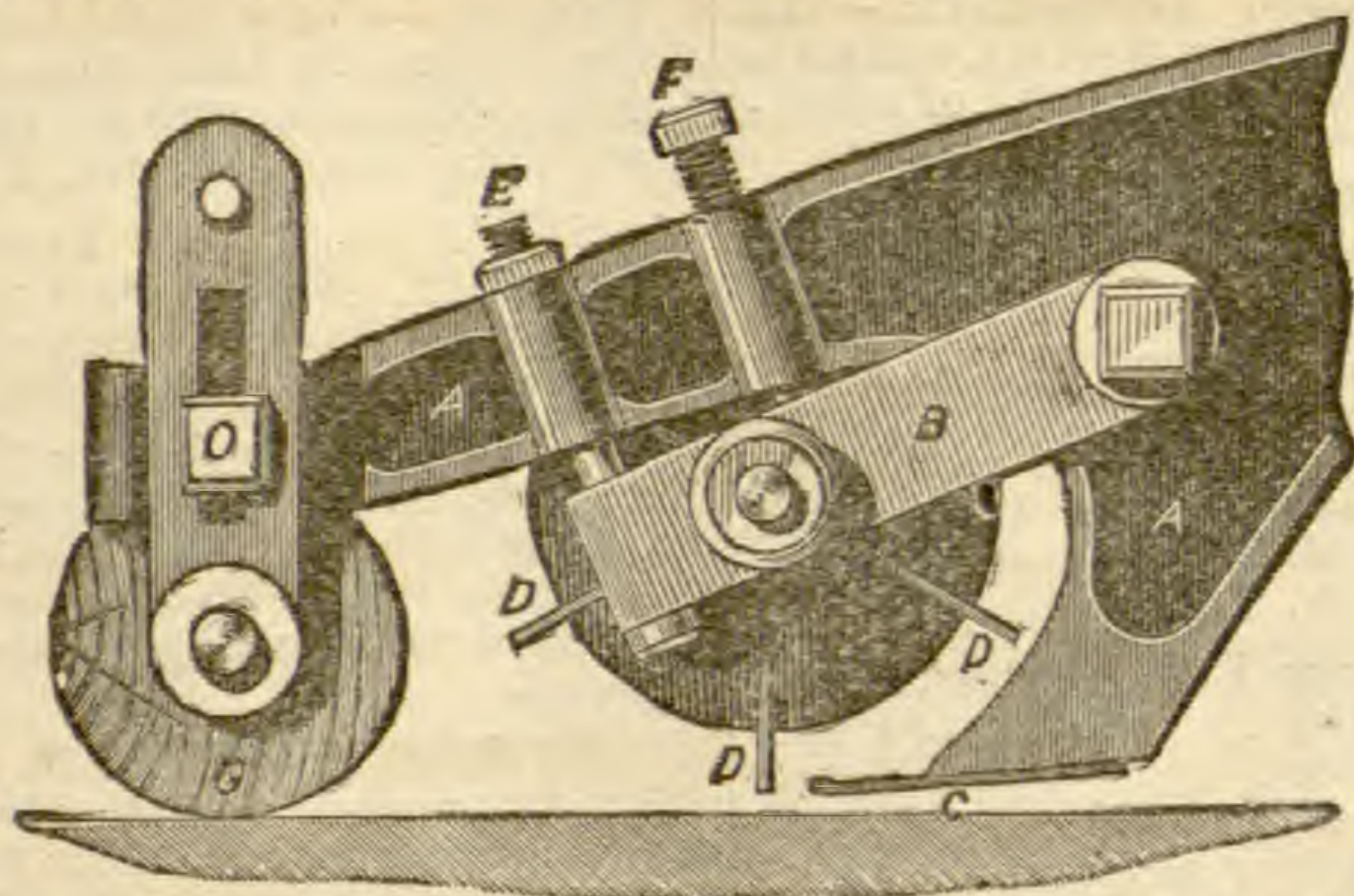
Showing mode of Adjusting the Cutters to the Ledger Blade, and regulating the cutting height from the ground.
