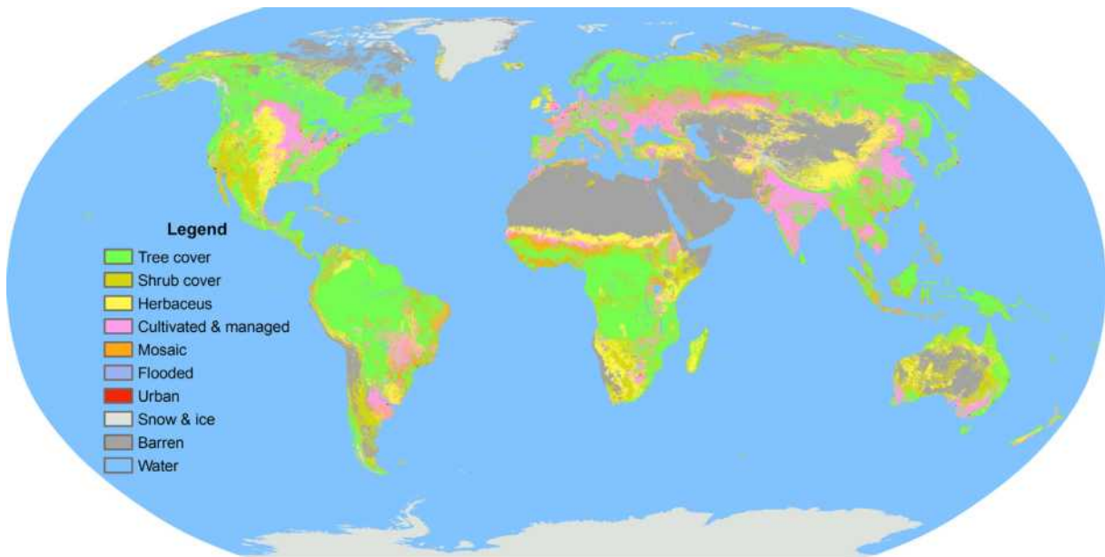
Fig. 6. The hybrid land cover map based on Geo-Wiki training points from the Hotspot Map Disagreement competition 2.
