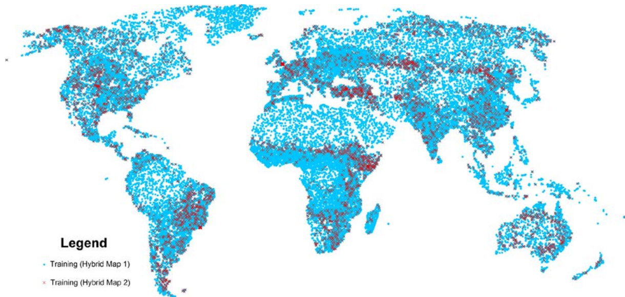
Fig. 2. Distribution of the training data for creation of the hybrid global land cover maps.
