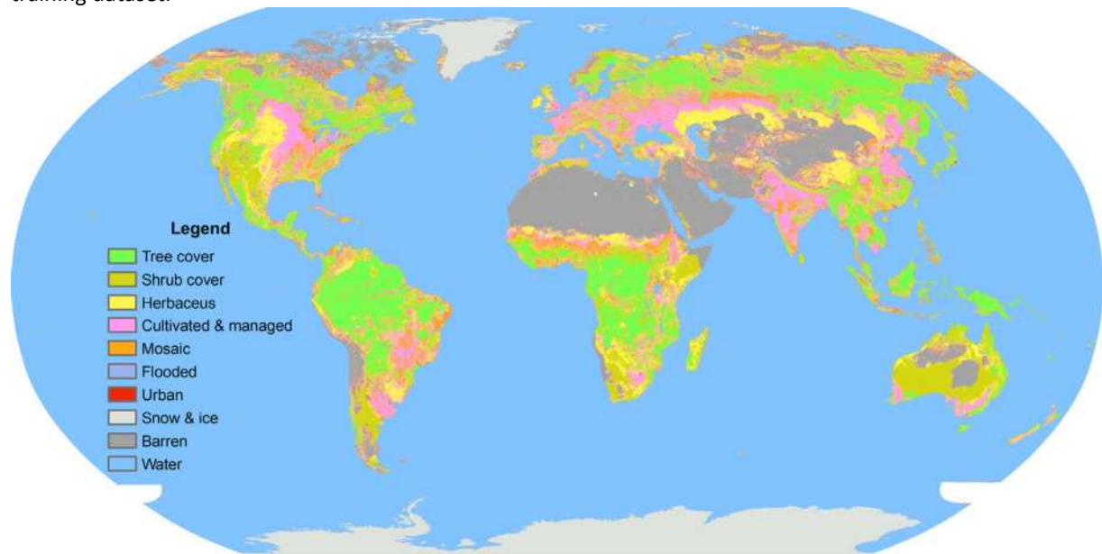
Fig. 5. The hybrid land cover map based on applying GWR trained with Geo-Wiki training data from Human Impact competition 1.
