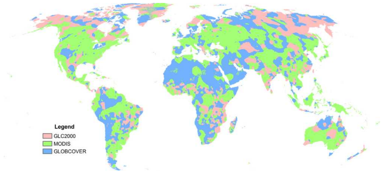
Fig. 4. Area when one or another land cover product shows the best agreement with the Geo-Wiki global training dataset.
