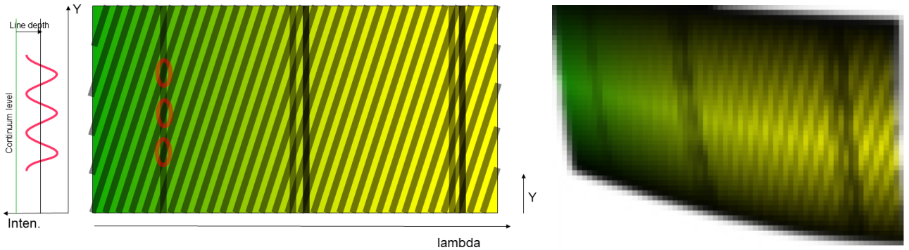
Figure 3. (left) Conceptual illustration of the spectrum of one star from MARVELS dispersed fixed-delay interferometry. The diagonal pattern of constructive and destructive interference is not sharp as in this simple diagram, but rather varies sinusoidally with y . The phase of the best-fitting sinusoid to each column of the data determines the corresponding wavelength shift, given the slope of the interference comb. (right) Illustration of some of the real-world effects of variable projection of spectra onto the focal plane, spectrograph alignment, point spread function, and the variable slope of the interference comb. There are 120 of these spectra (each roughly 4096 pixels by 34 pixels) per MARVELS exposure.
