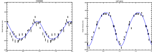
Figure 5. MARVELS observations of the radial velocities of the stars (left) HD68988 compared to the model of Butler et al. (2006); and (right) HIP-14810 compared to the model of Wright et al. (2009).
