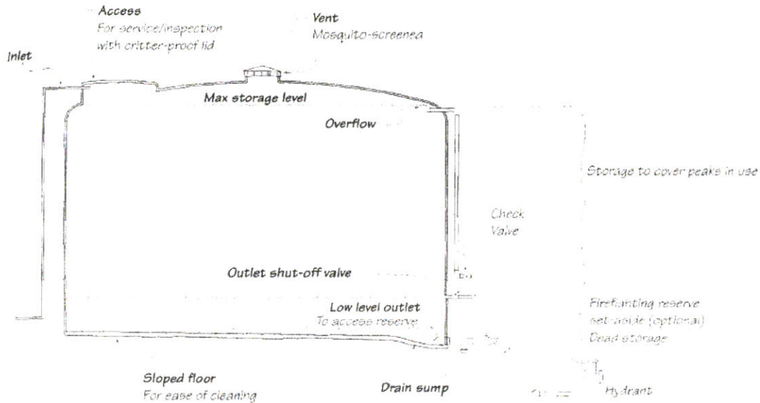
Figure 4: Common Tank Features (Ludwig 2005)
