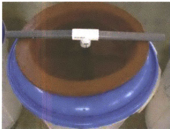
Figure 62: T-device in filter element for flow test
