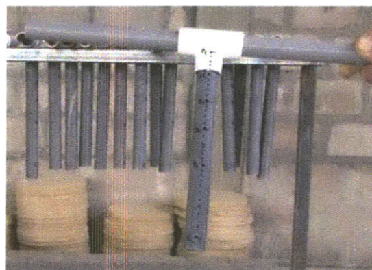
Figure 59: T-device close-up (Bradner 2011)
