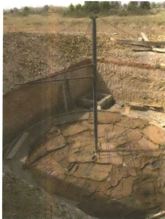
Figure 46: Finished foundation is covered with wet burlap sacks to keep it moist while concrete dries
