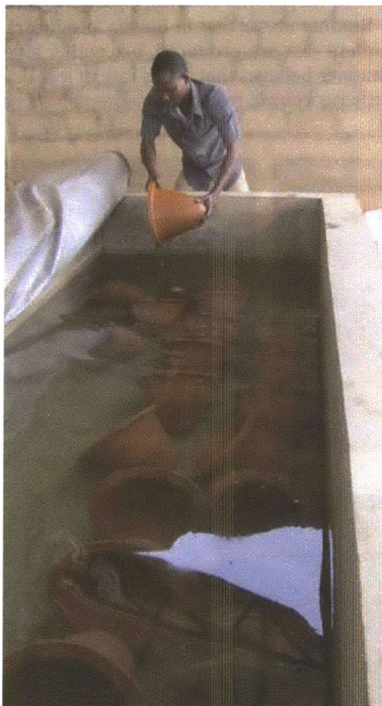
Figure 77: Karim bubble tests filters
