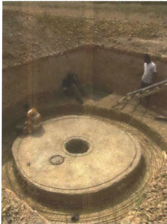
Figure 26: The steel bender begins radial reinforcement
