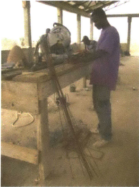
Figure 20: The steel bender bending 1/2 inch rebar
